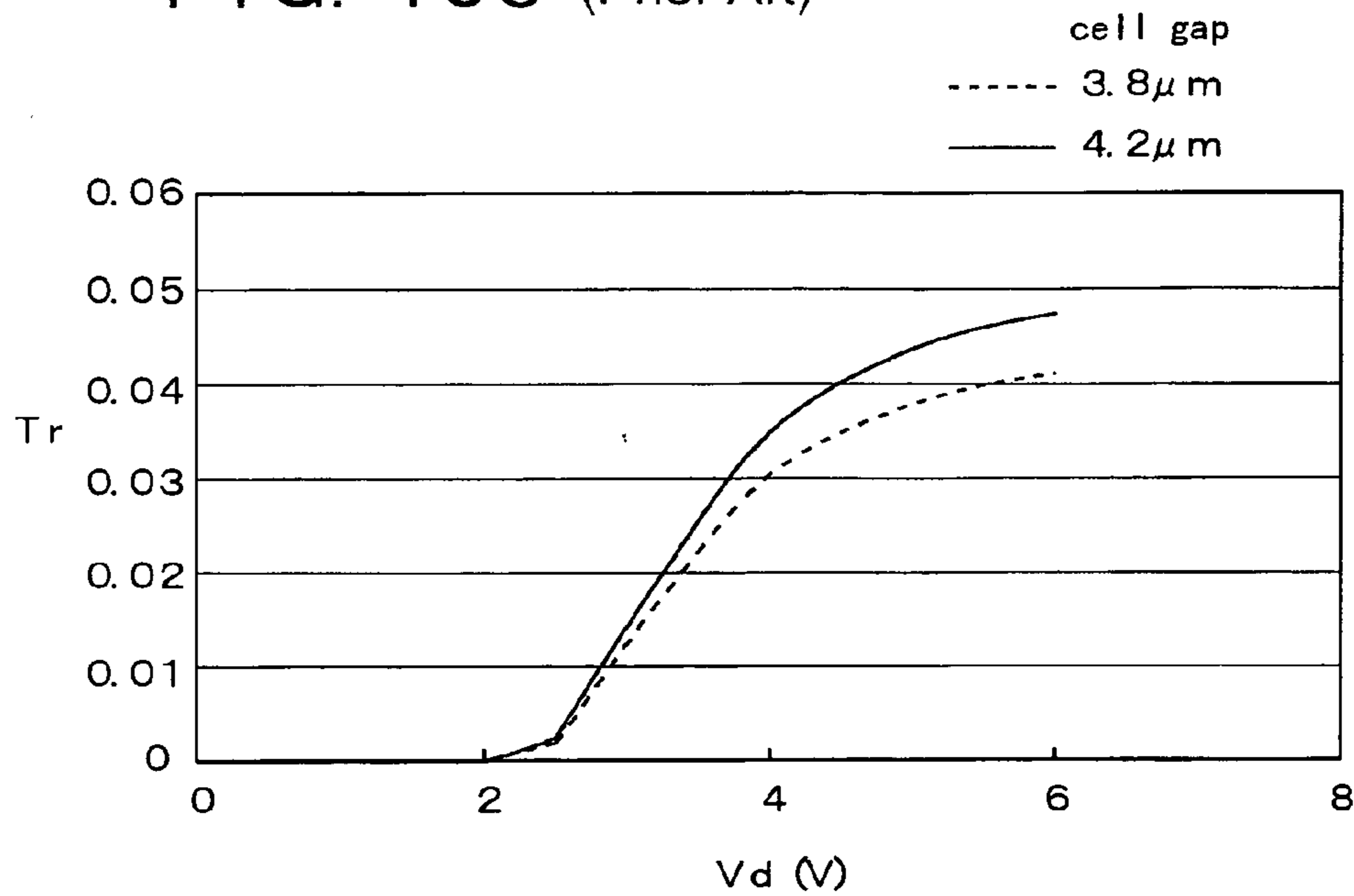
FIG. 103 (Prior Art)
