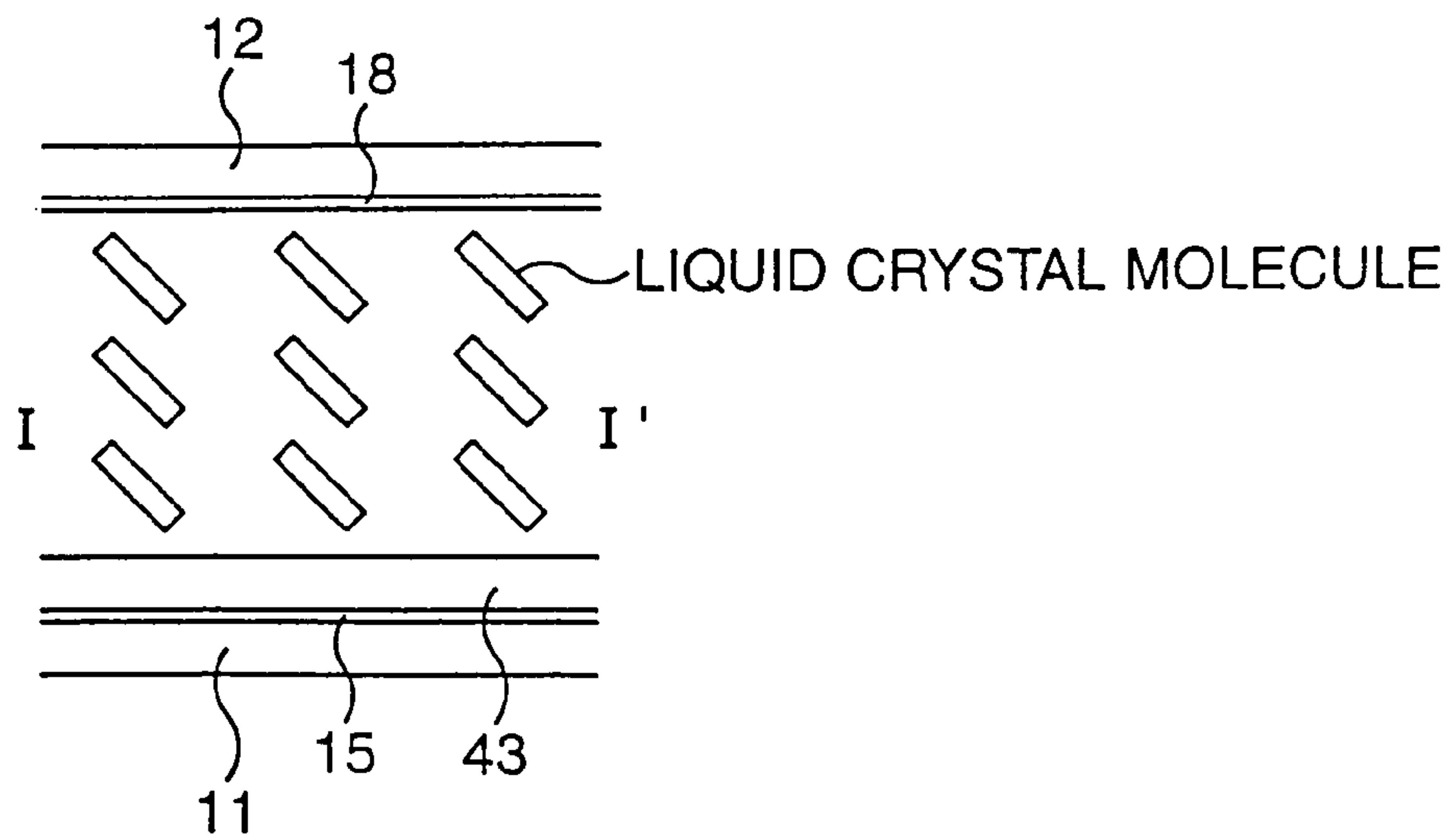
SECTIONAL VIEW
