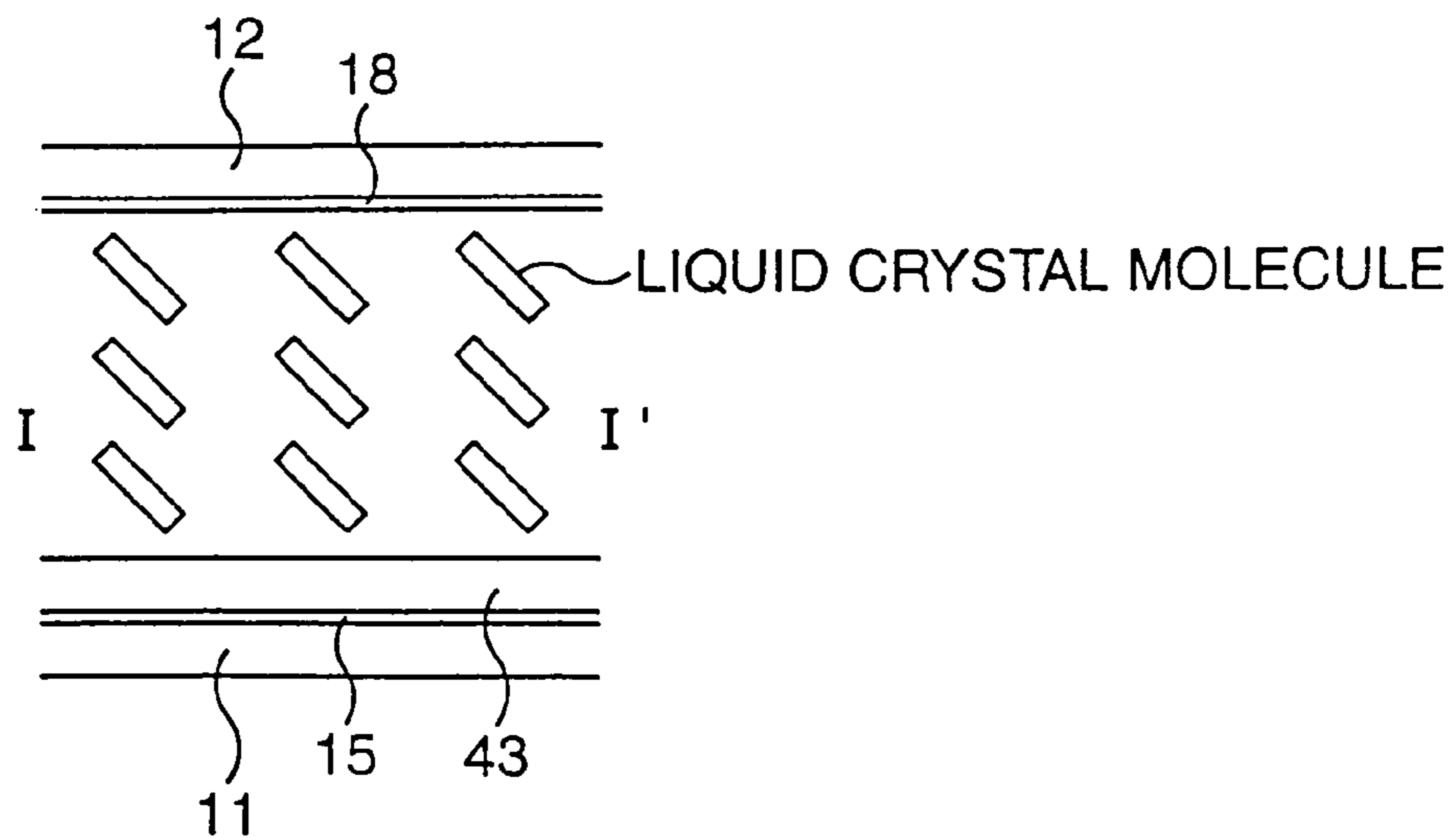
SECTIONAL VIEW
