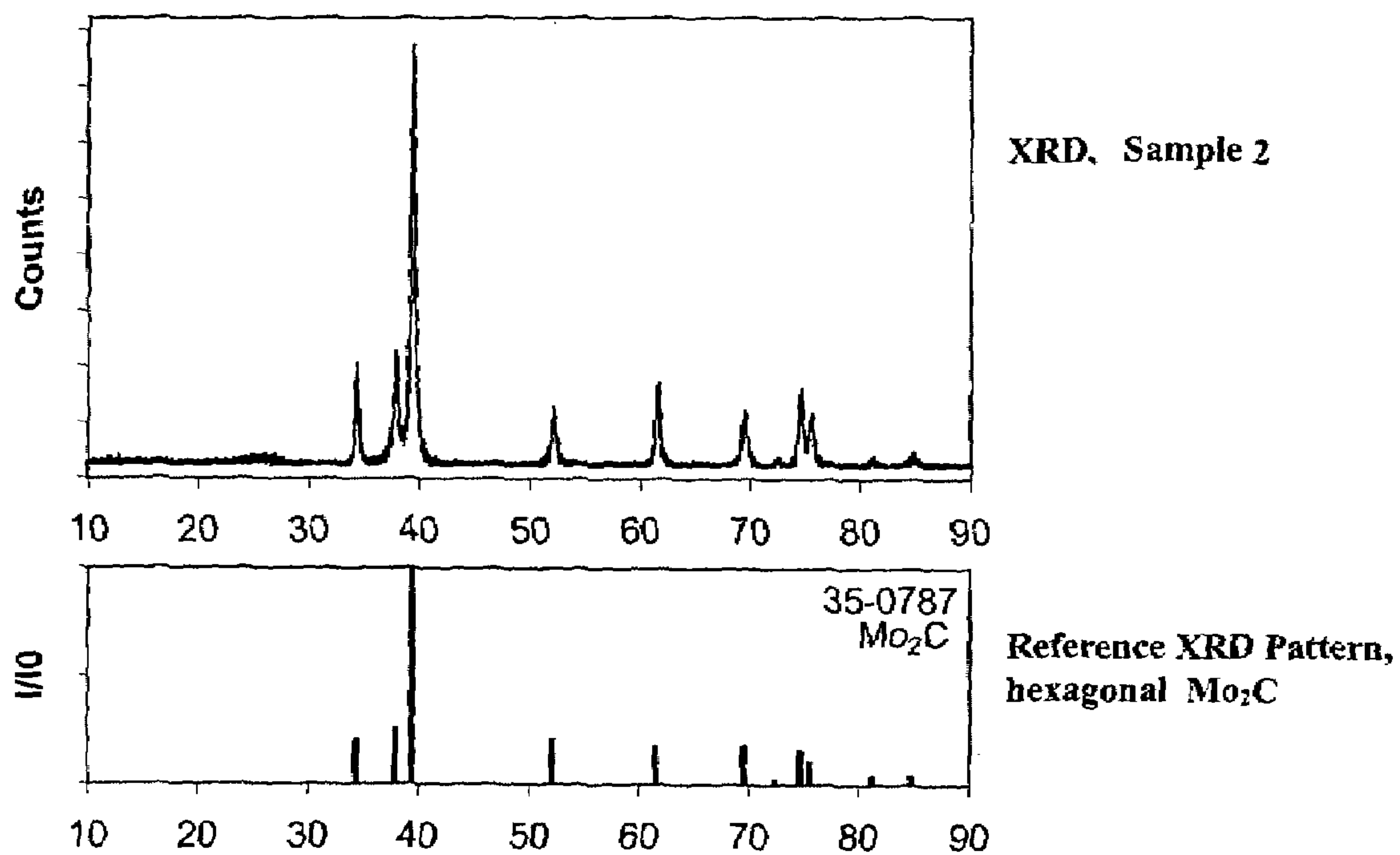
FIG. 2A XRD and HRTEM of CARBIDE NANORODS
