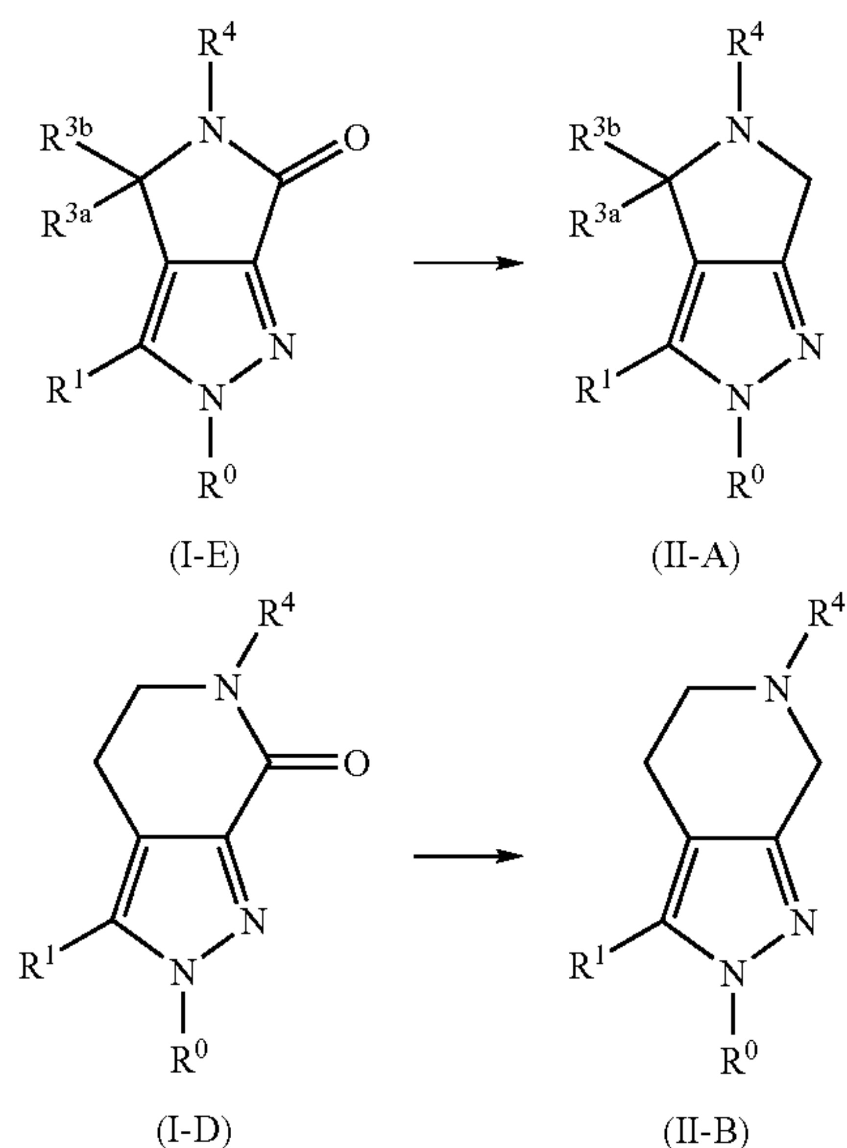
Scheme VIII
