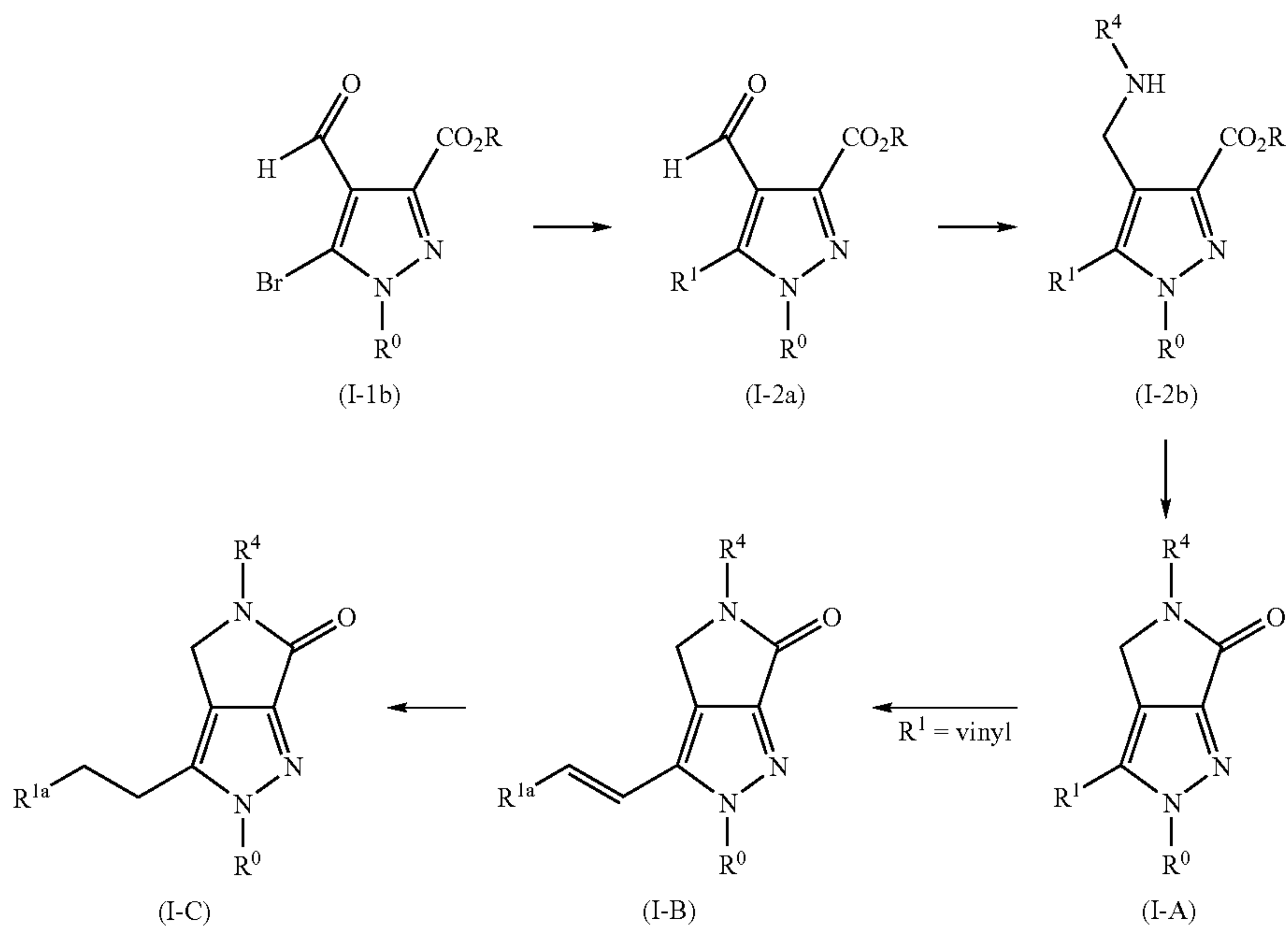
Scheme II
