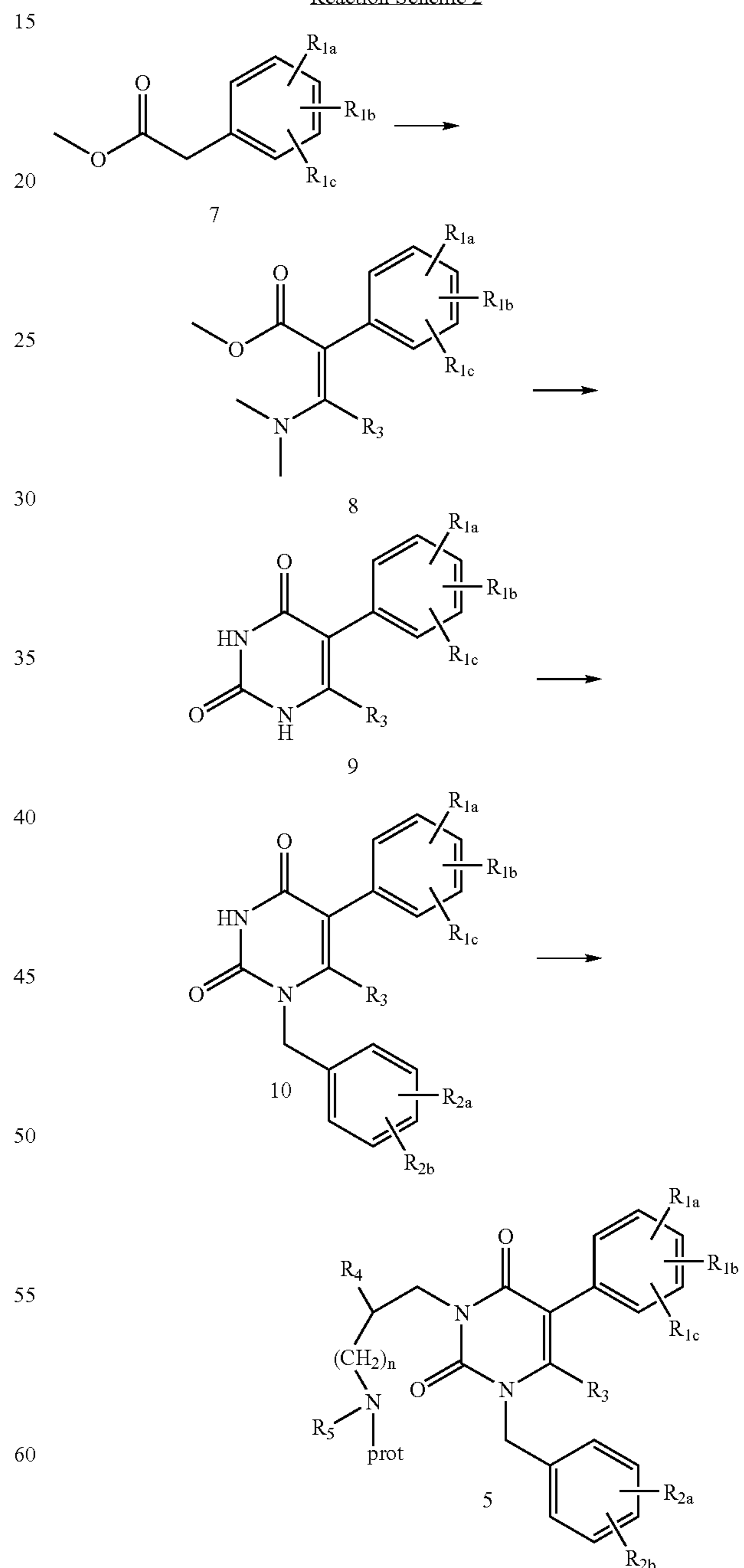
Reaction Scheme 2
