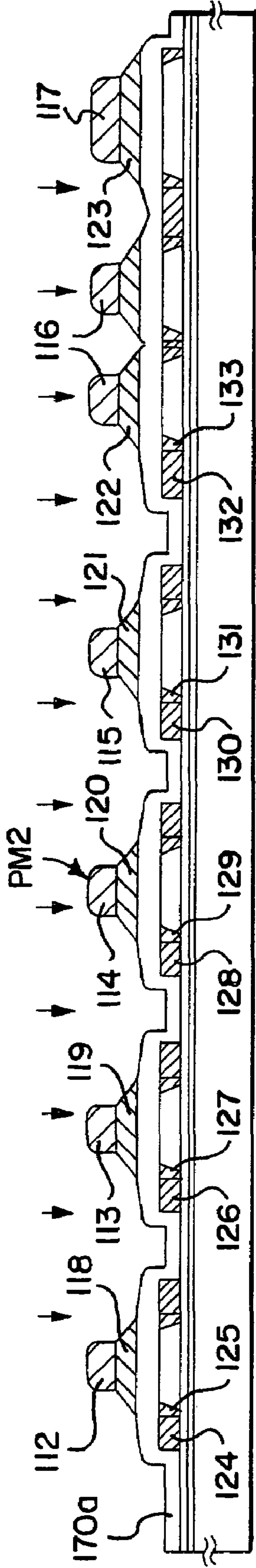
FIG. 7A FIRST ETCHING PROCESS/FIRST DOPING PROCESS (n + )
