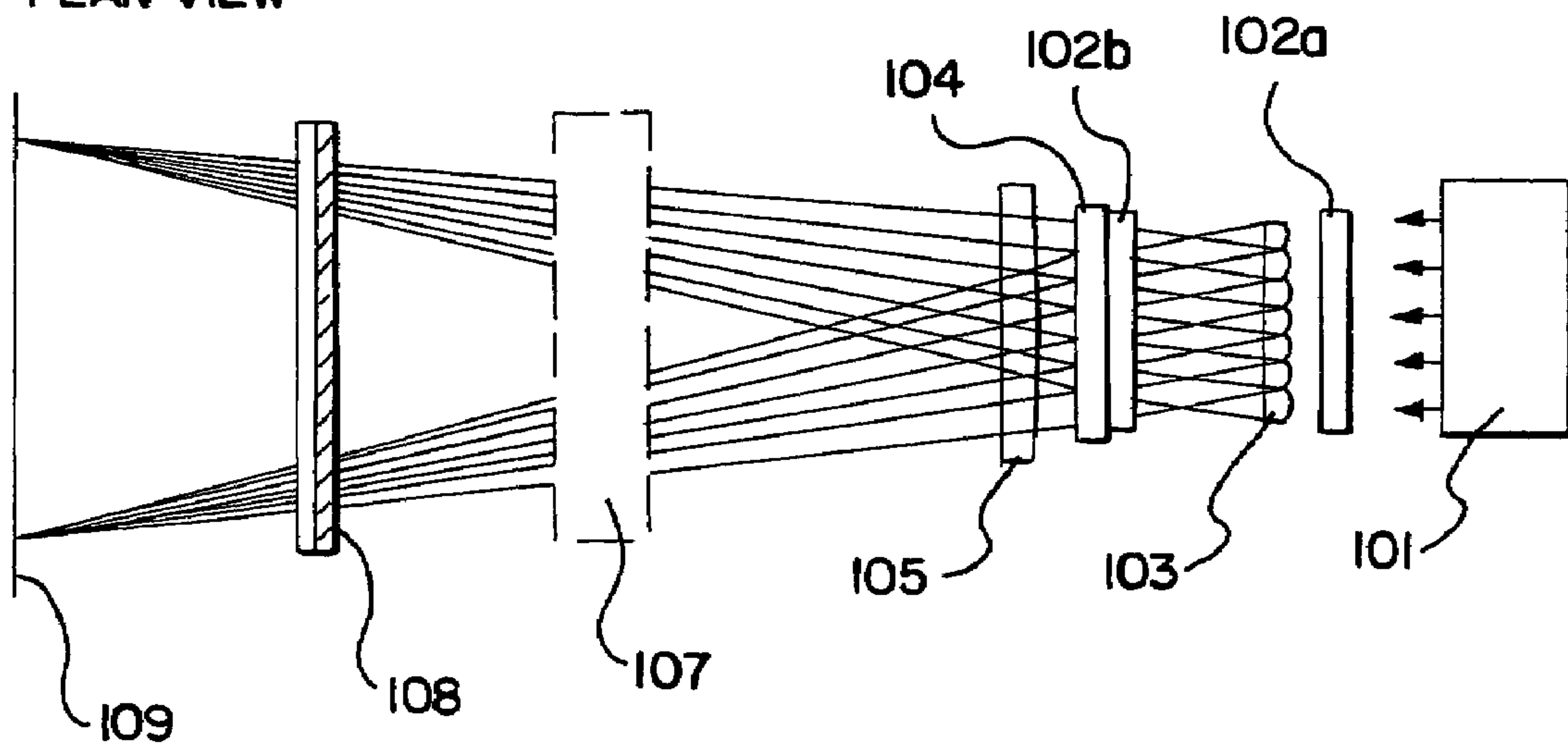
FIG. 1B PLAN VIEW
