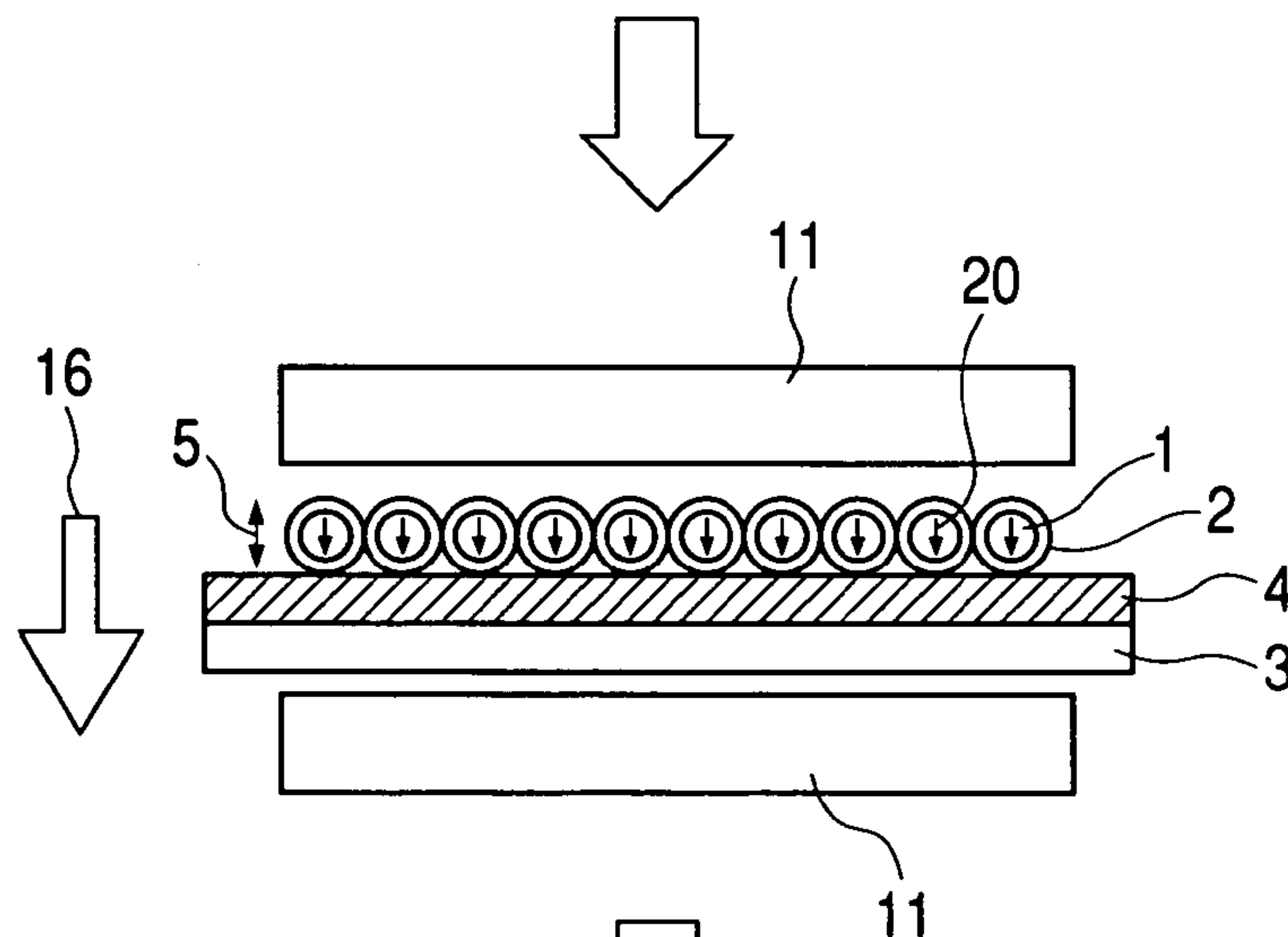
FIG. 7C SIDE VIEW
