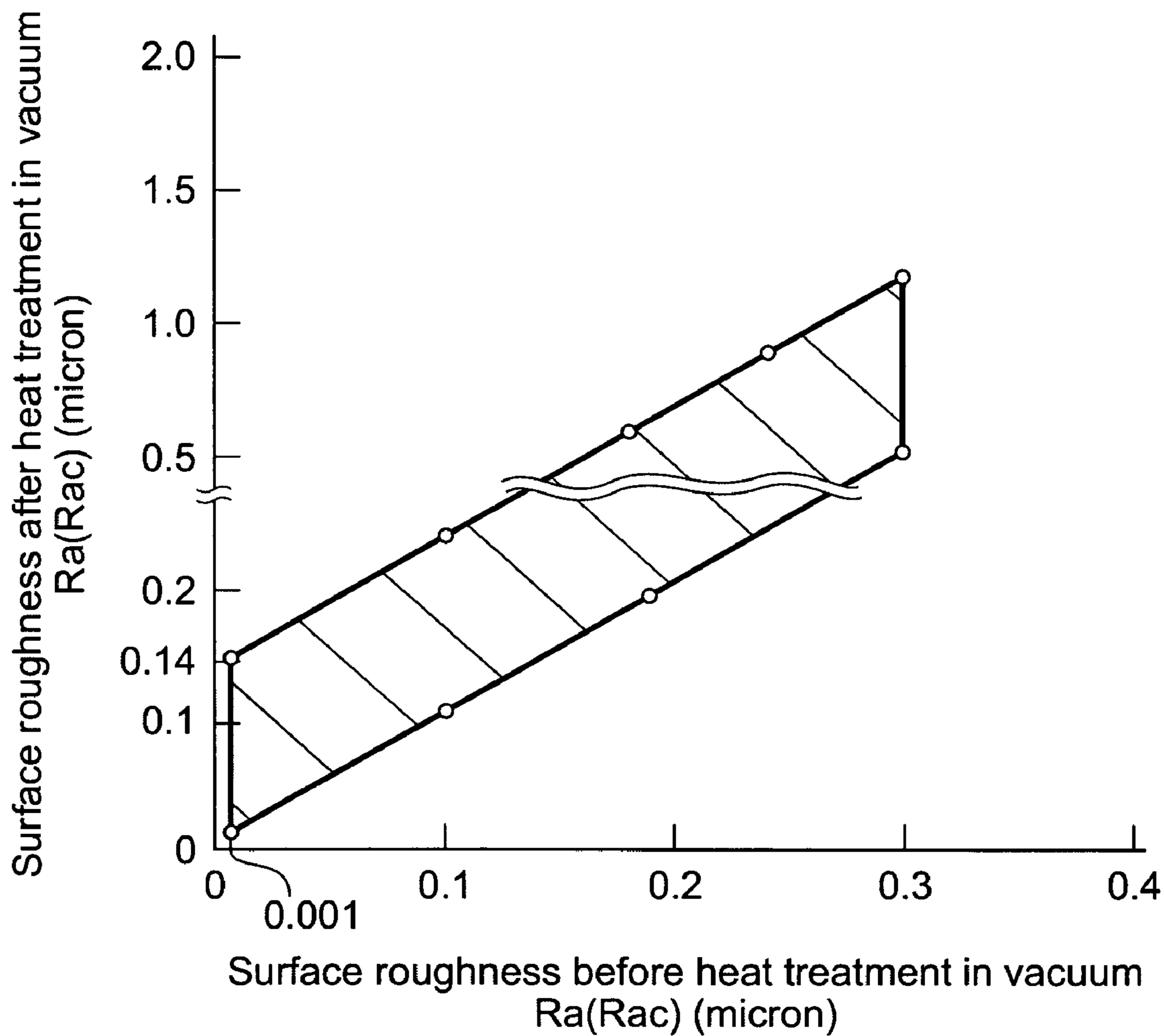
Change In Surface Roughness Before And After Heat Treatment In Vacuum
