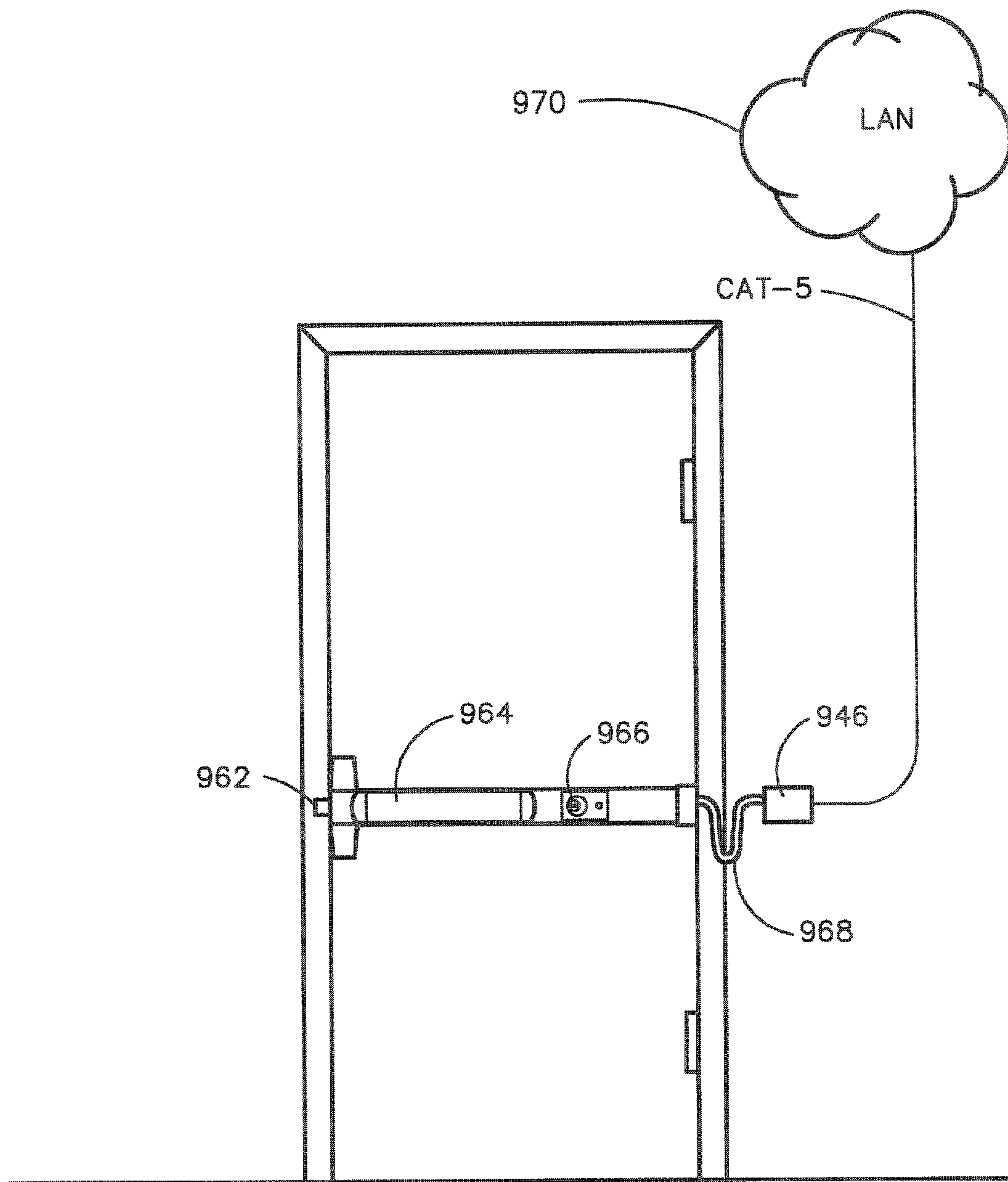
WIRED EXIT DEVICE
