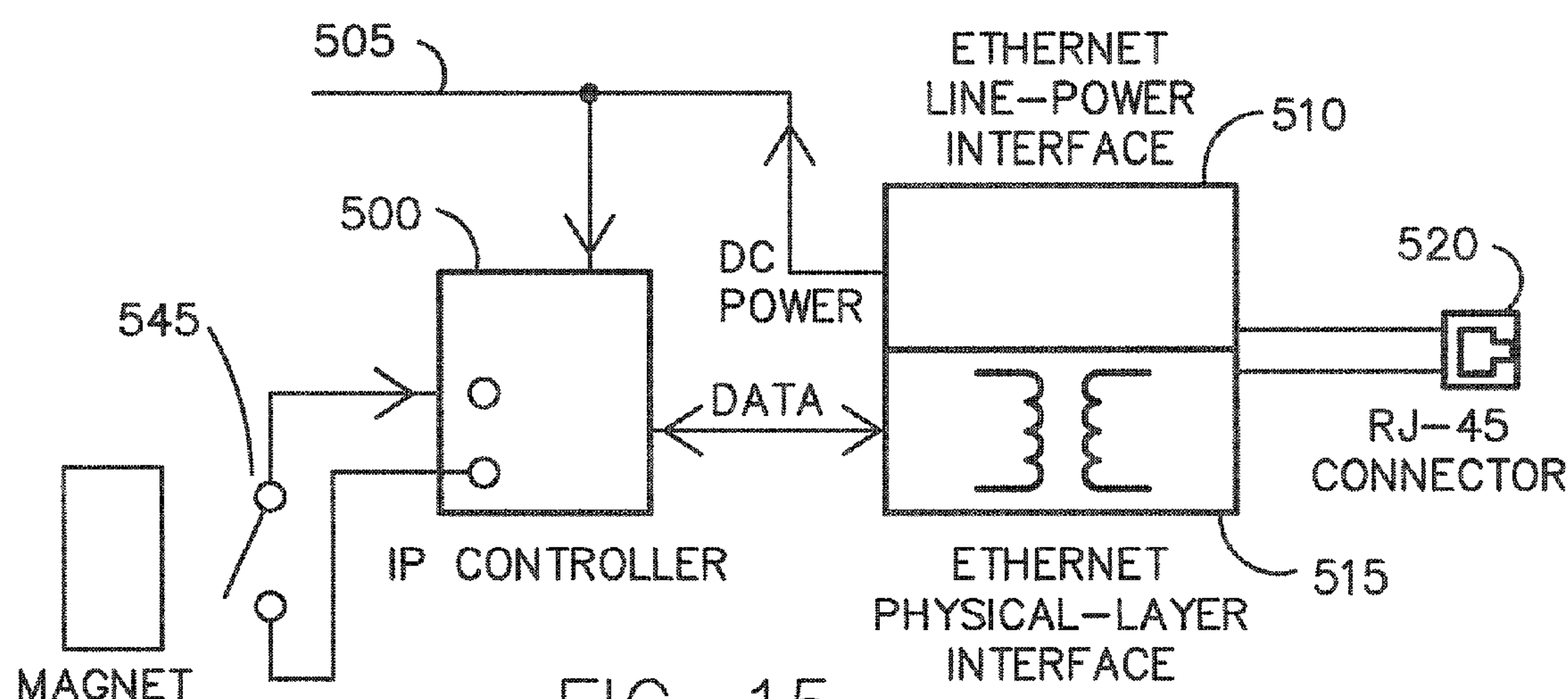
INTERNAL CONTACT INTERFACE
