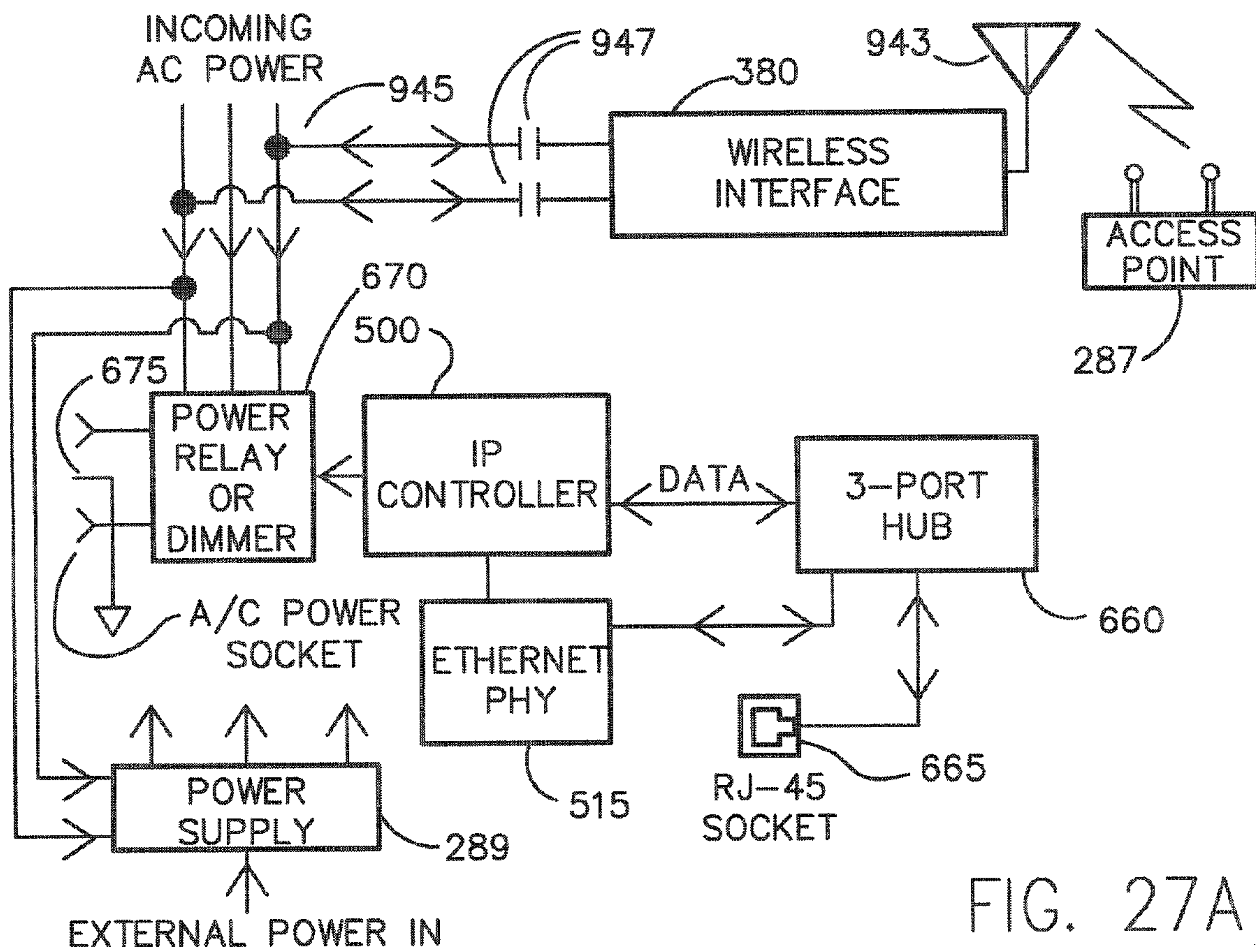
POWER CONTROL (SWITCH OR DIMMER)
