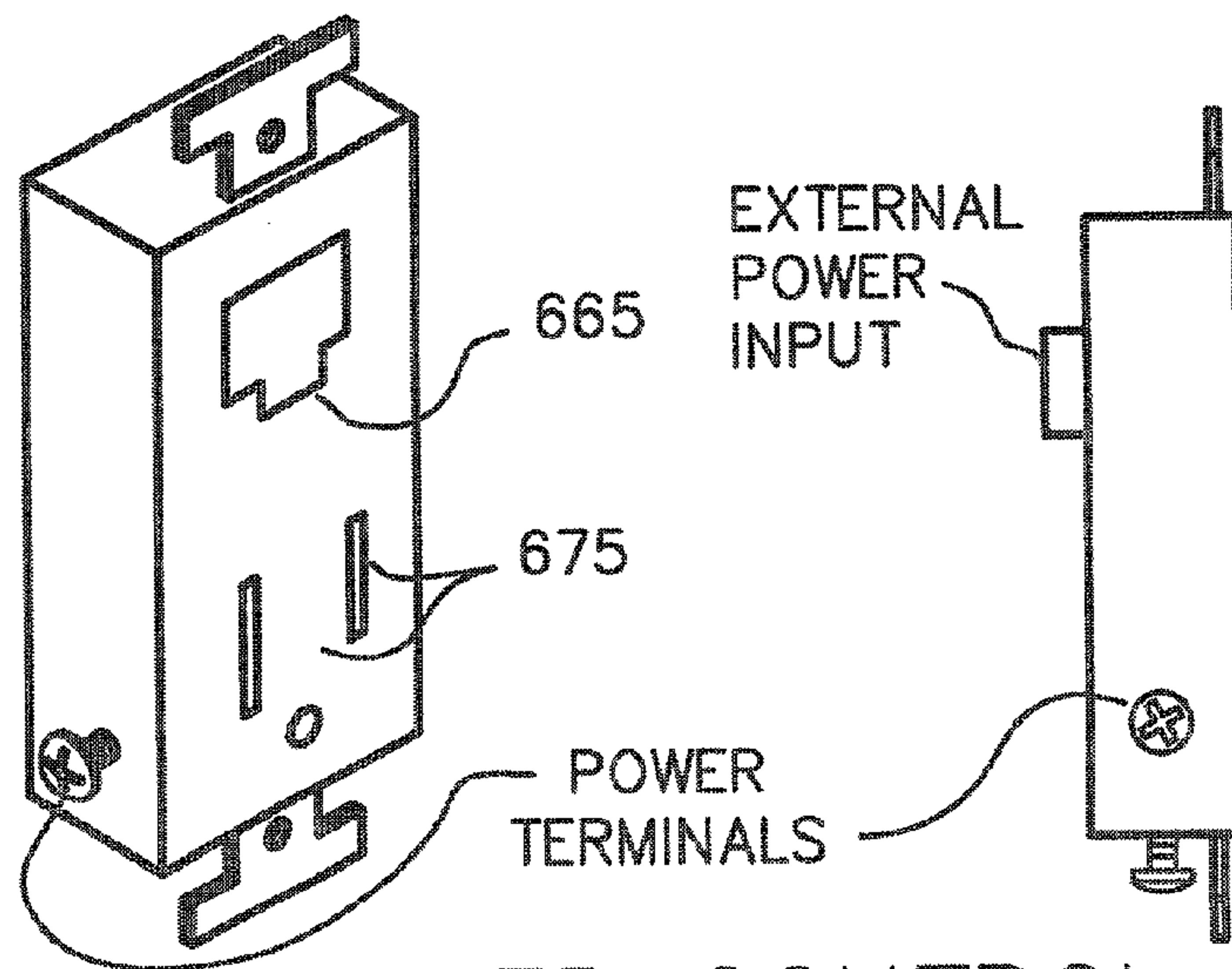
POWER CONTROL (SWITCH OR DIMMER)
