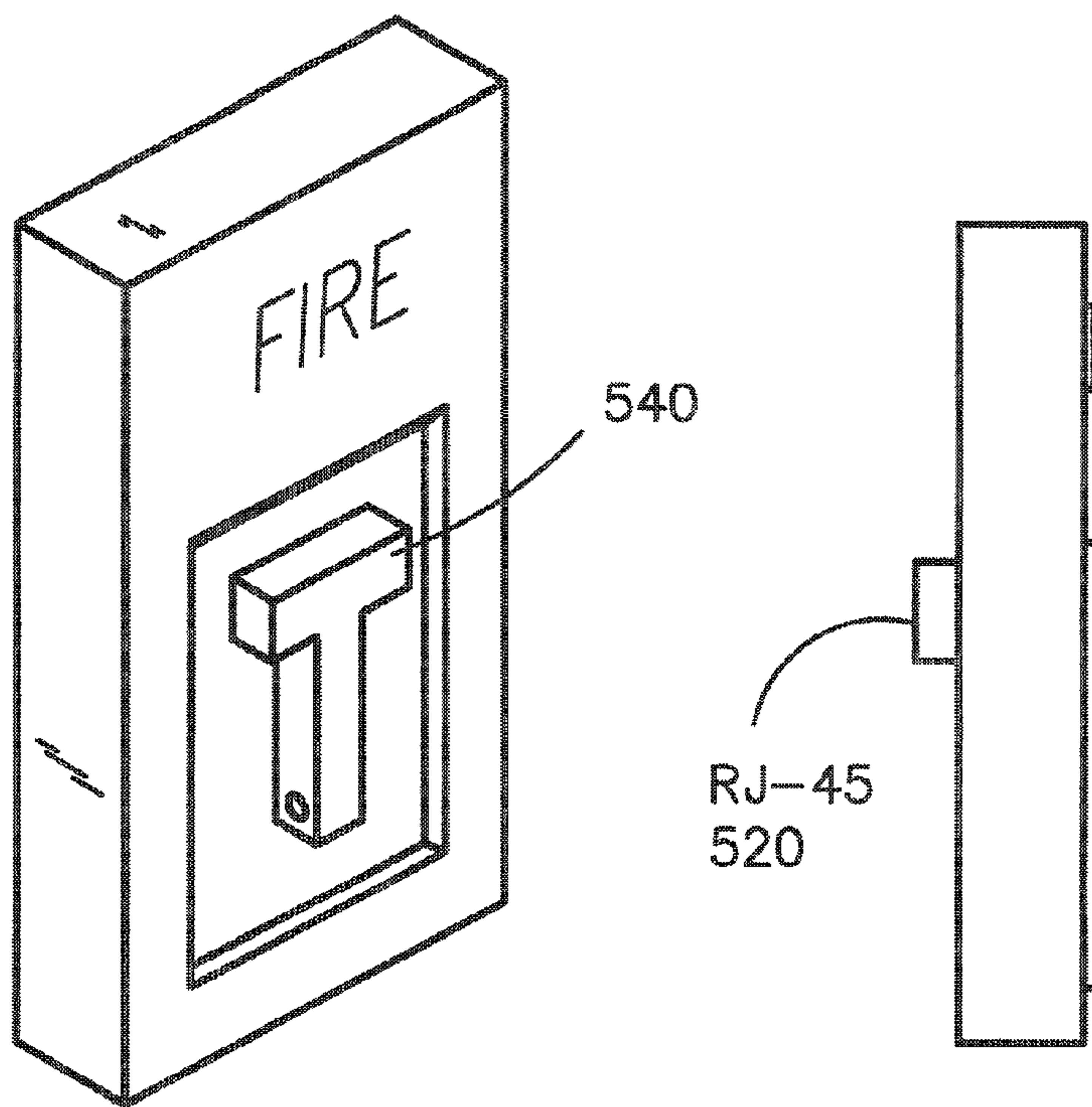
PULL HANDLE
