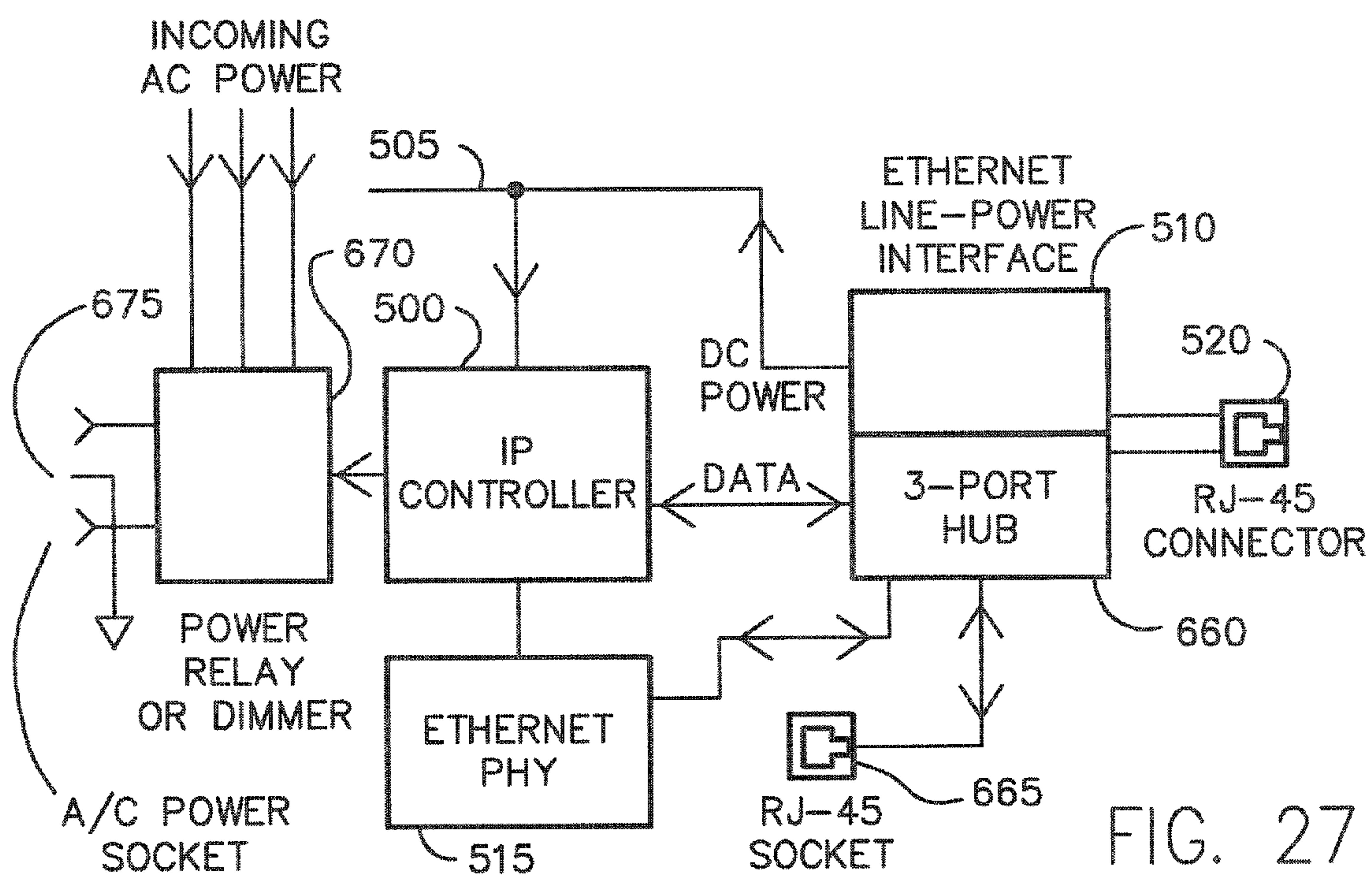
POWER CONTROL (SWITCH OR DIMMER)
