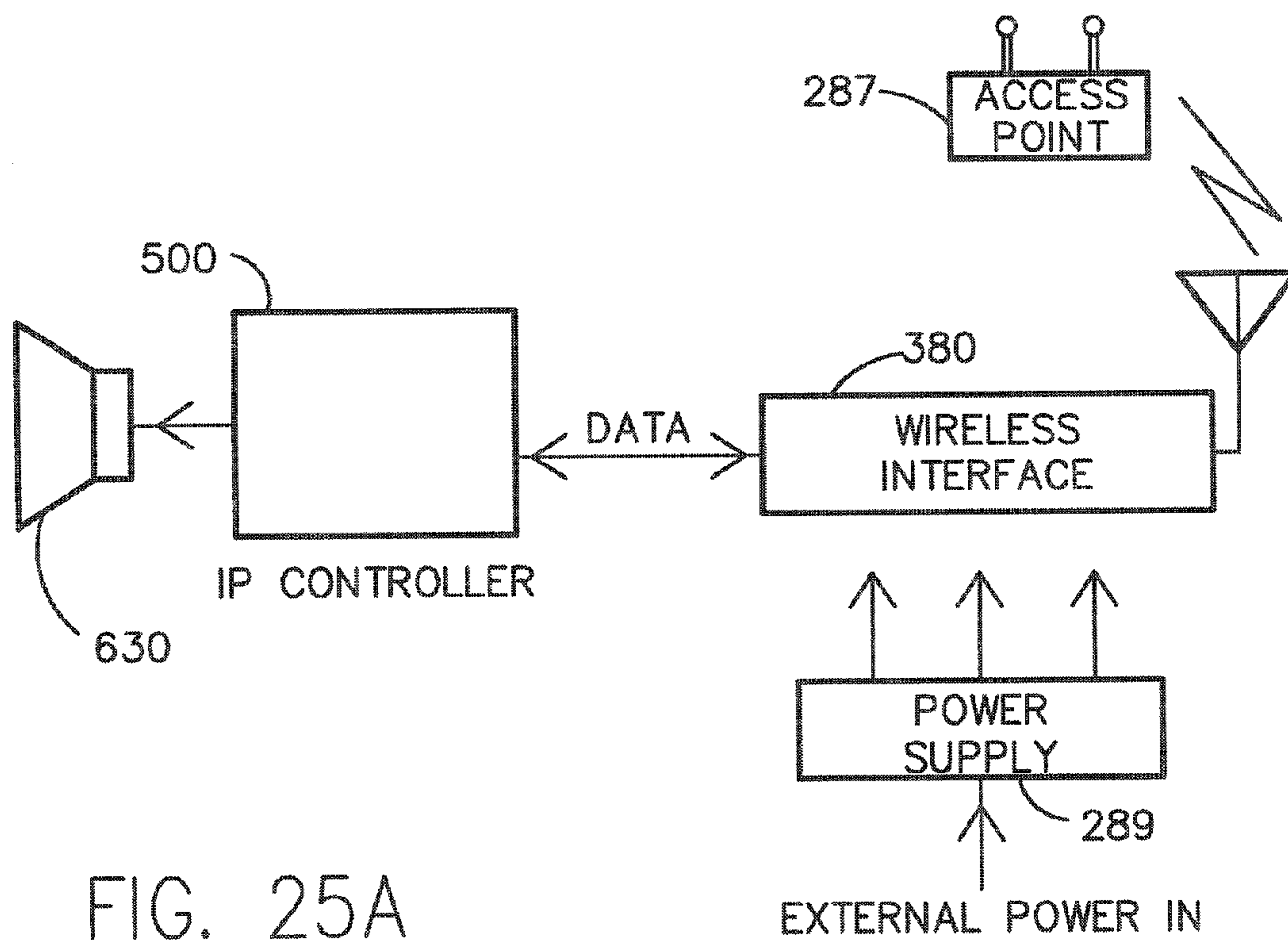
LOUDSPEAKER WITH AMPLIFIER
