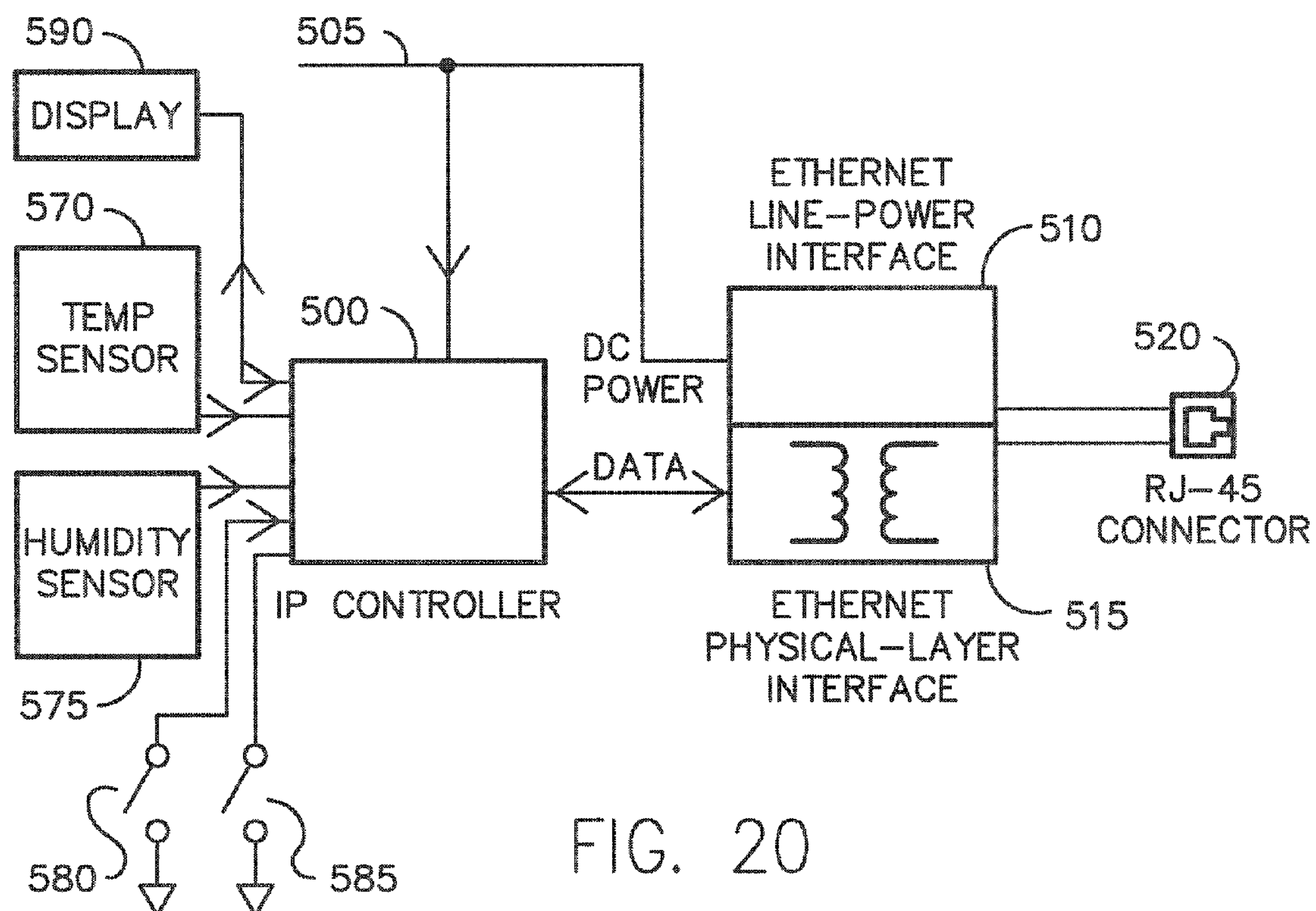
THERMOSTAT AND/OR HUMIDISTAT
