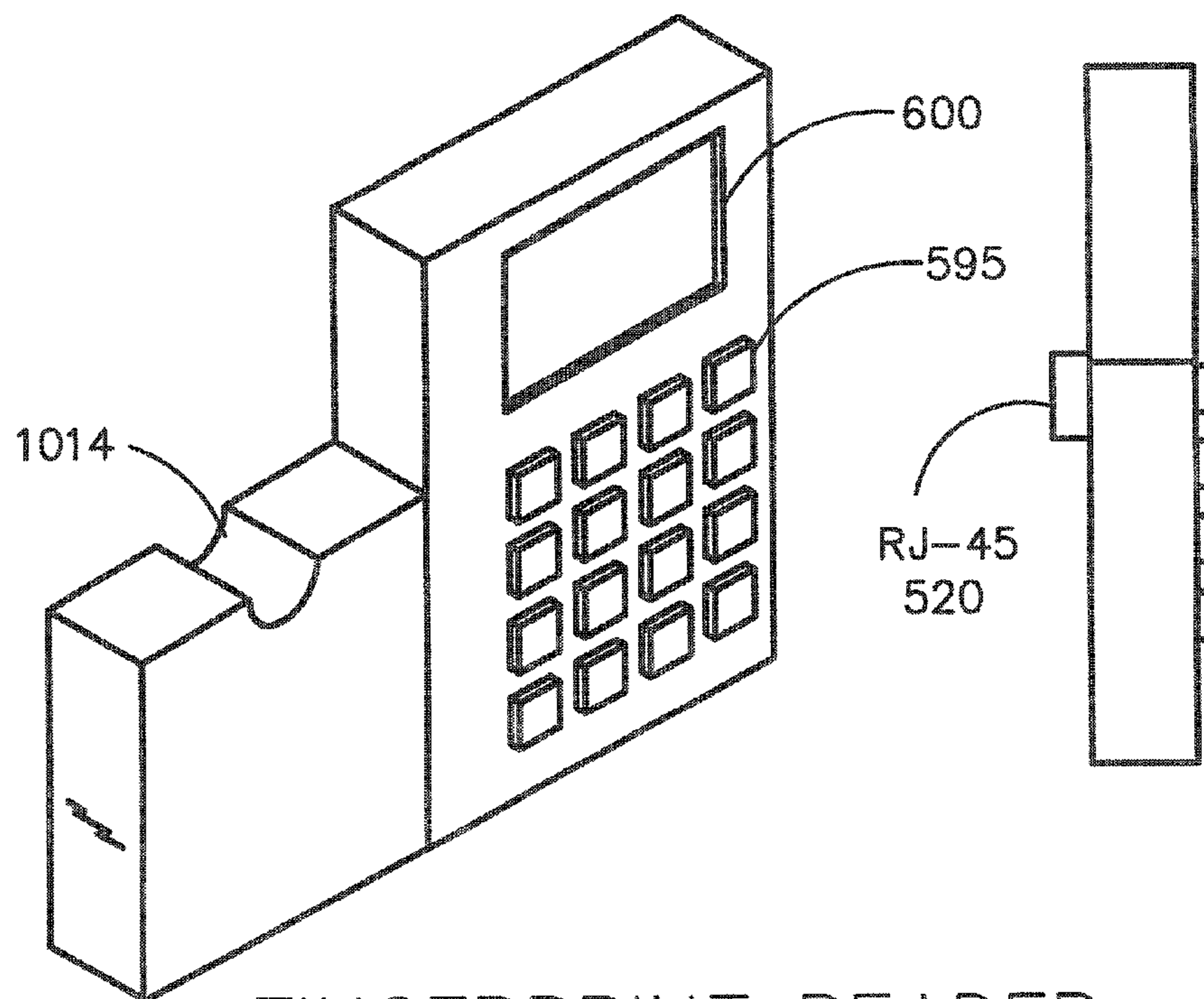
FINGERPRINT READER
