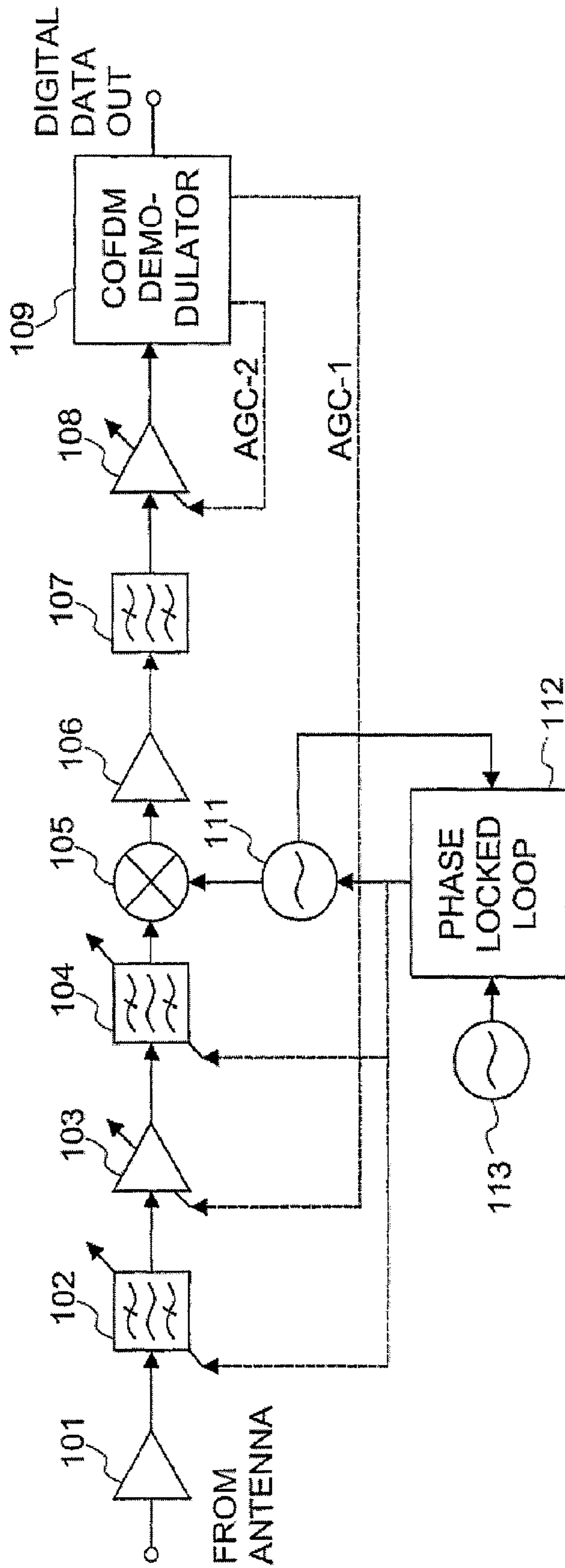
Fig. 1 (PRIOR ART)
