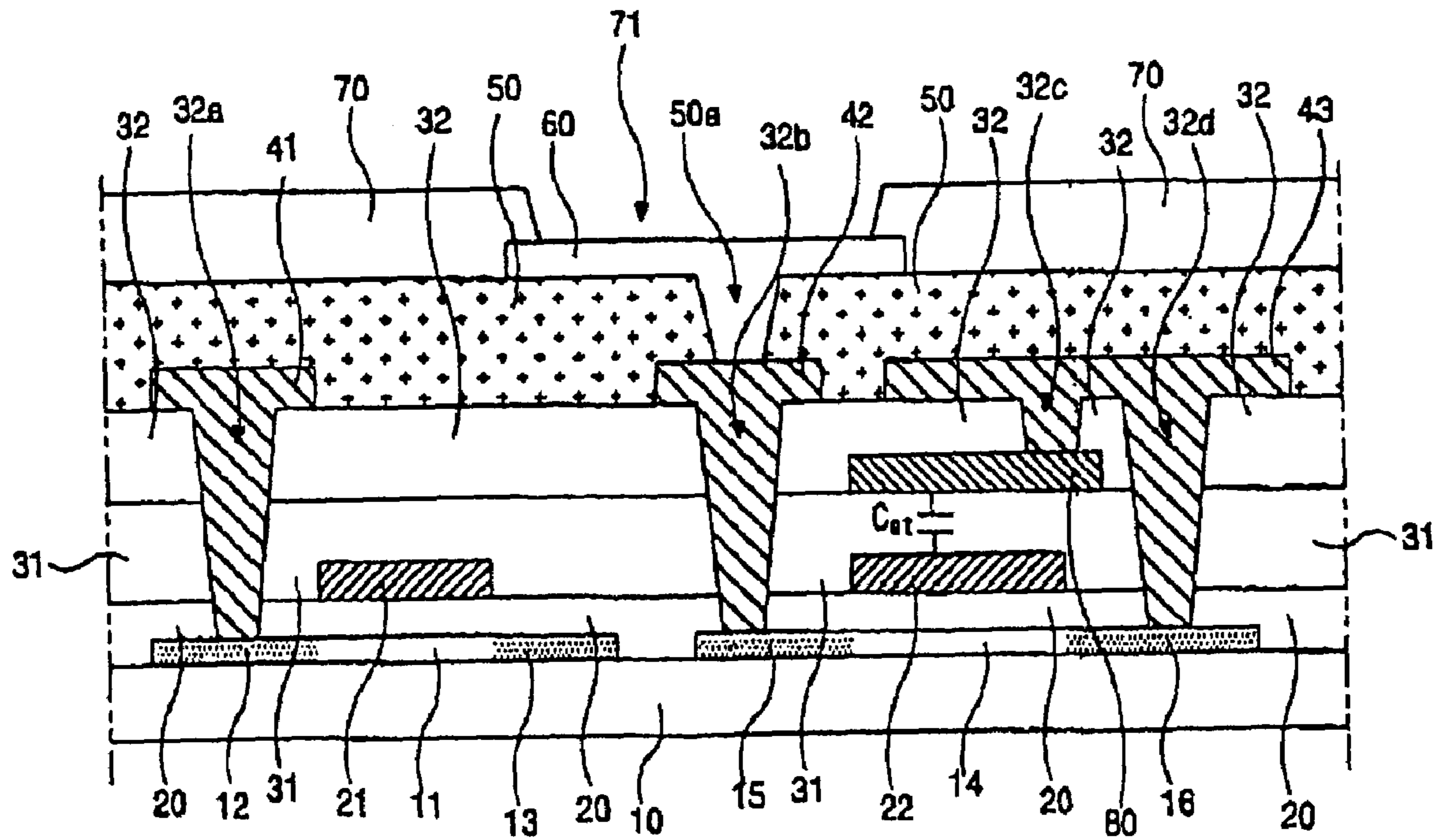
FIG. 4 (RELATED ART)
