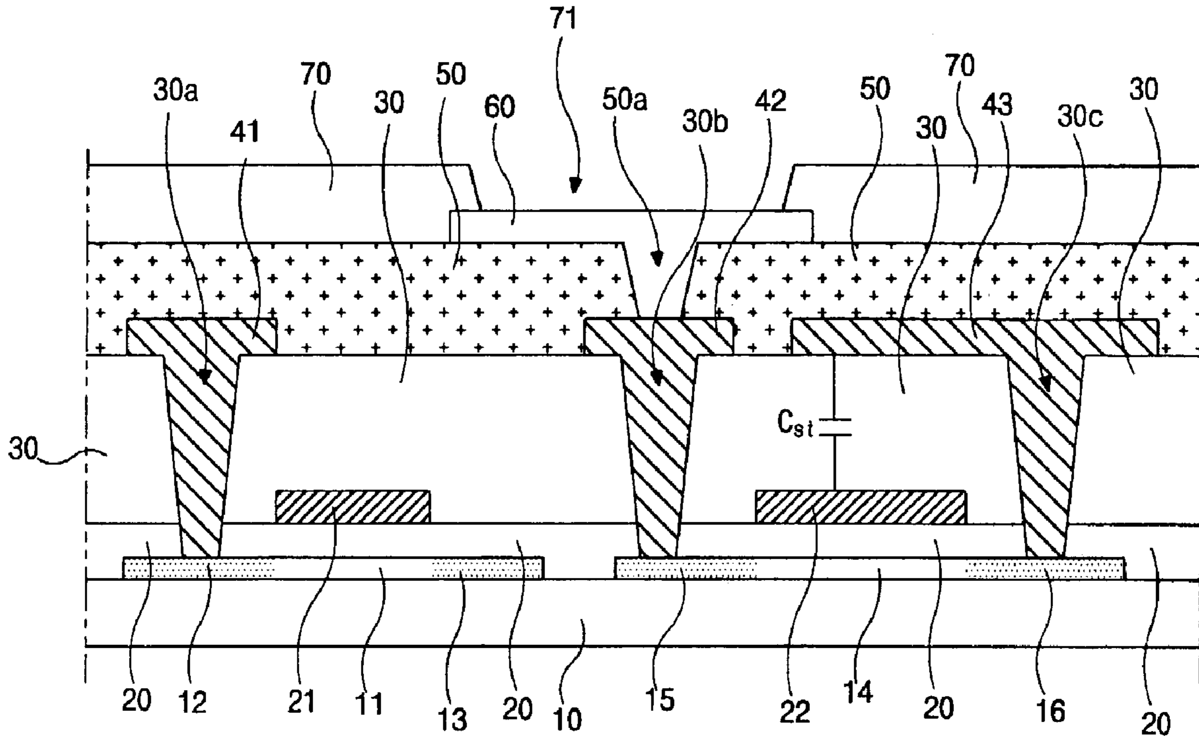
FIG. 2 (RELATED ART)
