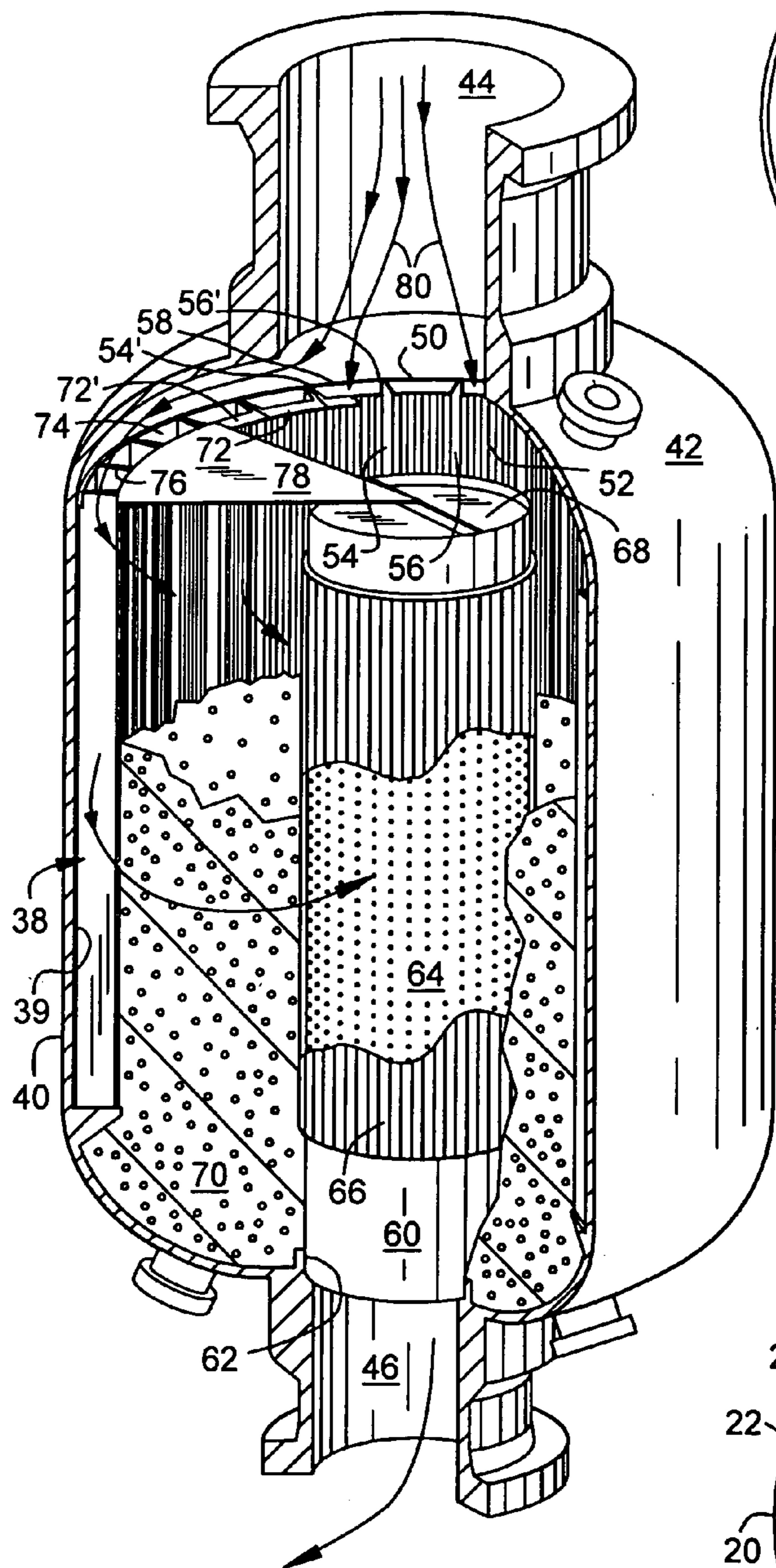
FIG. 2 (PRIOR ART)
