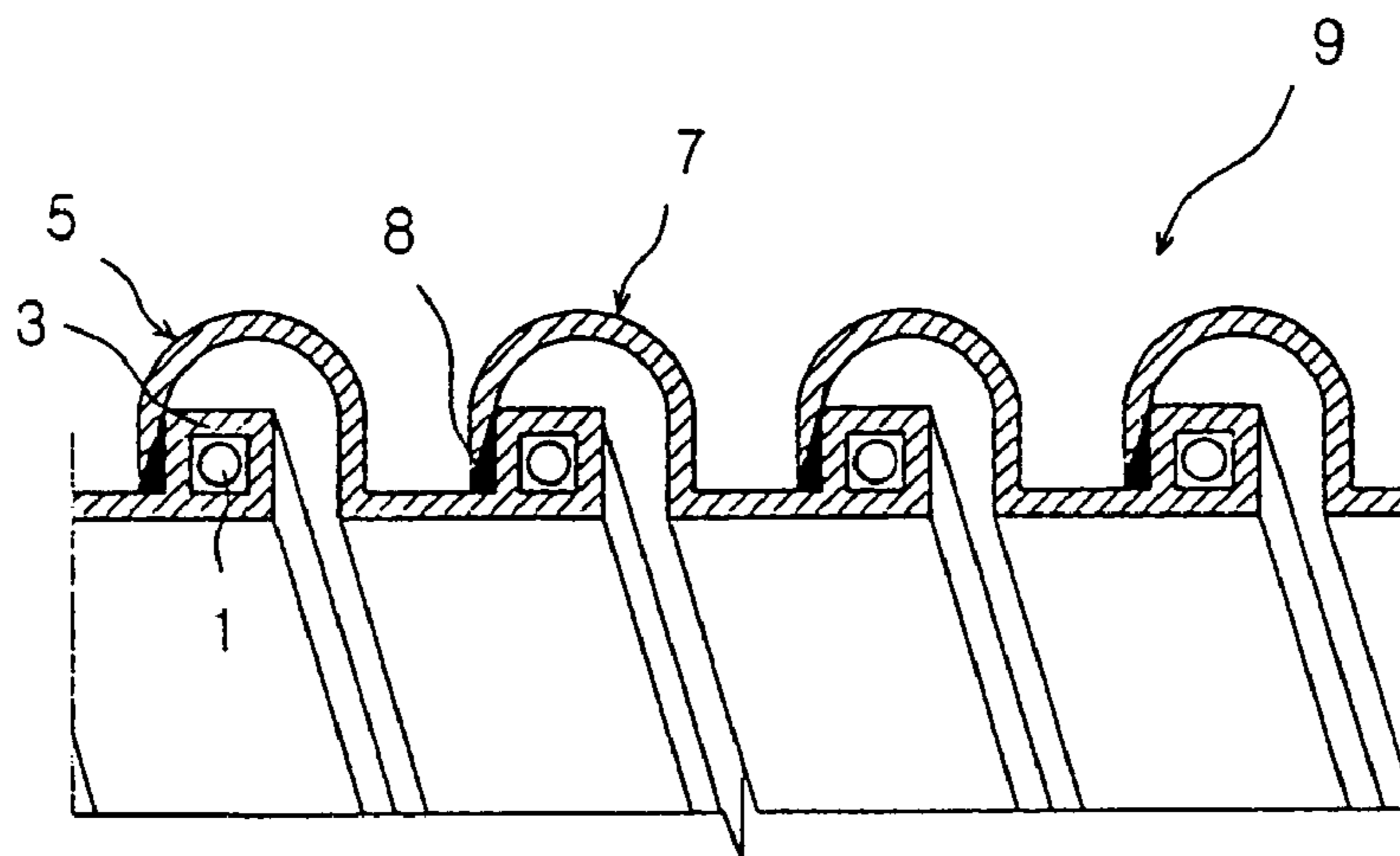
FIG. 9 (PRIOR ART)
