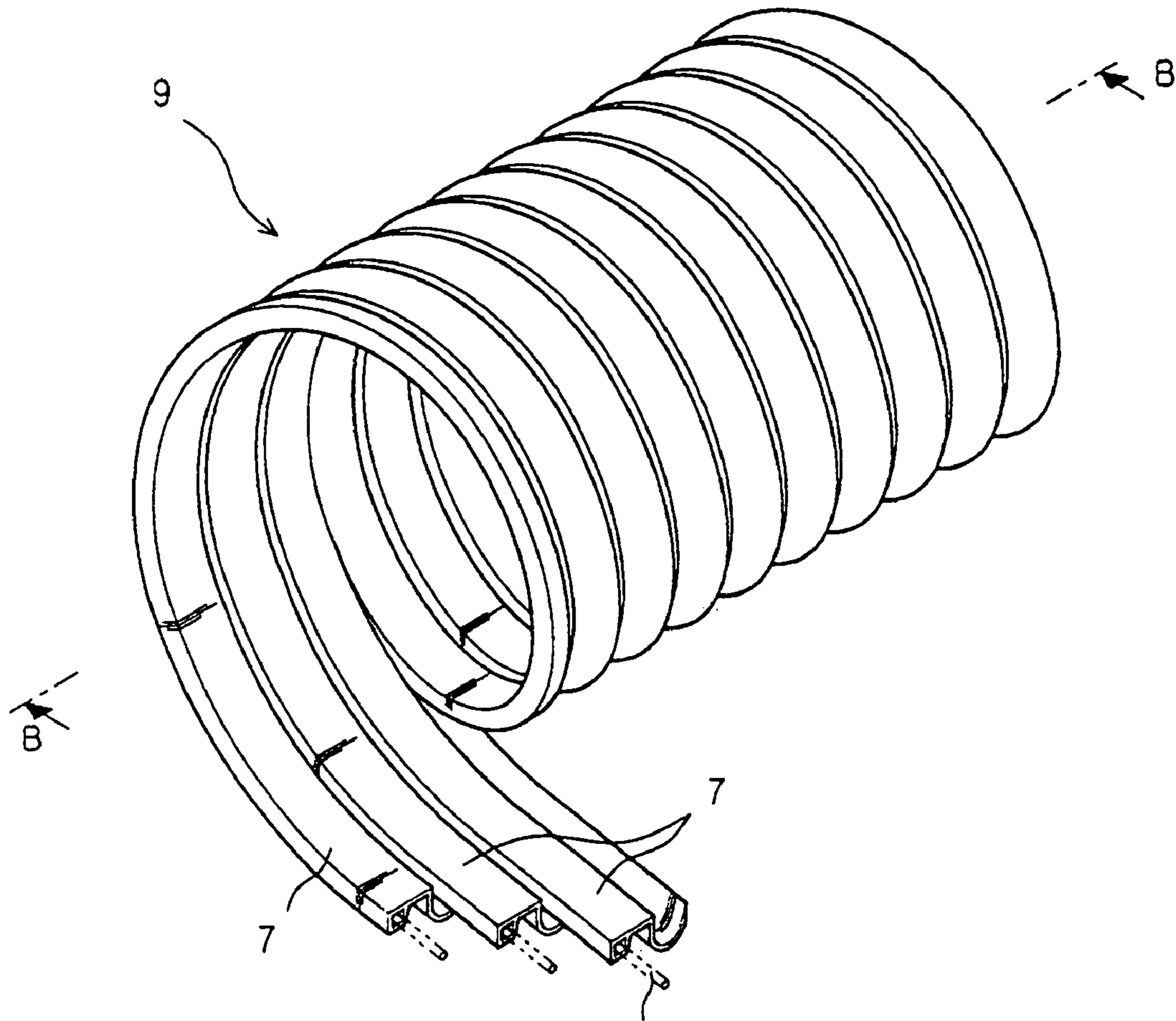
FIG. 8 (PRIOR ART)
