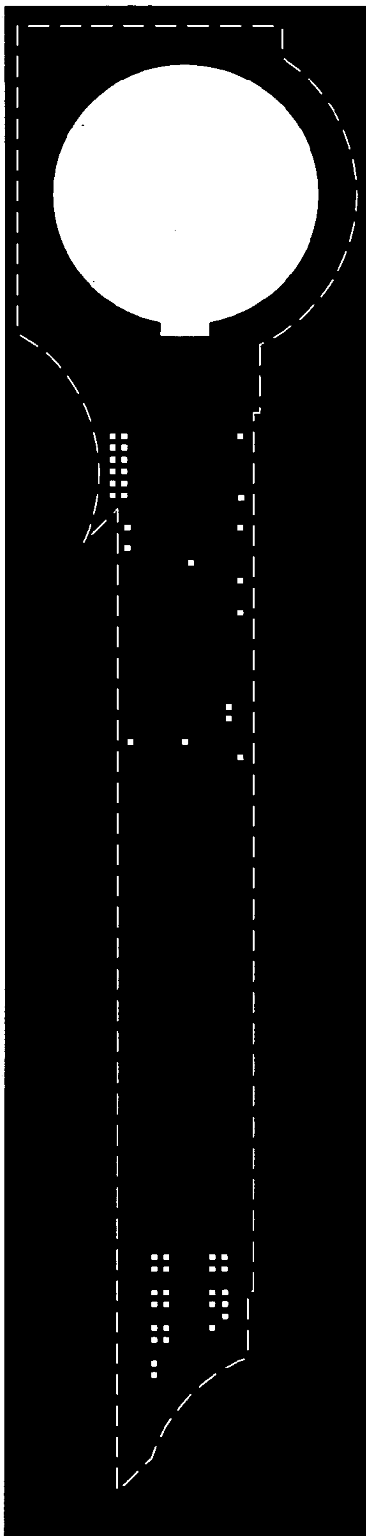
Via 1 mask
