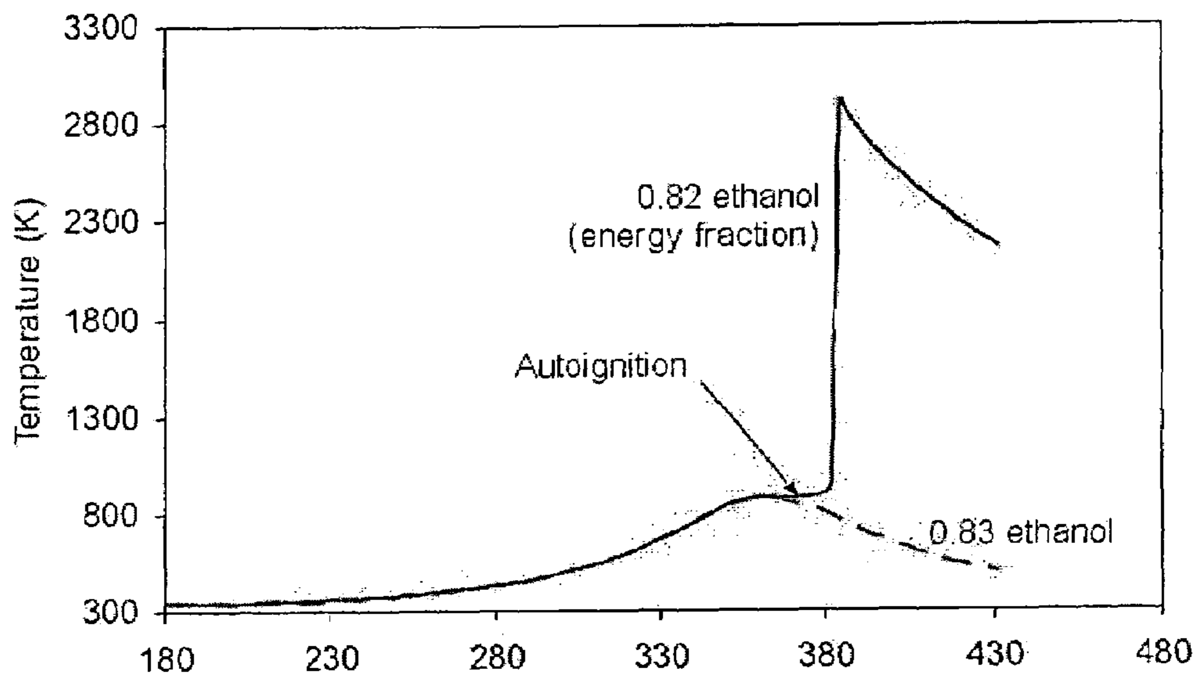
FIG. 2b Crank angle
