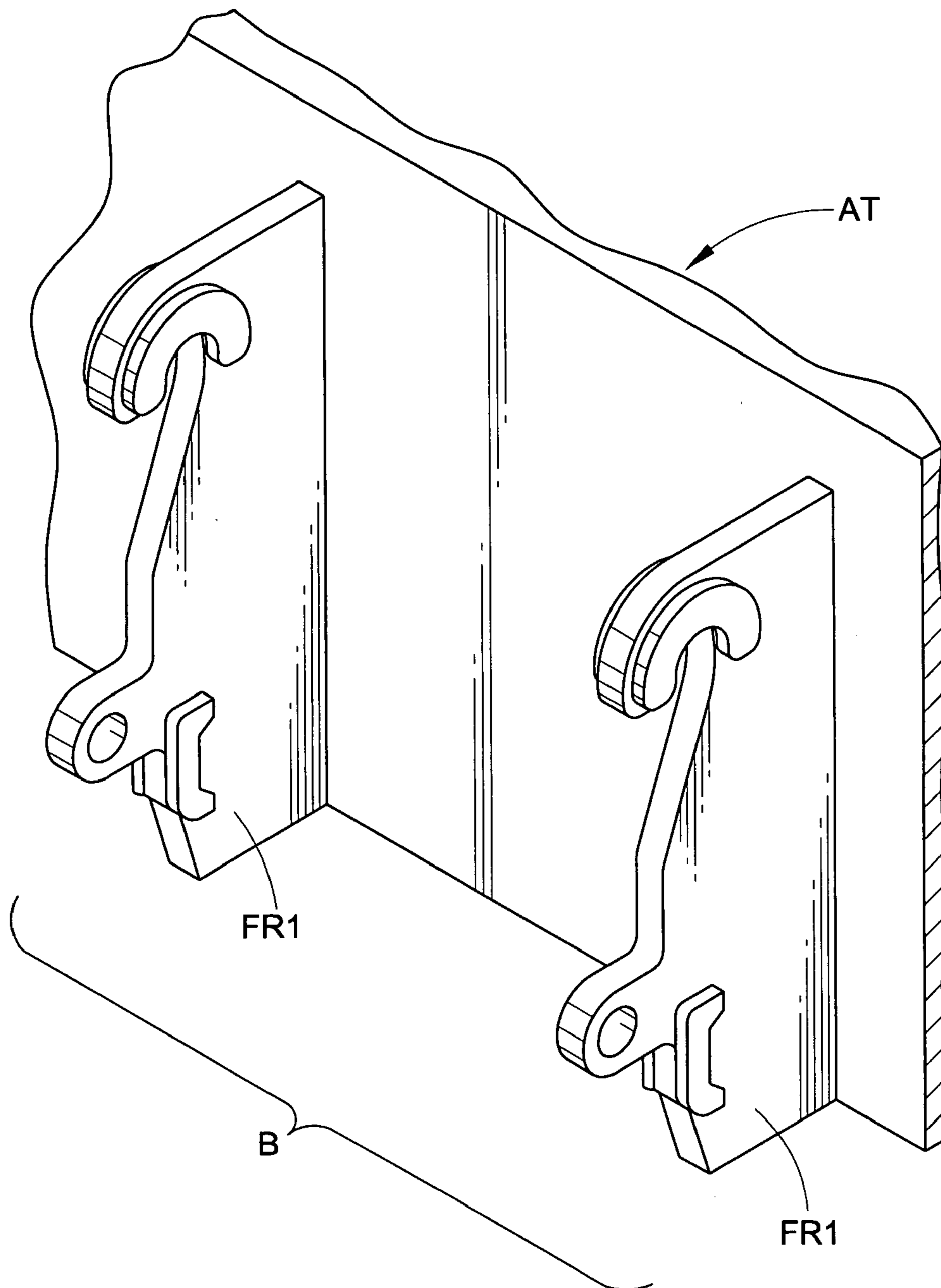
FIG. 1C (PRIOR ART)
