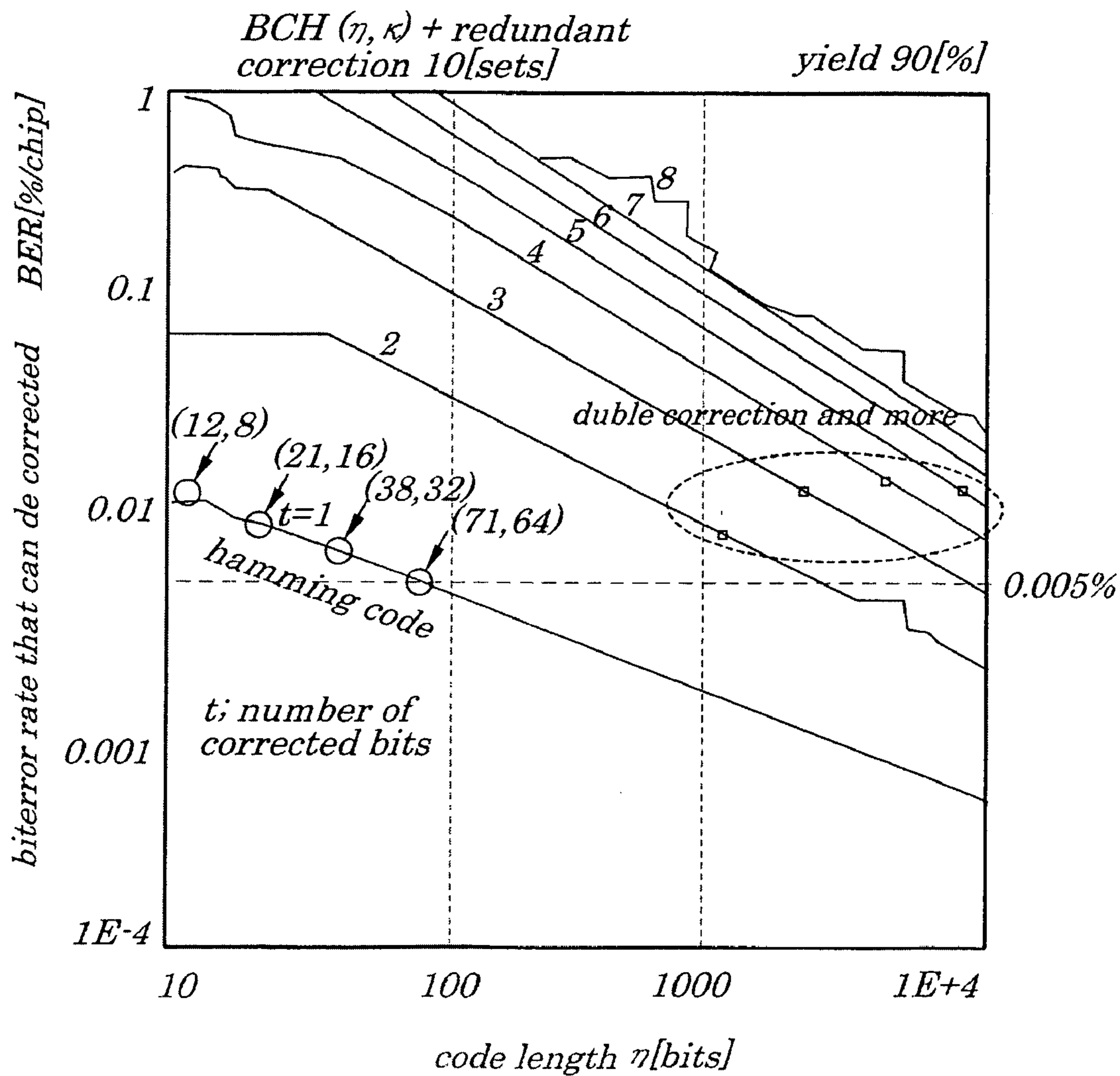
FIG. 19 RELATED ART
