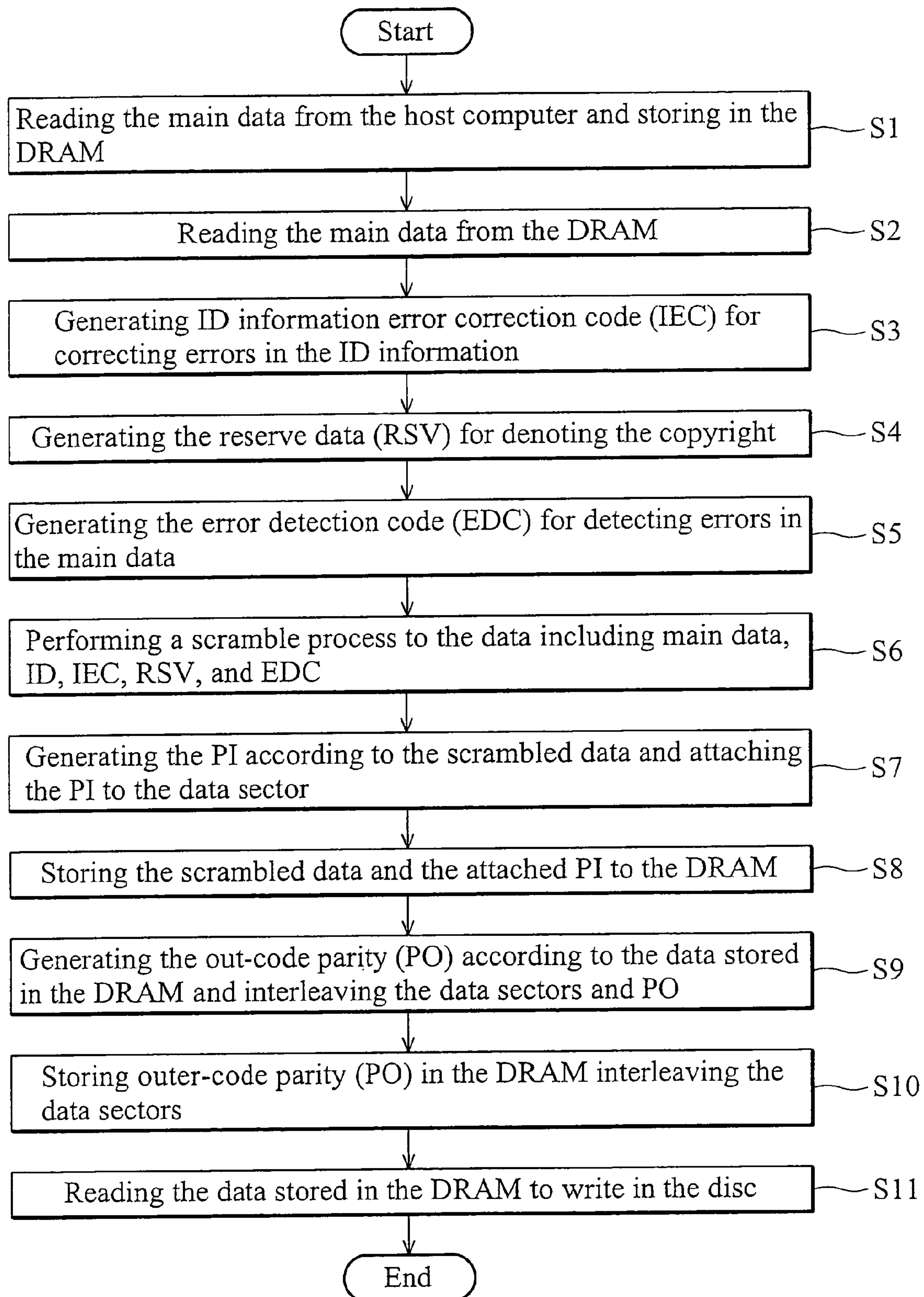
FIG. 4 (RELATED ART)
