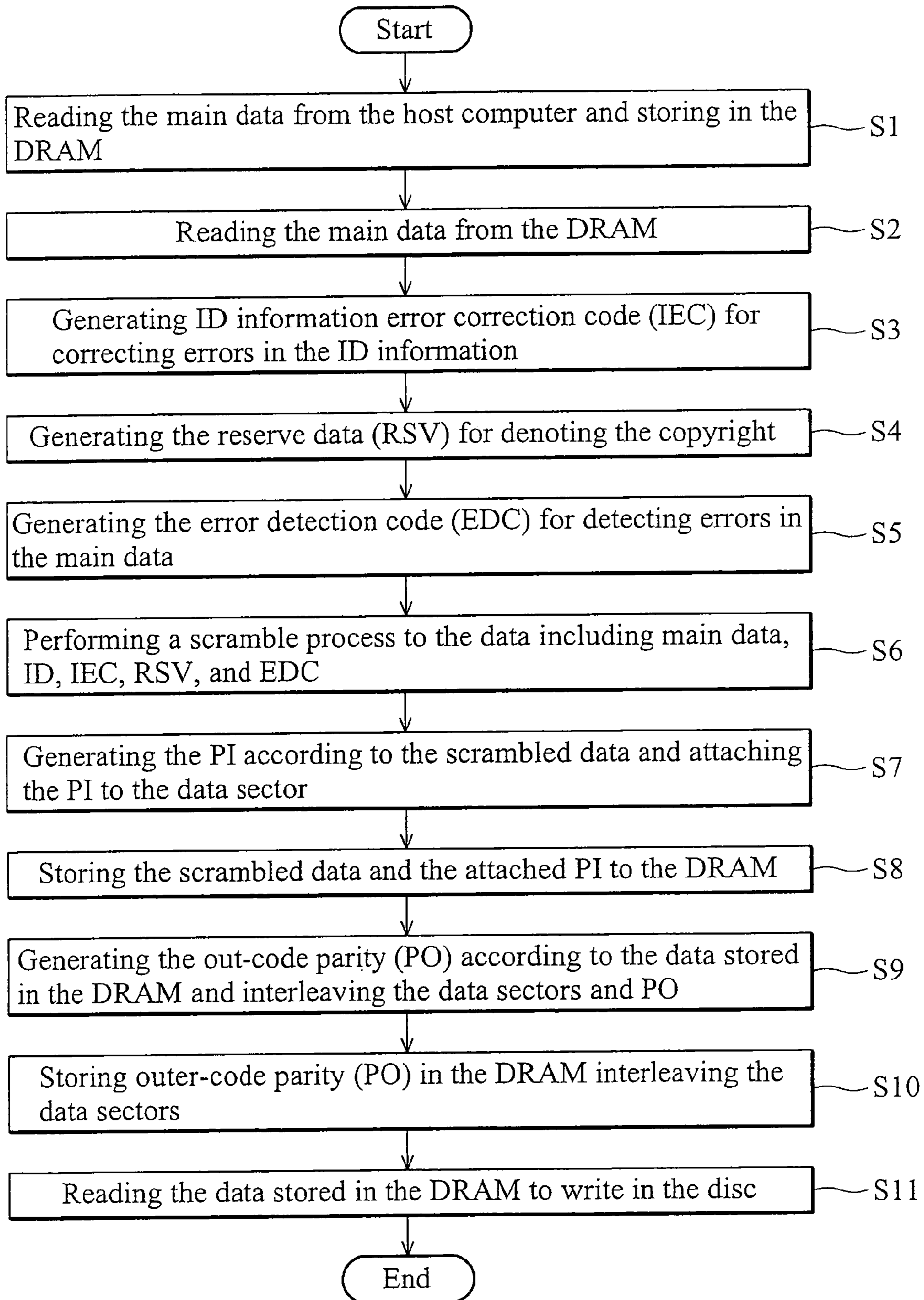
FIG. 4 (RELATED ART)
