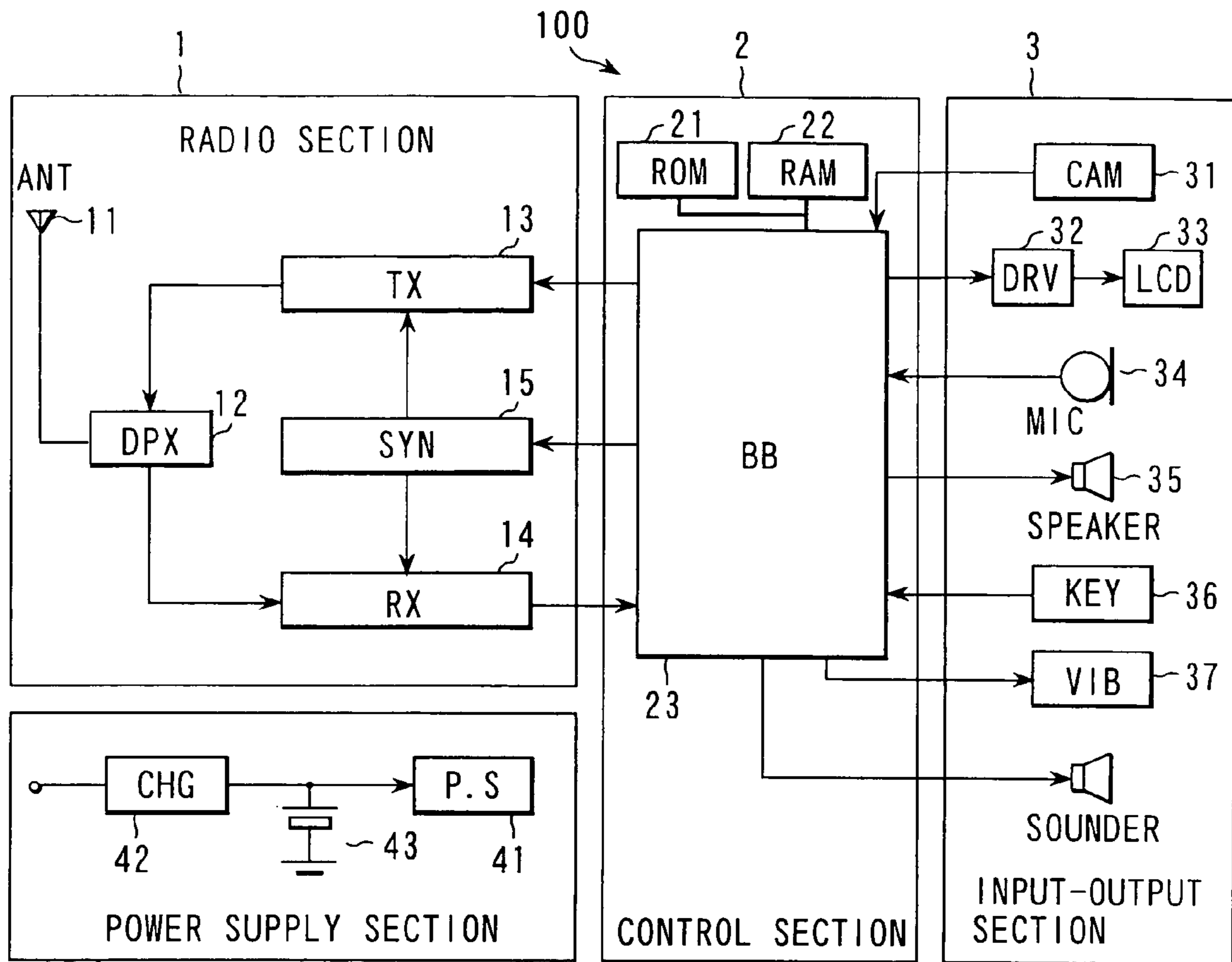
FIG. 7 RADIO COMMUNICATION TERMINAL
