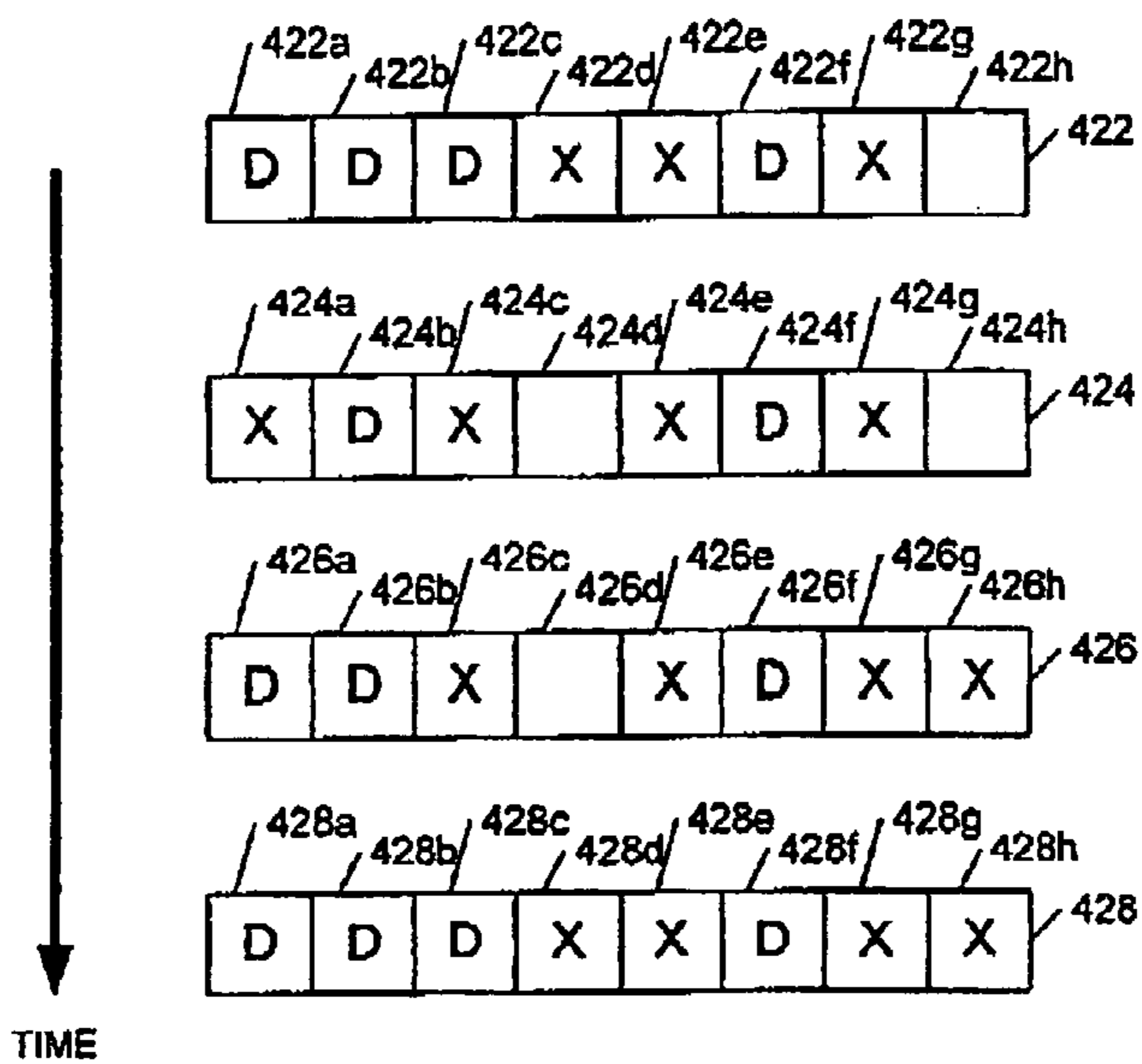
Figure 4b (PRIOR ART)
