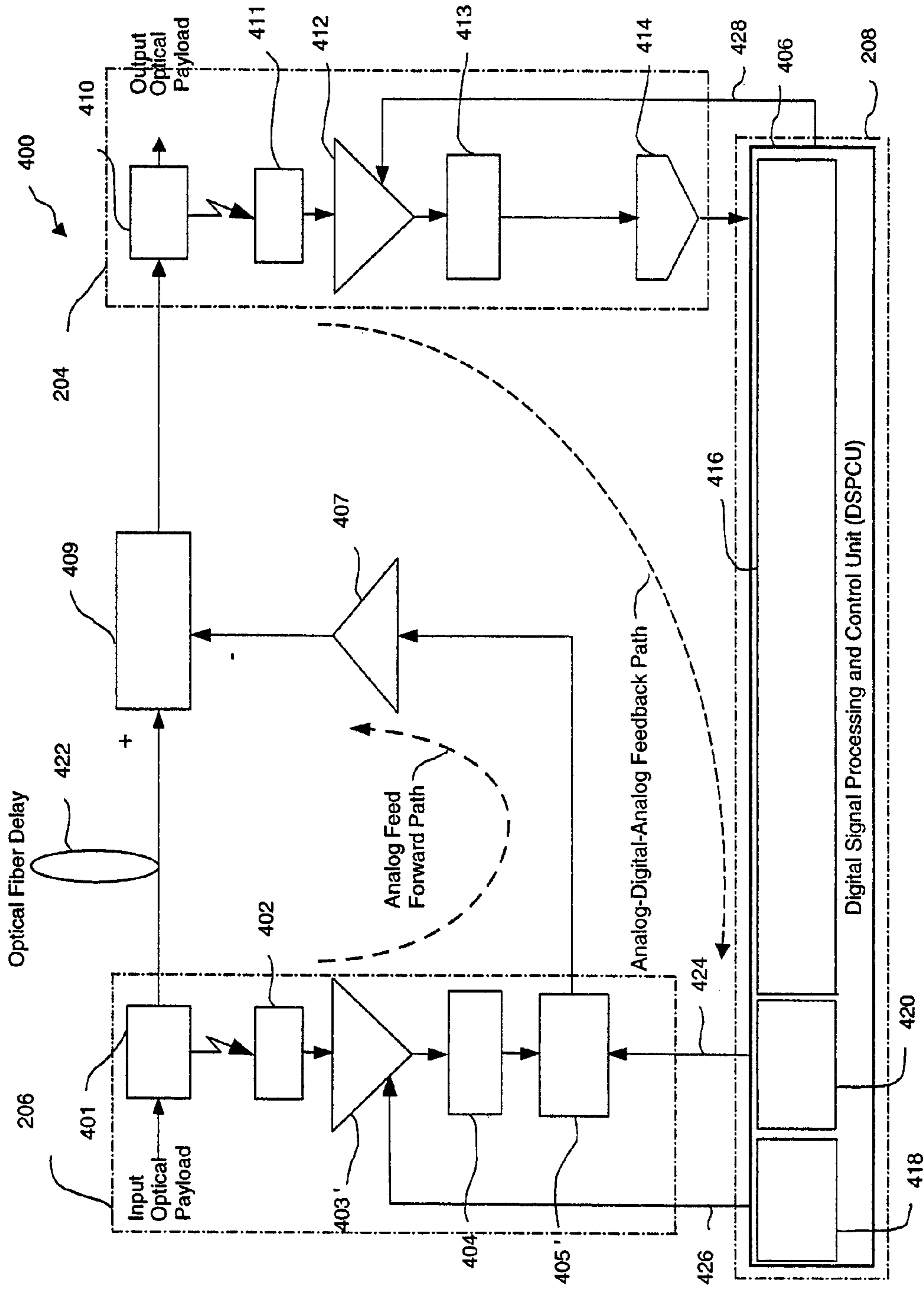
Figure 4. Detailed Payload Cancellation Scheme
