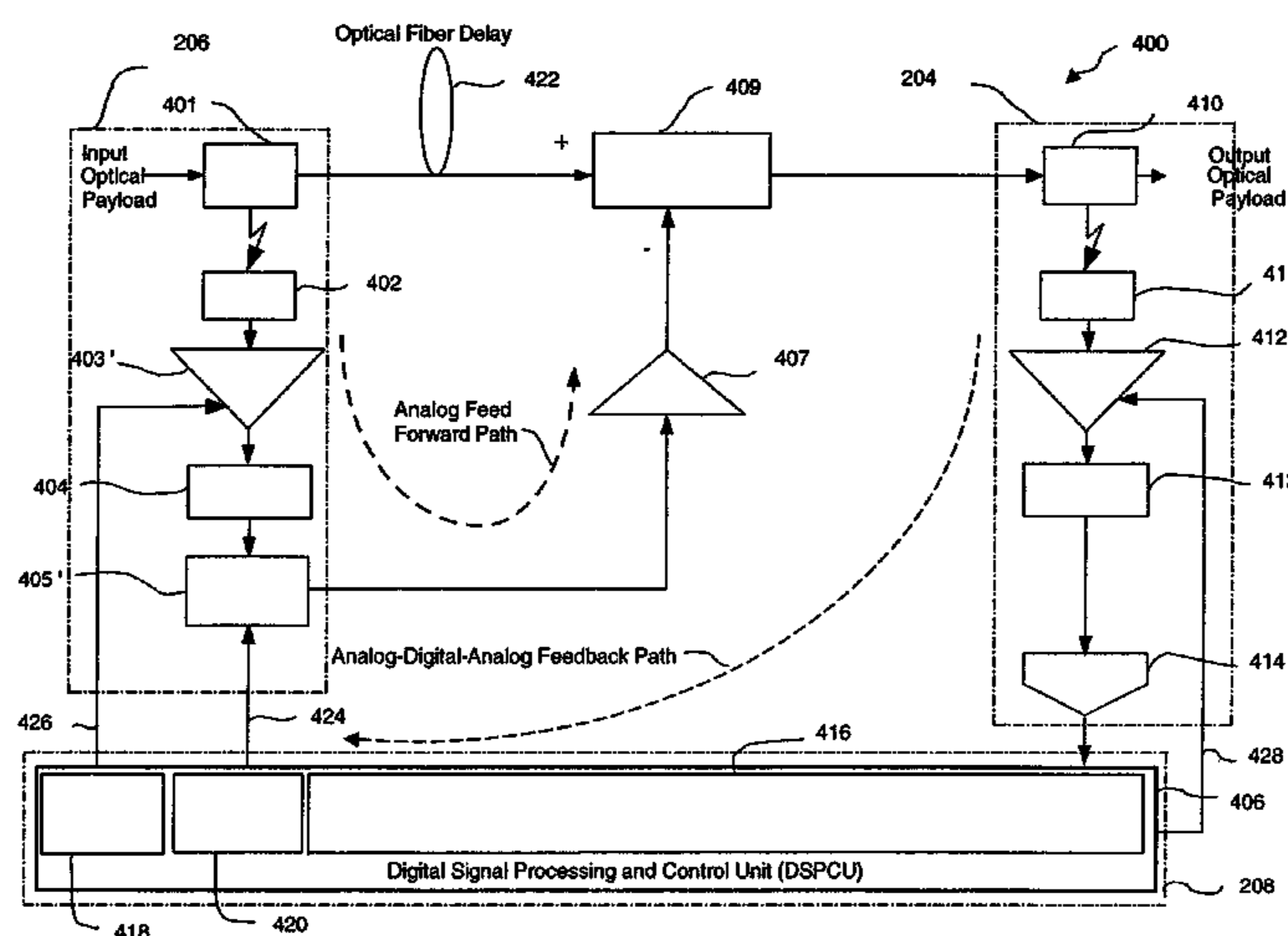
Detailed Payload Cancellation Scheme
