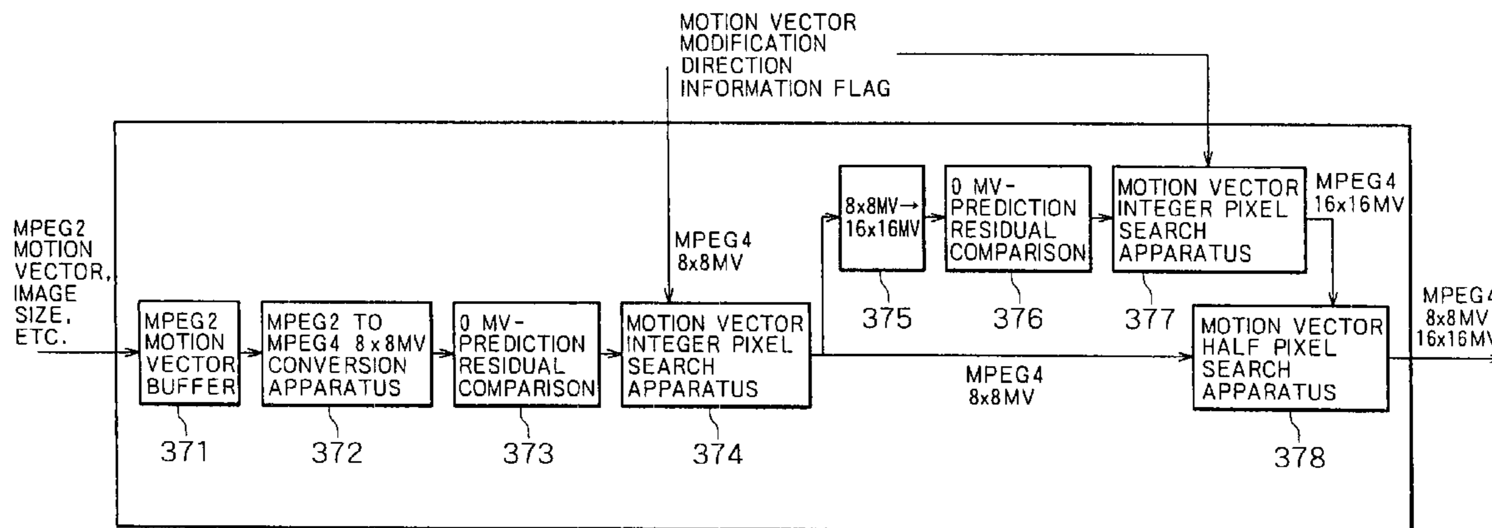
I TO P MOTION VECTOR CONVERSION APPARATUS
