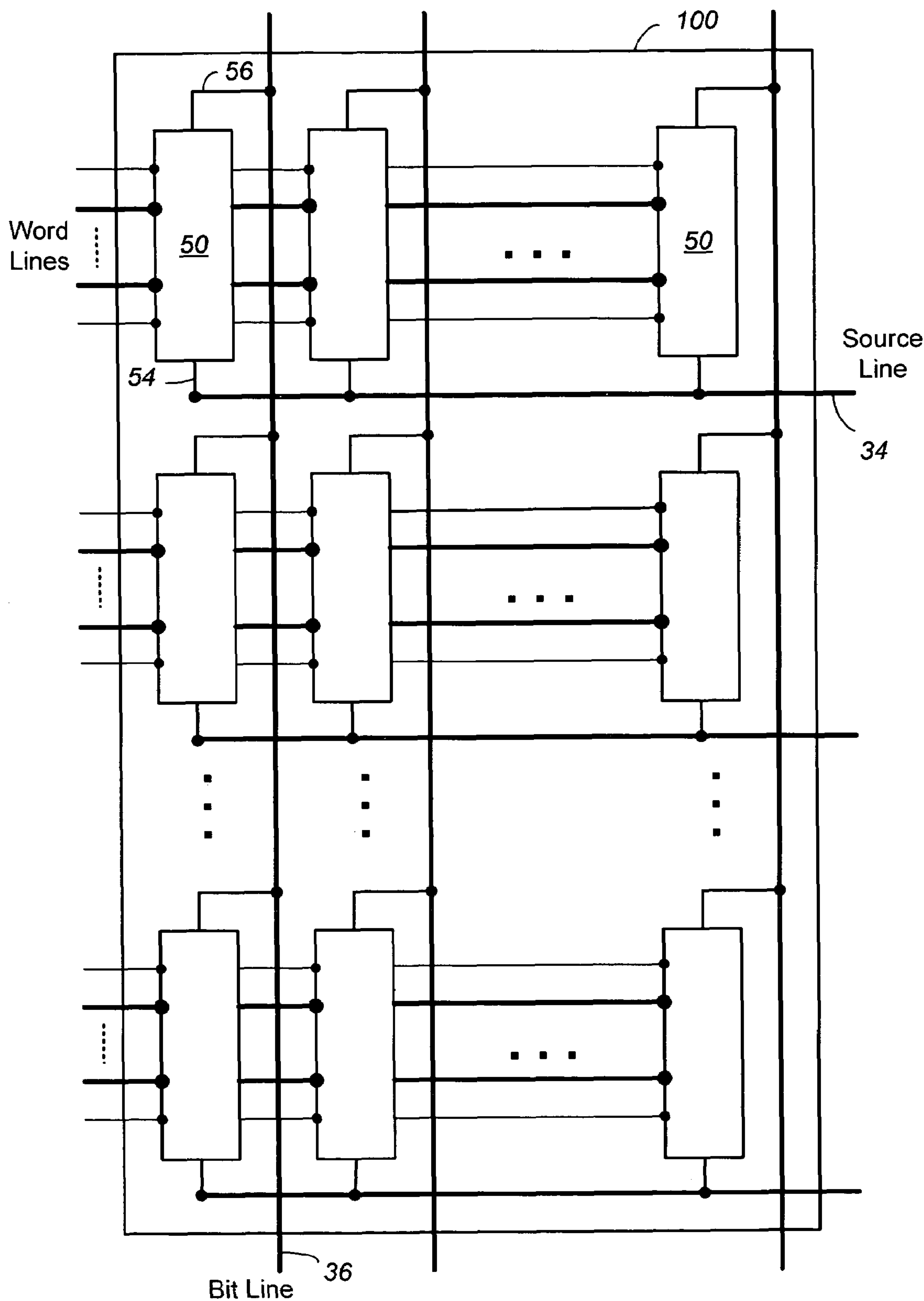
FIG. 3 (Prior Art)
