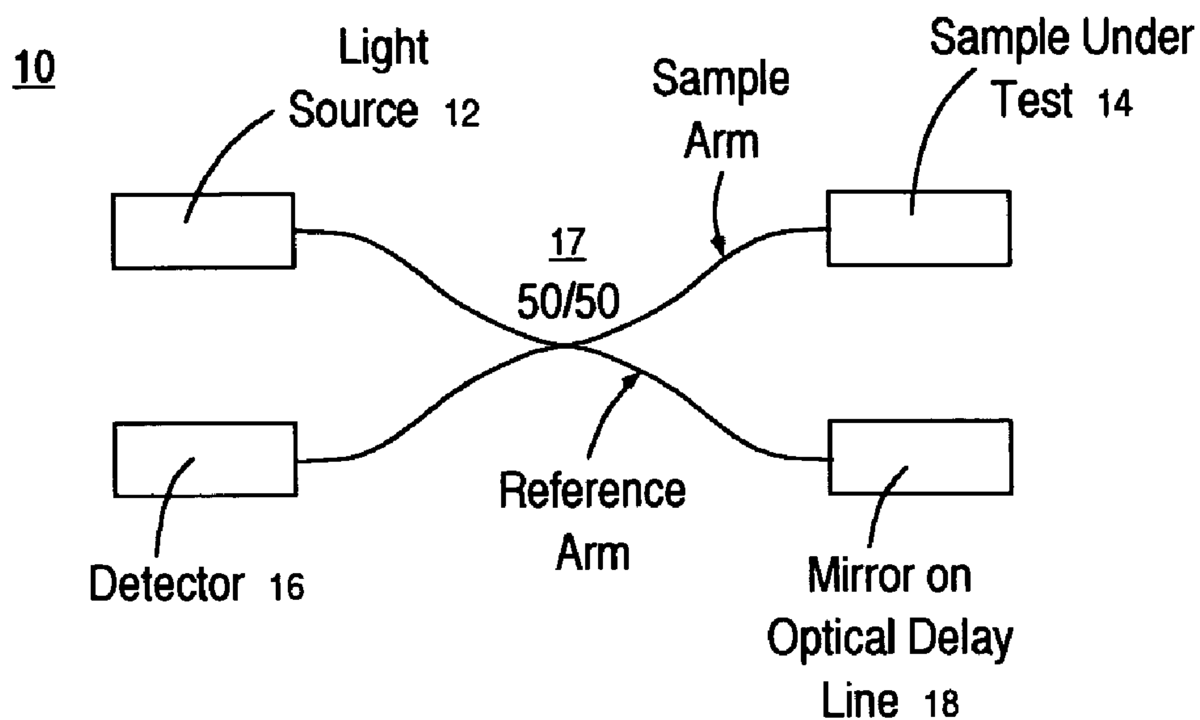
Figure 1 (Prior Art)
