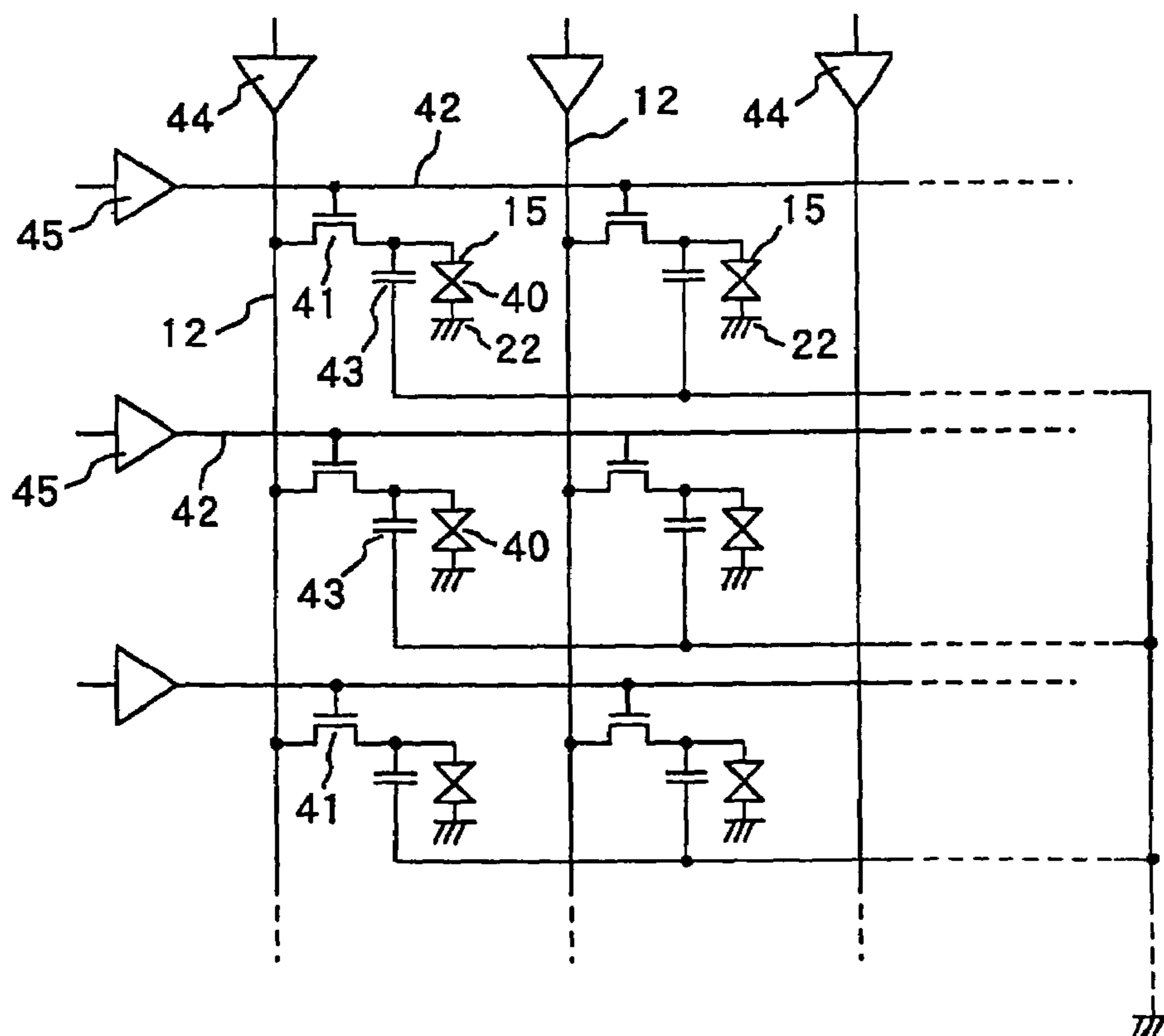
Fig. 2 (PRIOR ART)
