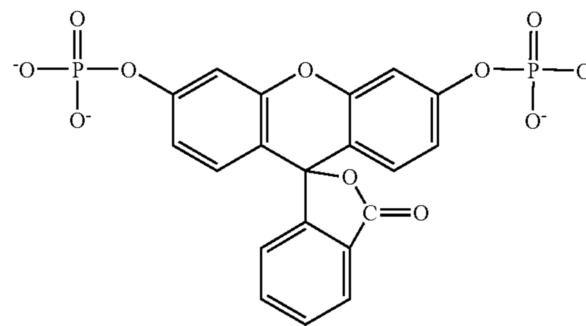
fluorescein diphosphate
