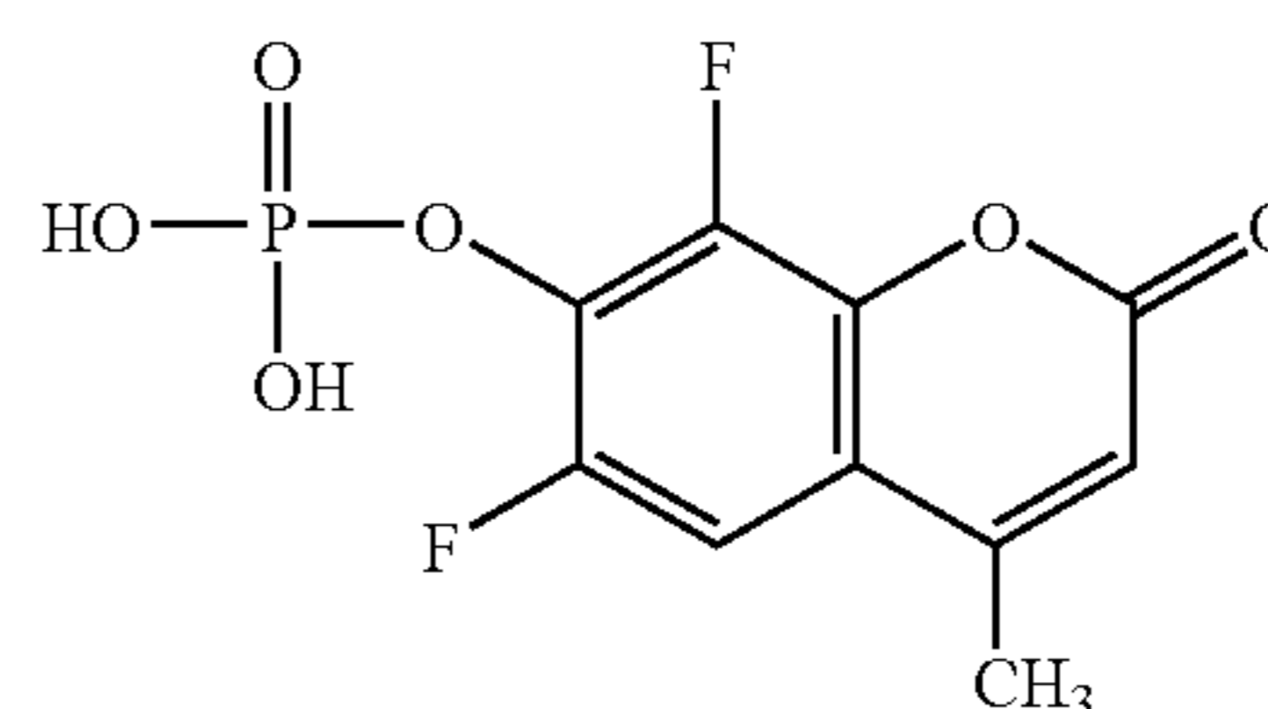
6,8-difluoro-4-methylumbelliferyl phosphate
