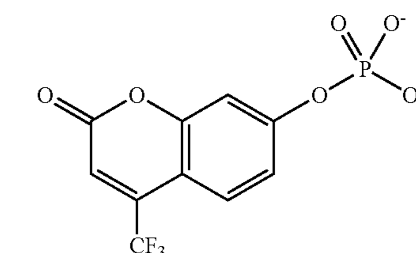
4-Trifluoromethylumbelliferyl phosphate
