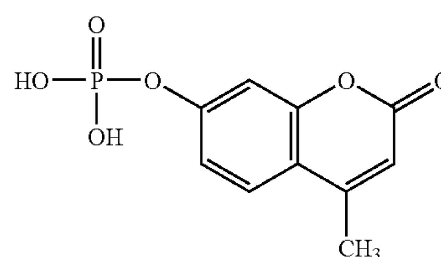
4-methylumbelliferyl phosphate
