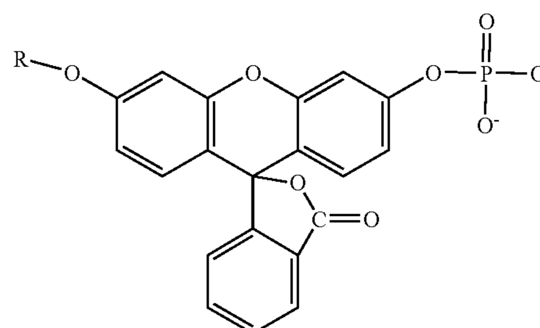
fluorescein 3'(6')-O-alkyl-6'(3')-phosphate
