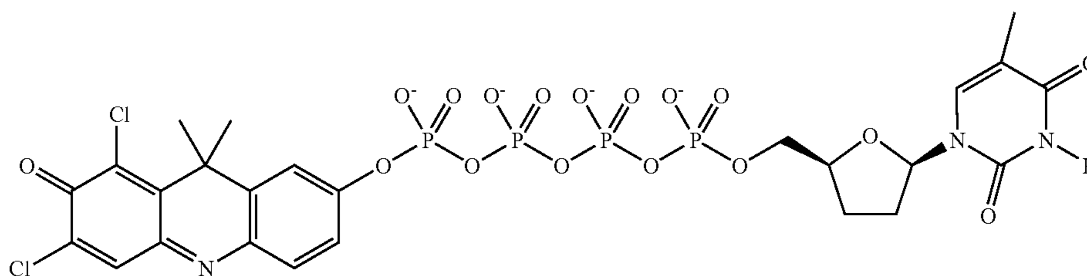
ddT4P-DDAO
