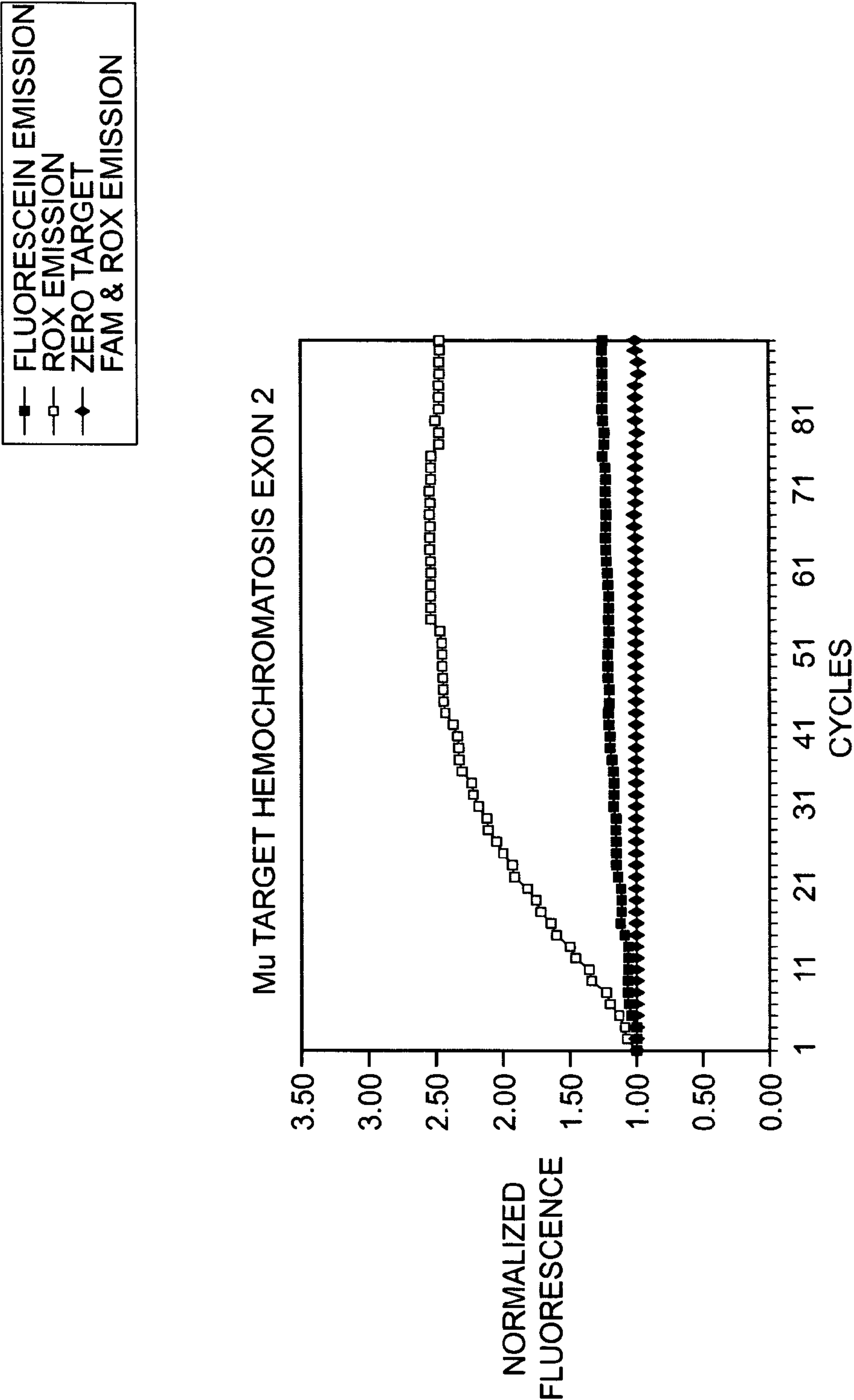
FIG. 4B TWO-COLOR SNP ANALYSIS ON PROBE TEC
