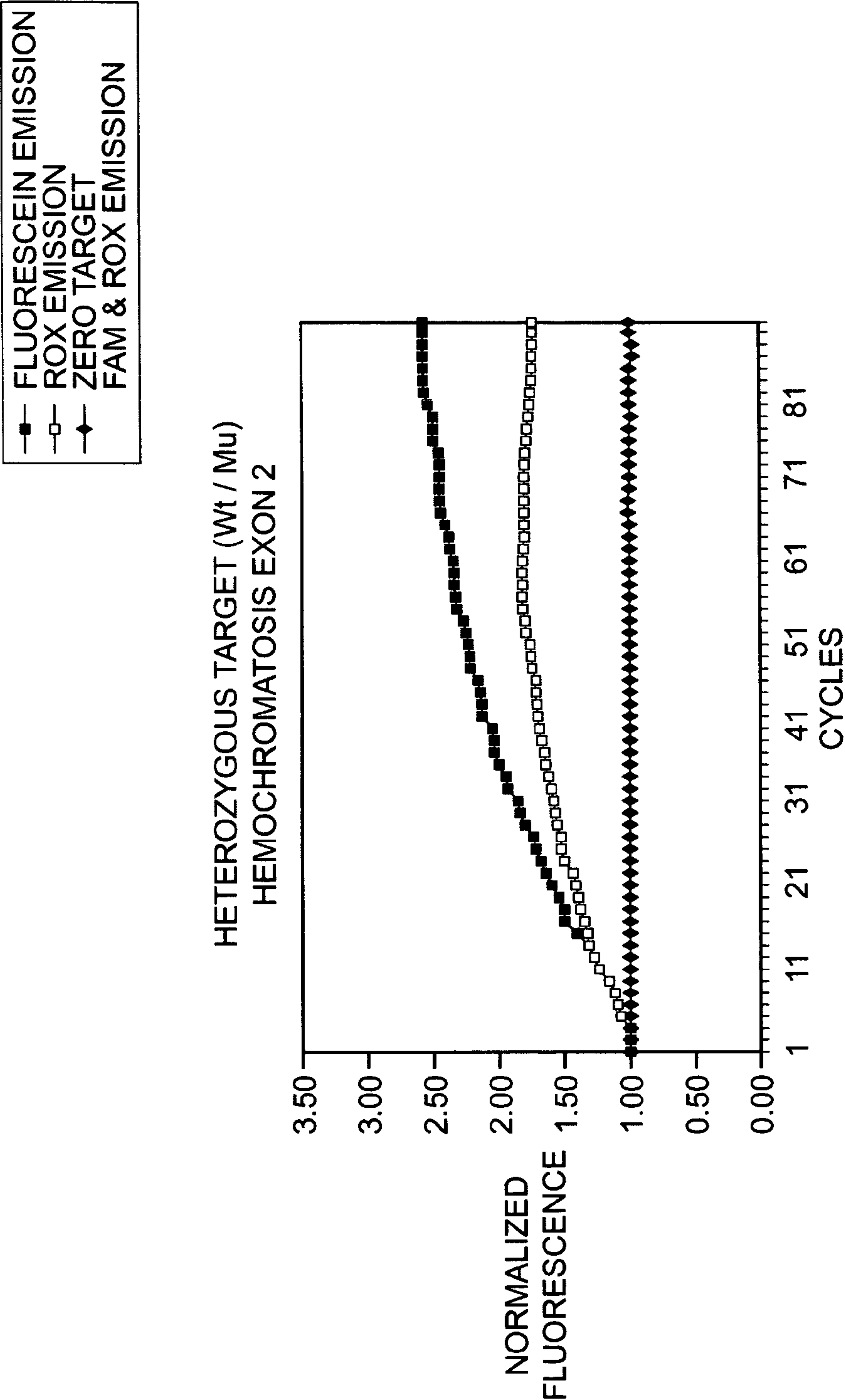
FIG. 4C TWO-COLOR SNP ANALYSIS ON PROBE TEC
