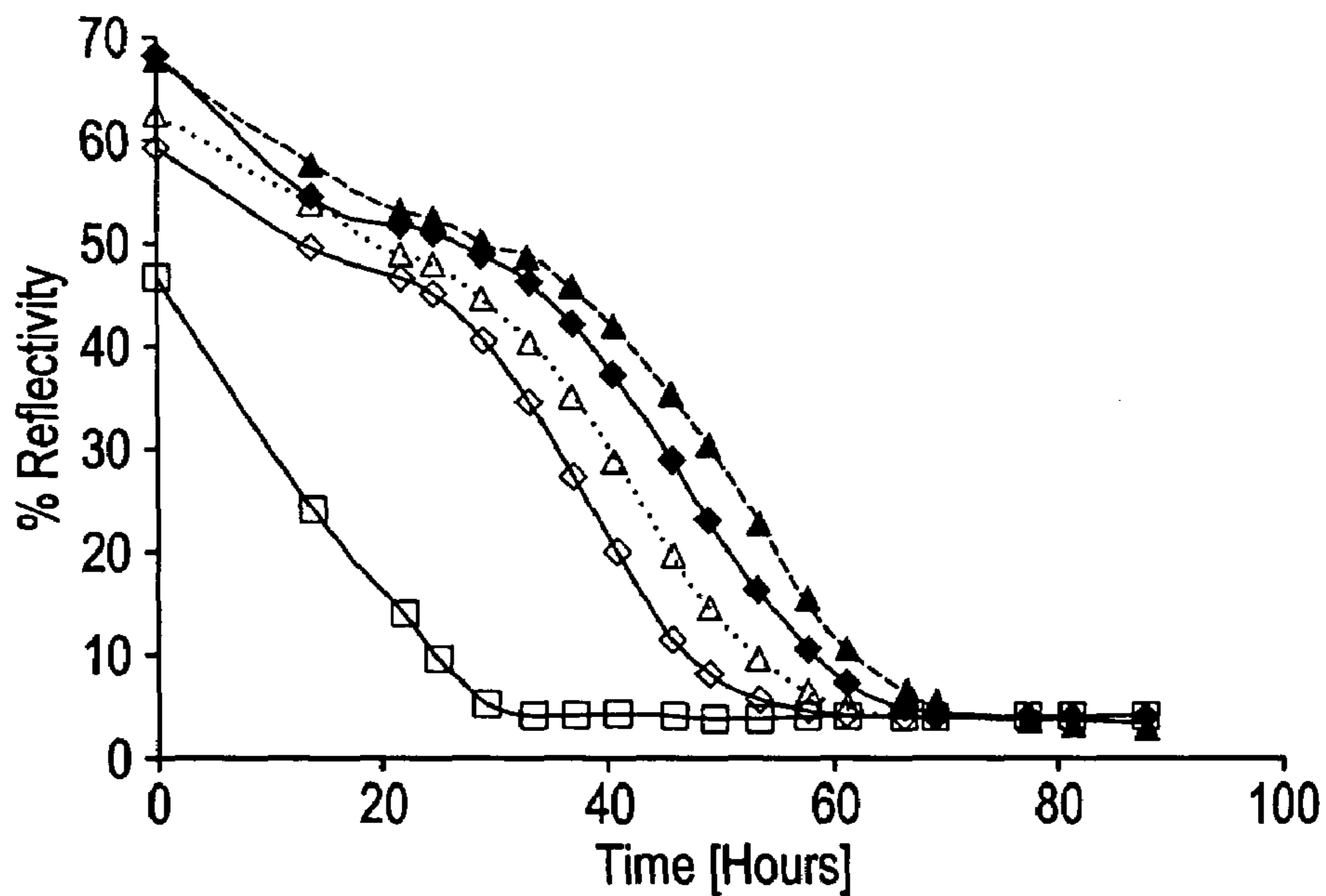
Comparison of Kinetics of Samples With and Without Barrier Coating
