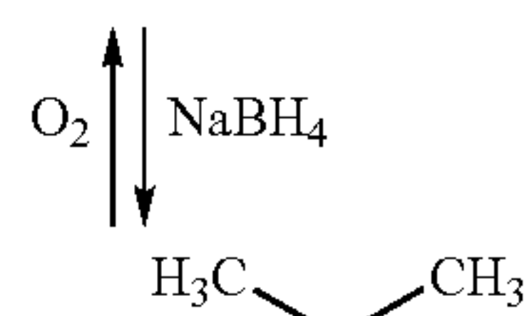
oxidized form
