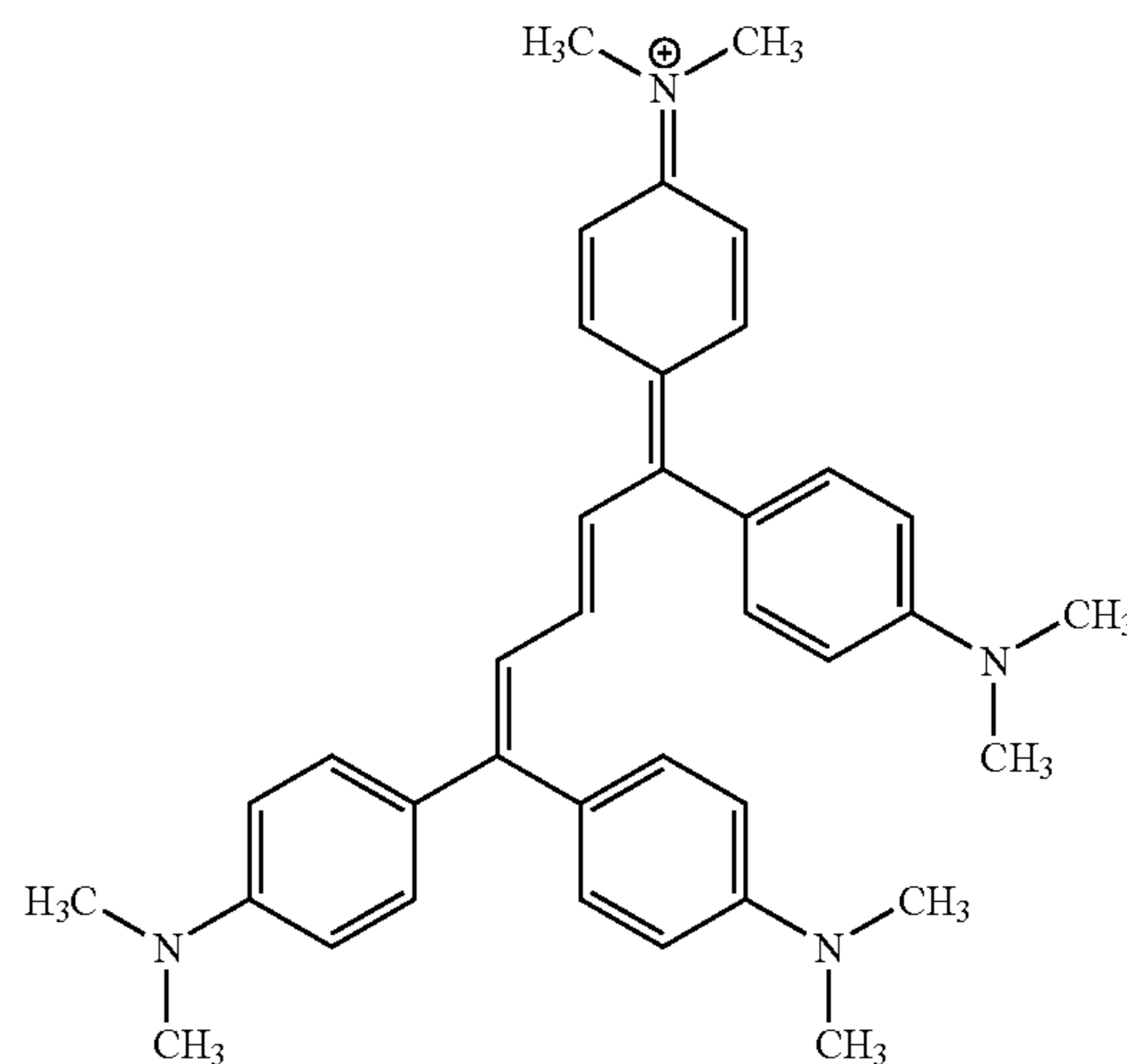
oxidized form
