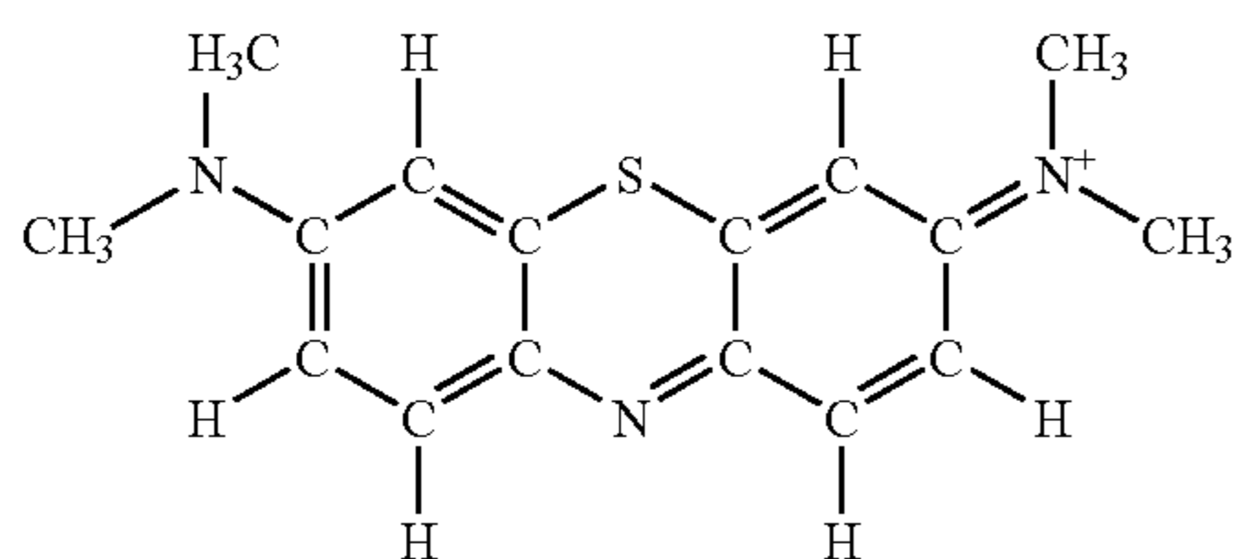
methylene blue
