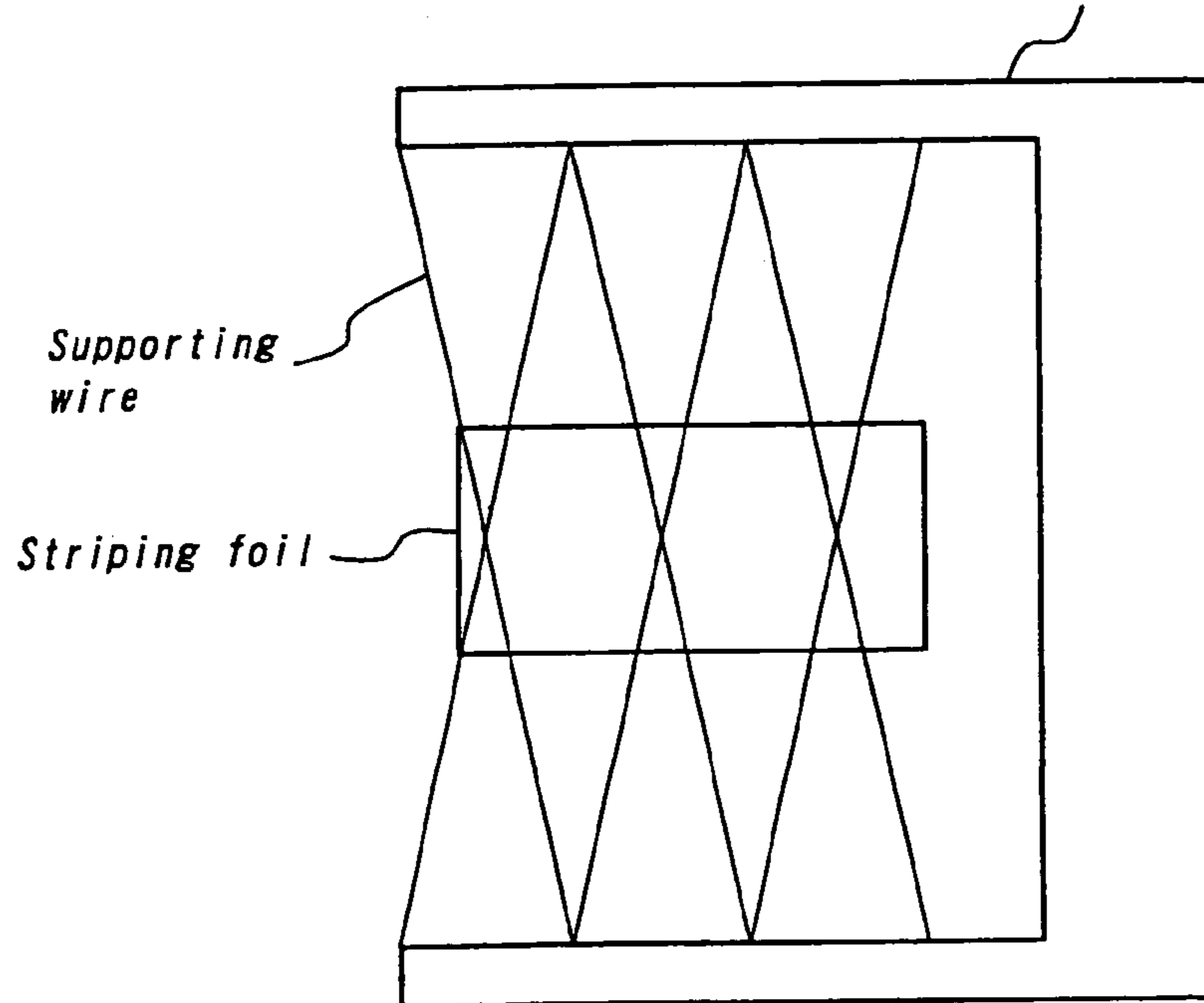
FIG. 4 Supporting frame
