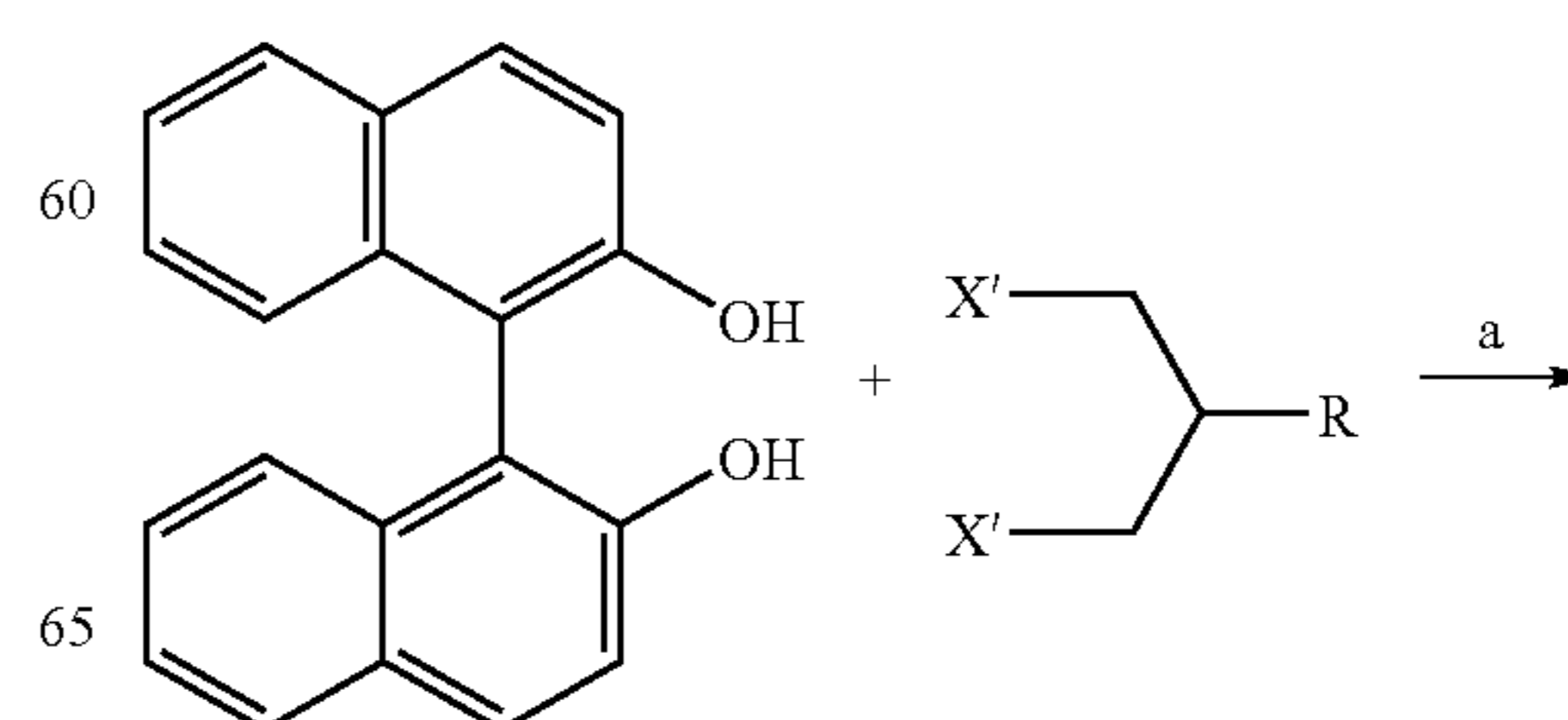
Scheme 1
