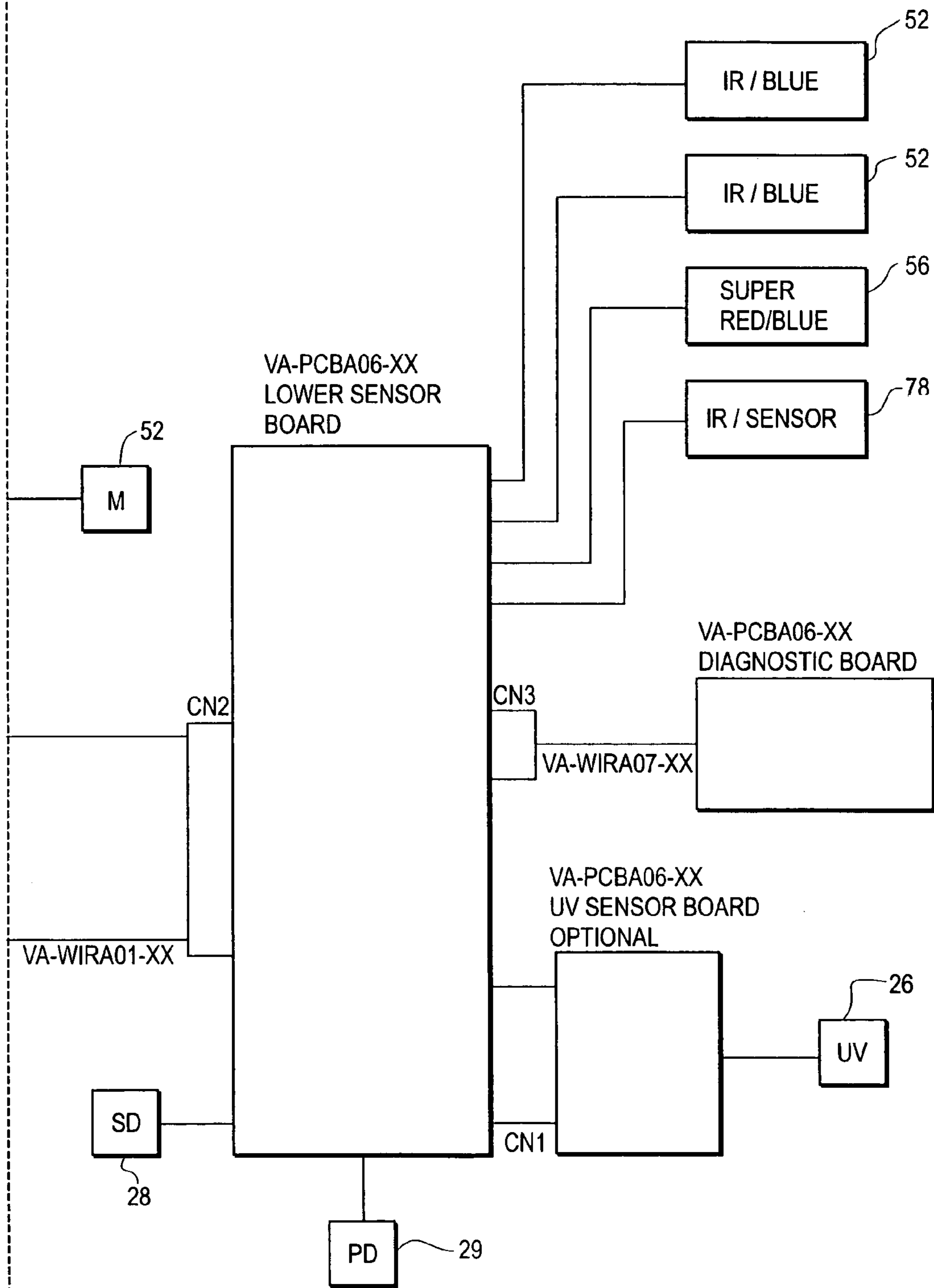
Fig. 6b LOWER HEAD ASSEMBLY
