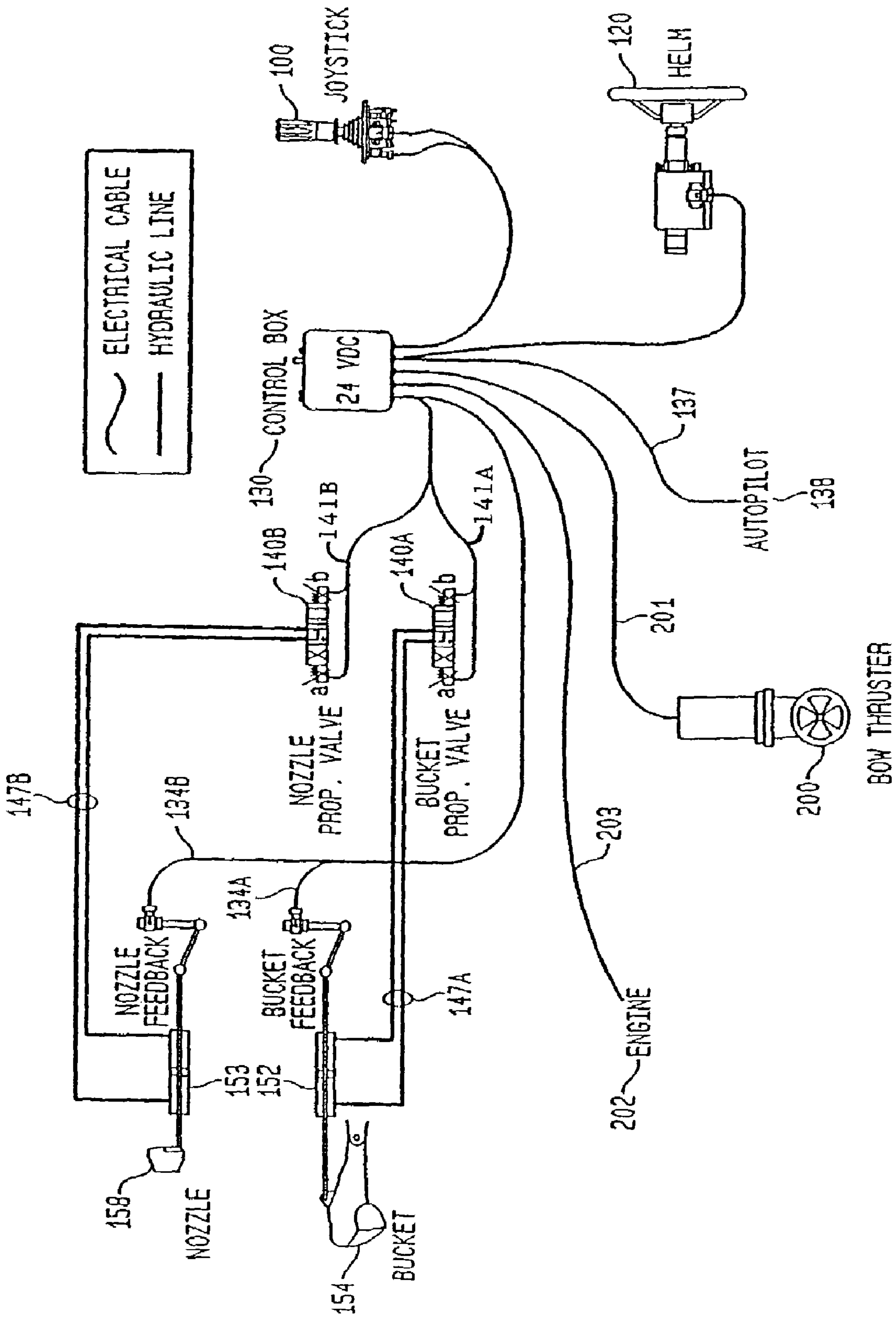
FIG. 6 SINGLE JET SYSTEM DIAGRAM
