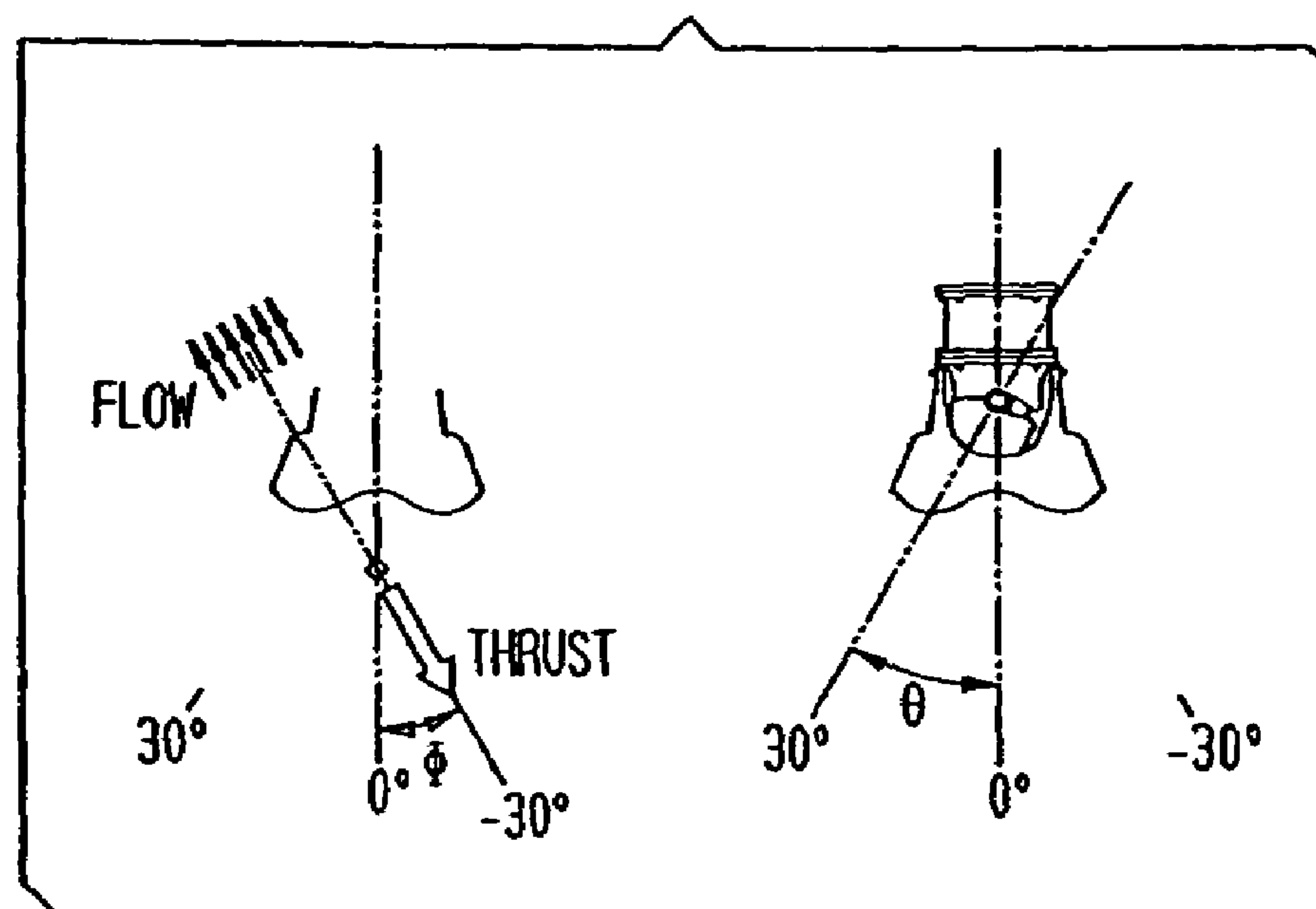
FIG. 25B FULL REVERSE BUCKET
