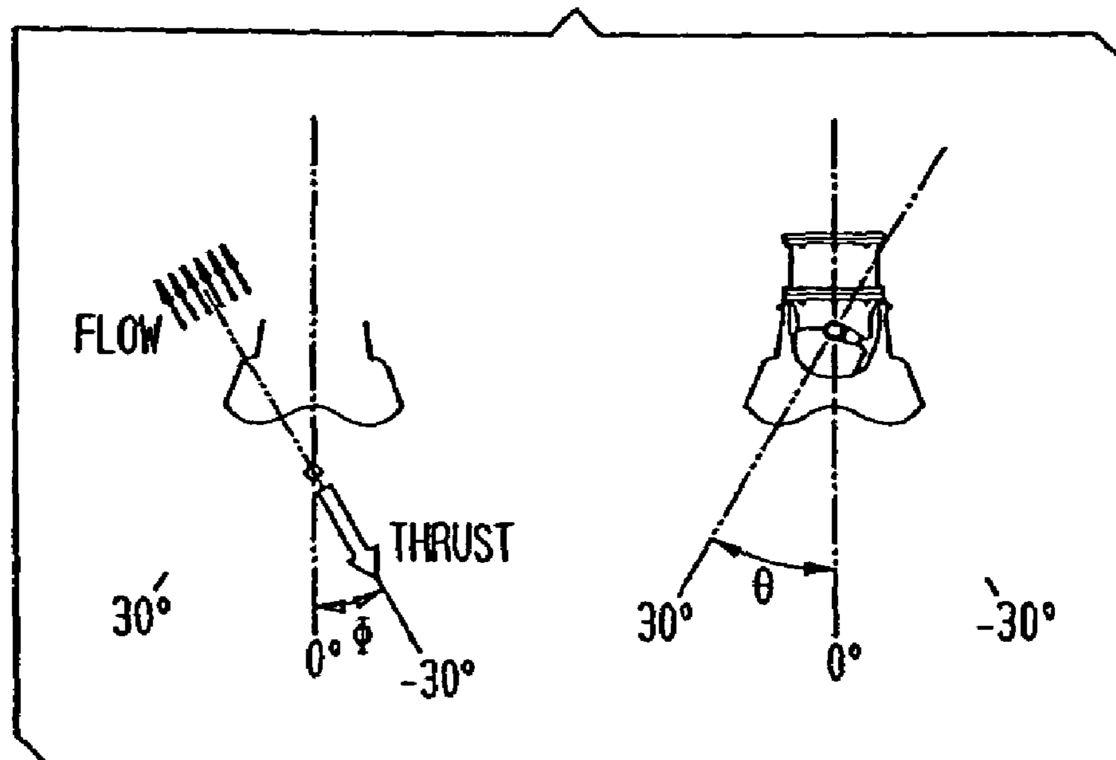
FIG. 25B FULL REVERSE BUCKET
