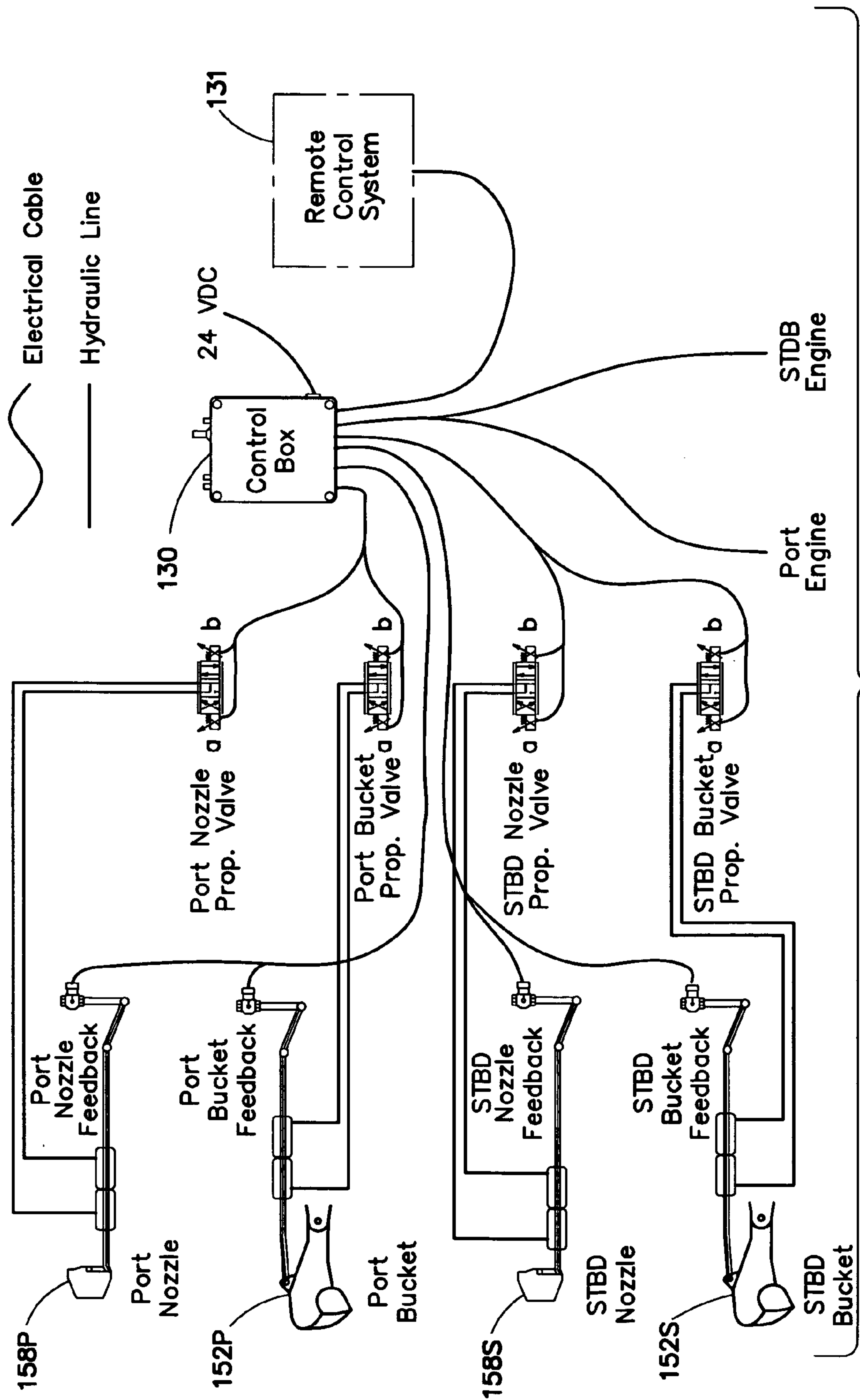
TWIN JET REMOTELY CONTROLLED SYSTEM DIAGRAM
