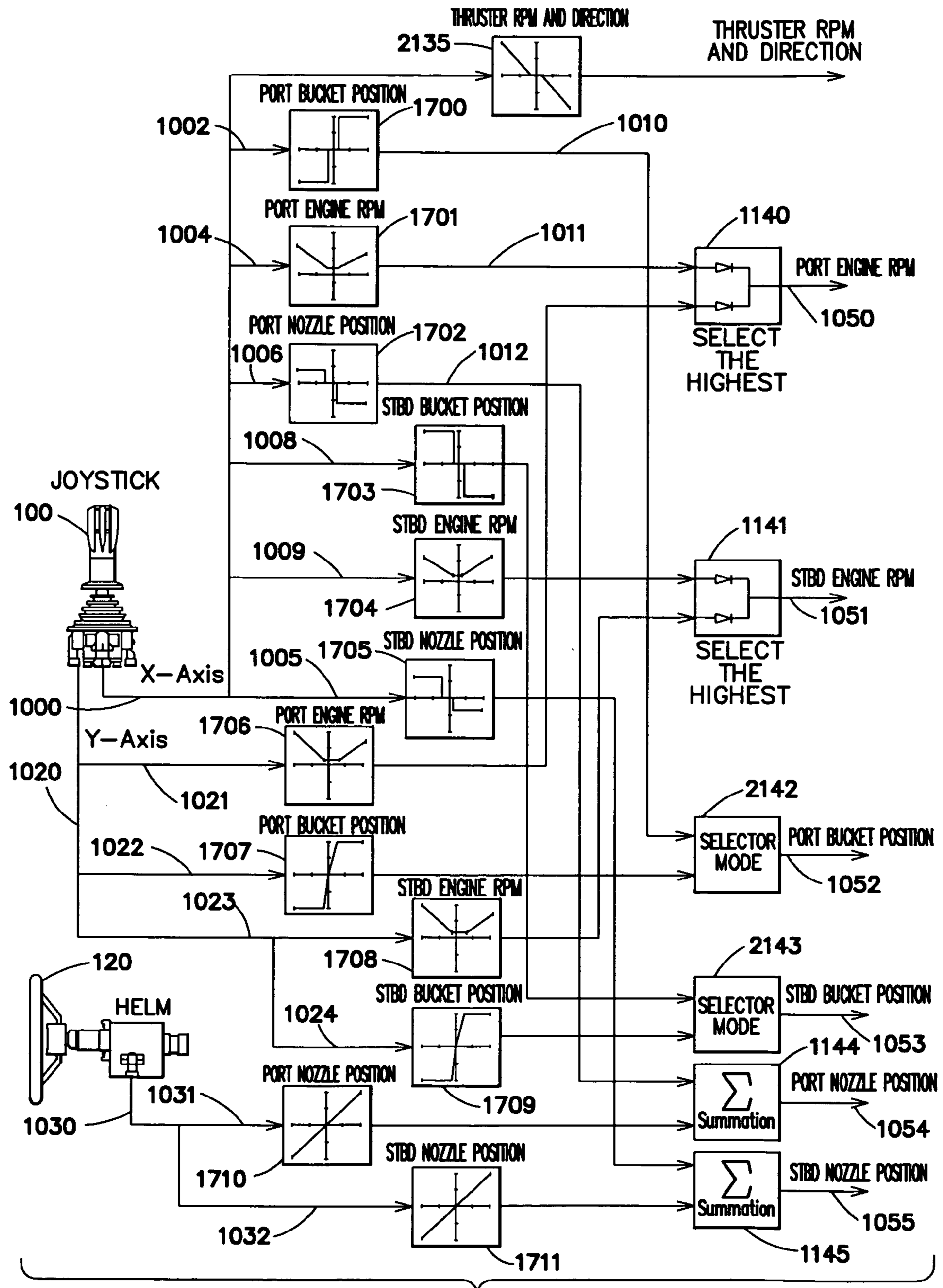
TWIN WATERJET SIGNAL DIAGRAM WITH BOWTHRUSTER
