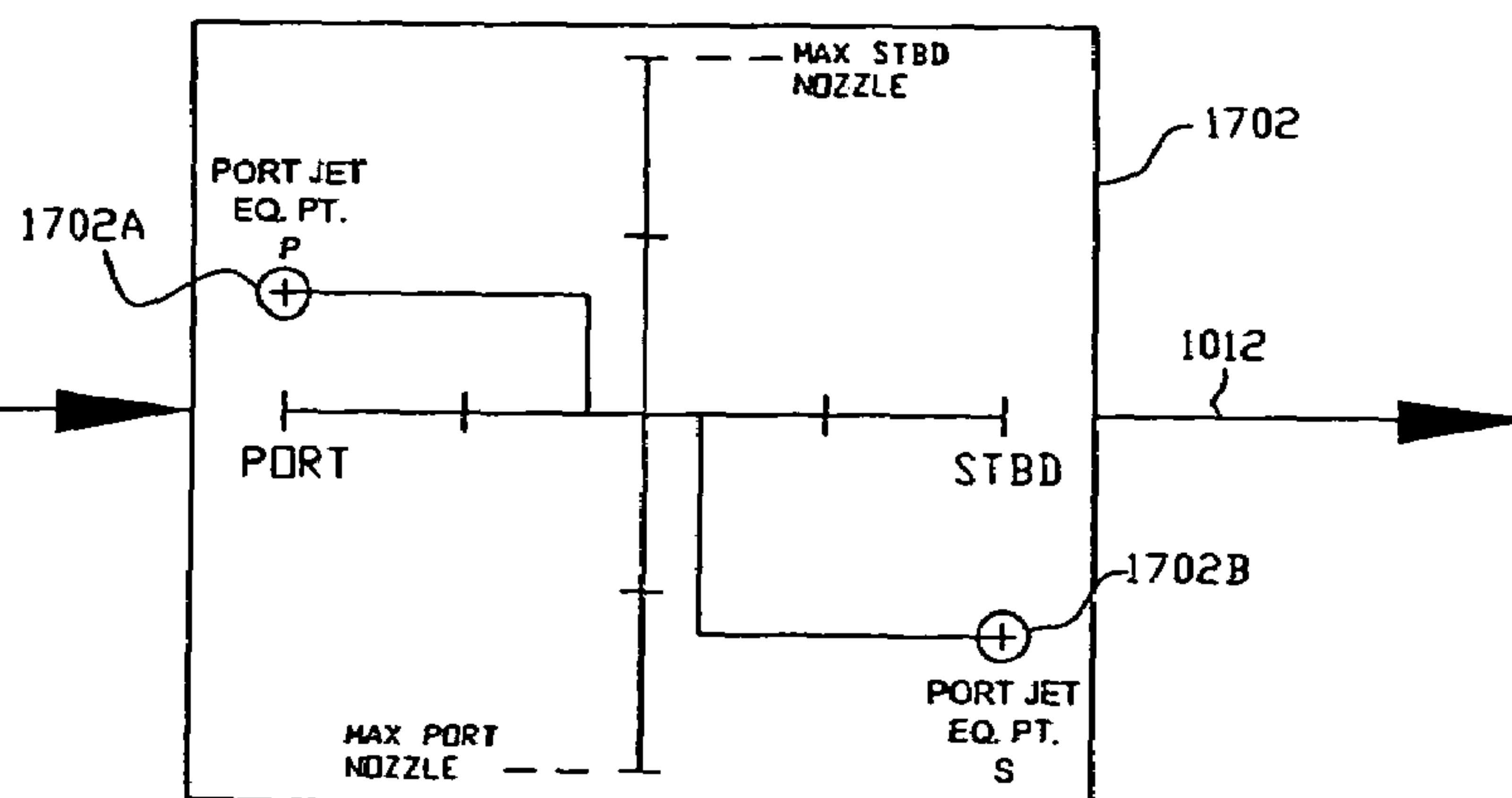
FIG. 14F PORT NOZZLE POSITION
