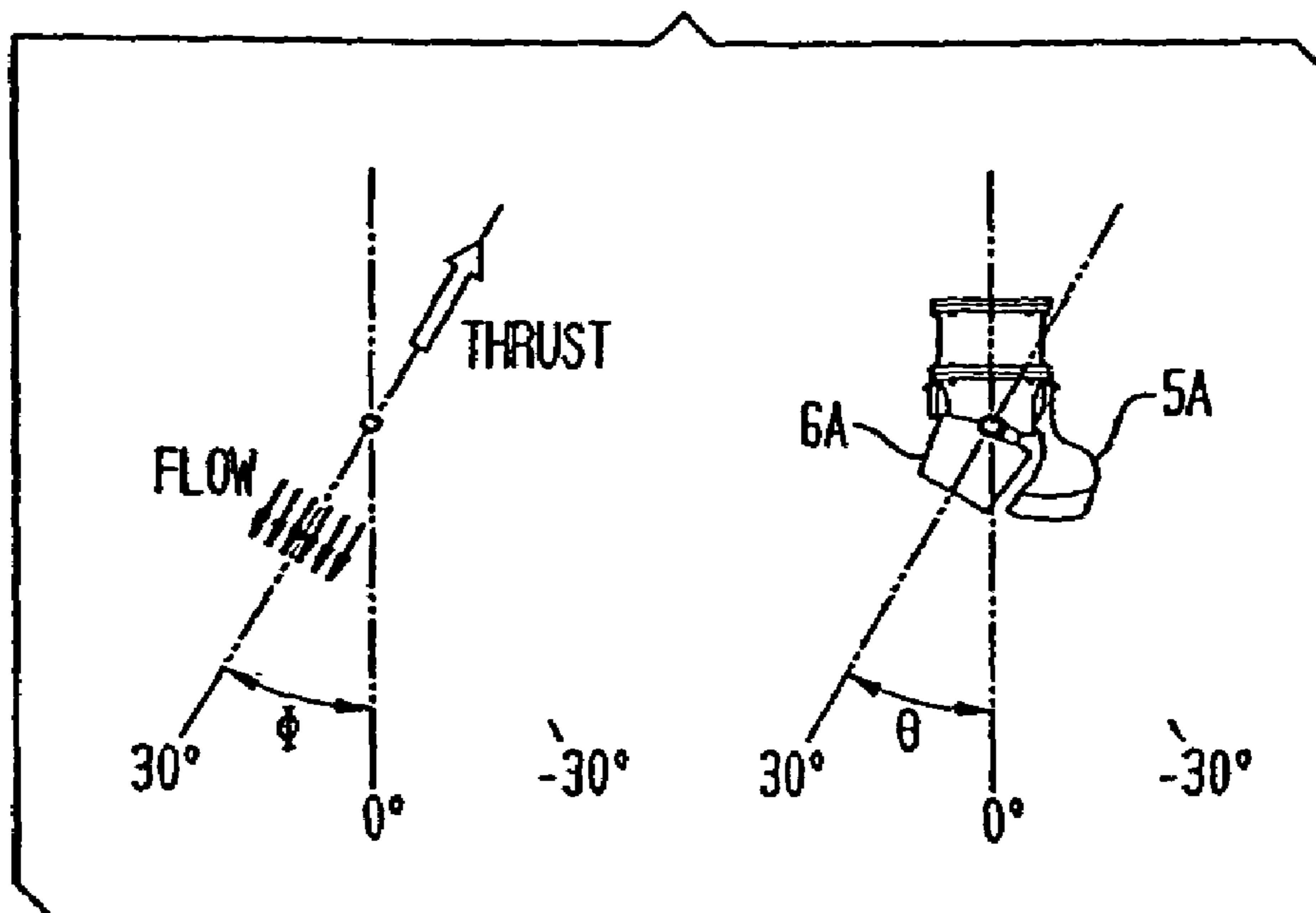
FIG. 25A FULL AHEAD BUCKET
