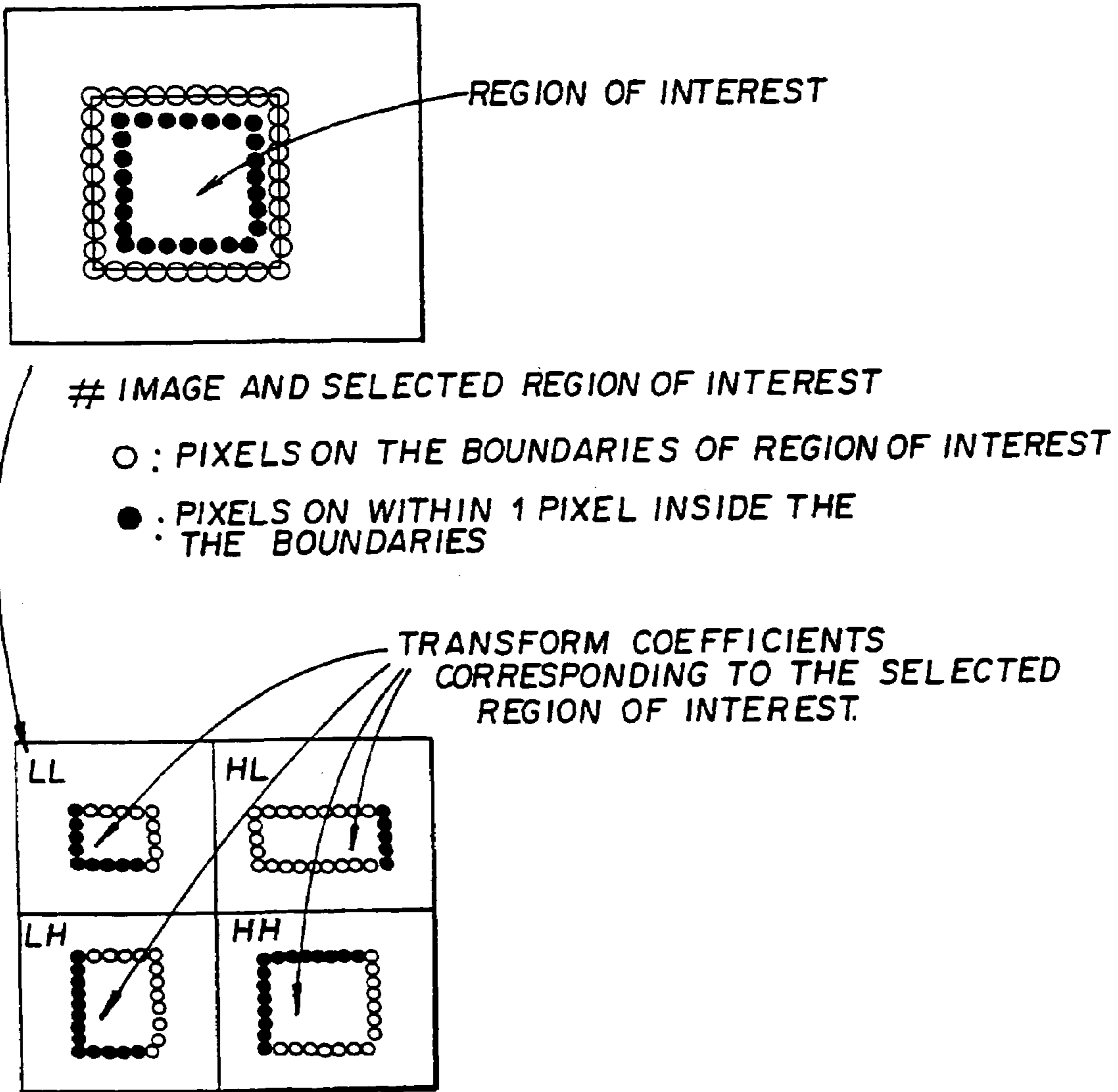
ROI COEFFICIENT IDENTIFICATION IN 1 LEVEL WAVELET DECOMPOSED SUBBANDS
