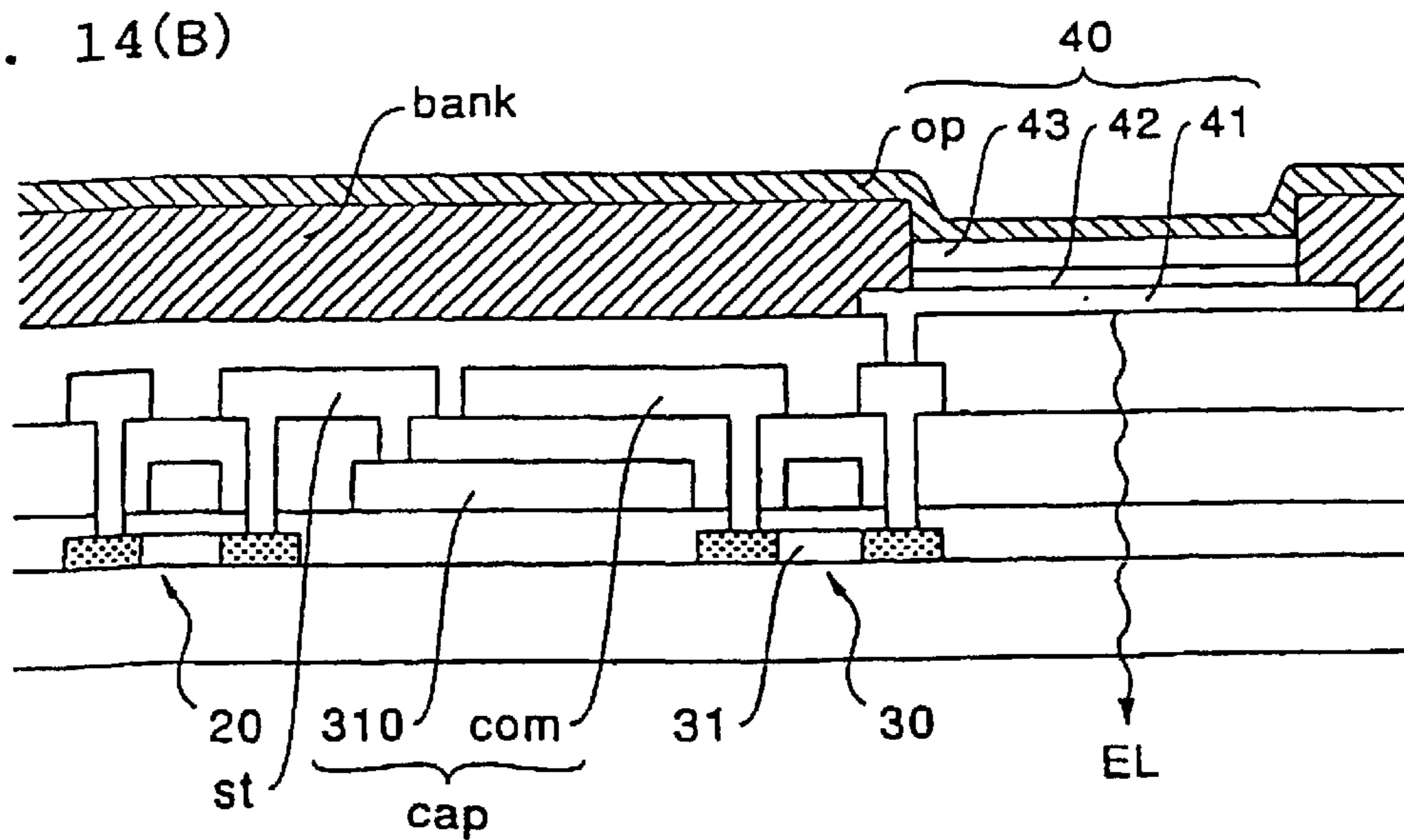
SECTION E-E'
