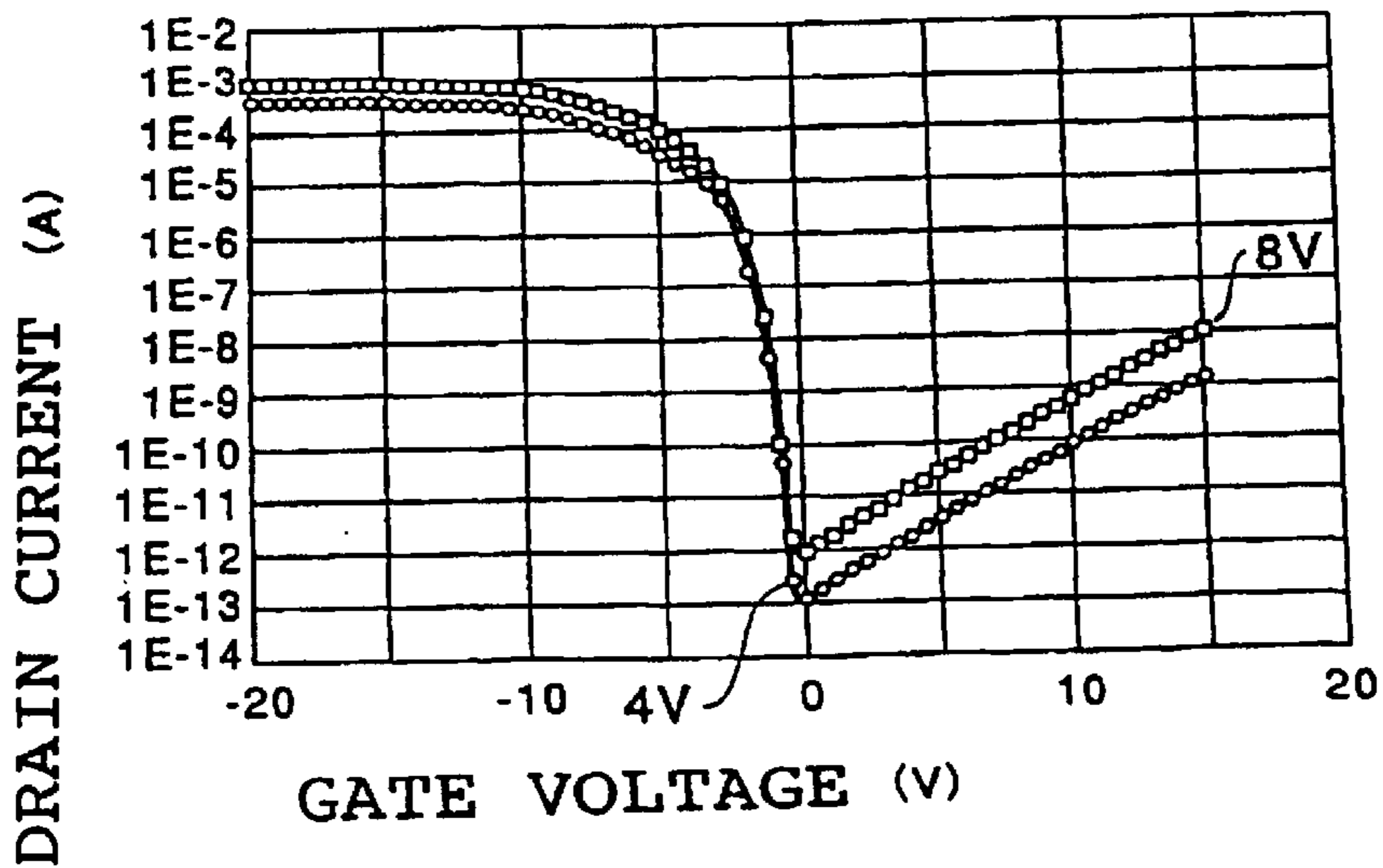
FIG. 12 AMPERE/VOLT CHARACTERISTICS P CHANNEL TYPE TFT
