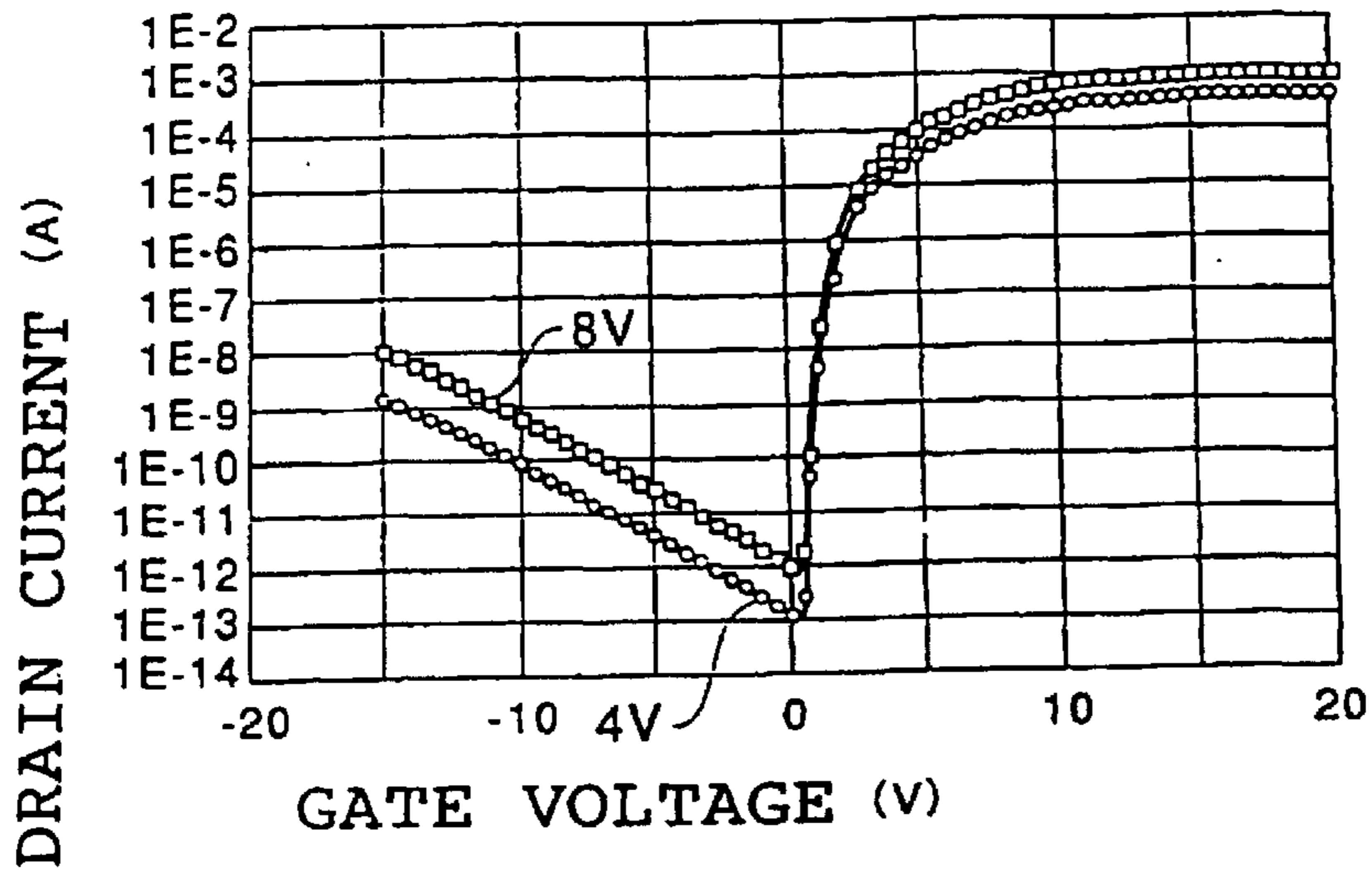
FIG. 11 AMPERE/VOLT CHARACTERISTICS N CHANNEL TYPE TFT
