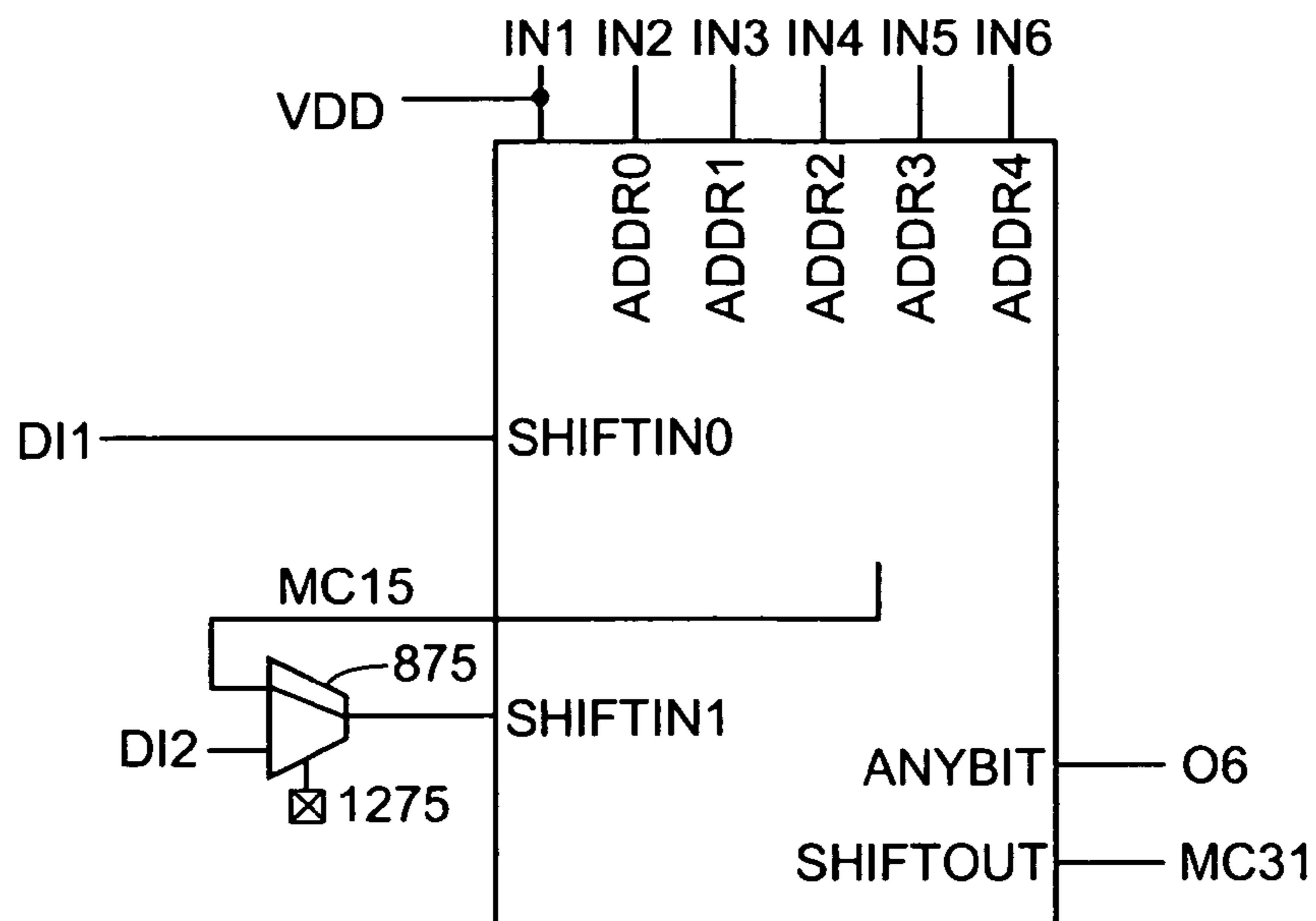
FIG. 12 (32x1 SRL)
