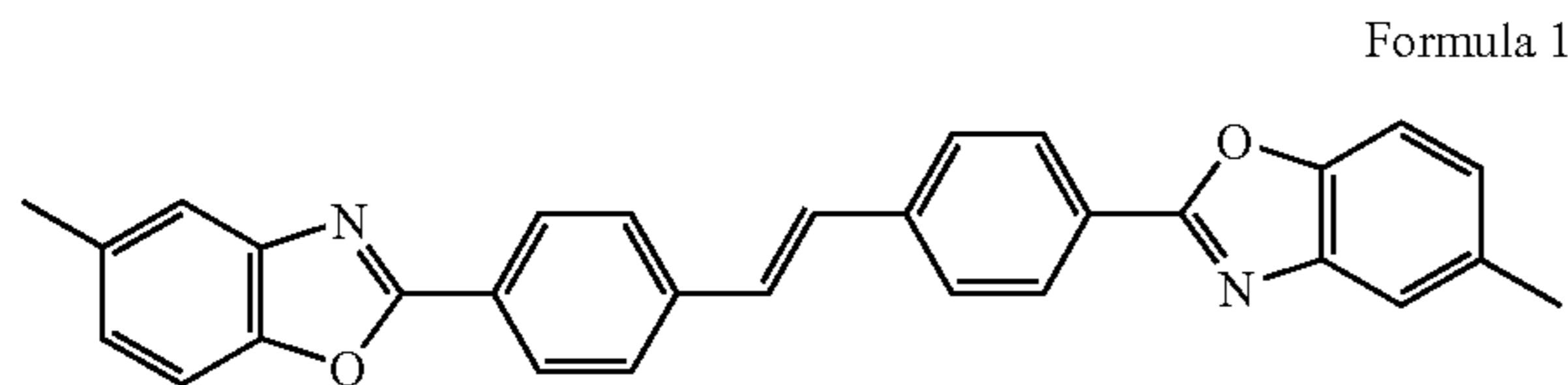
4,4'-Bis(5-methyl benzoxazol-2-yl)stilbene
