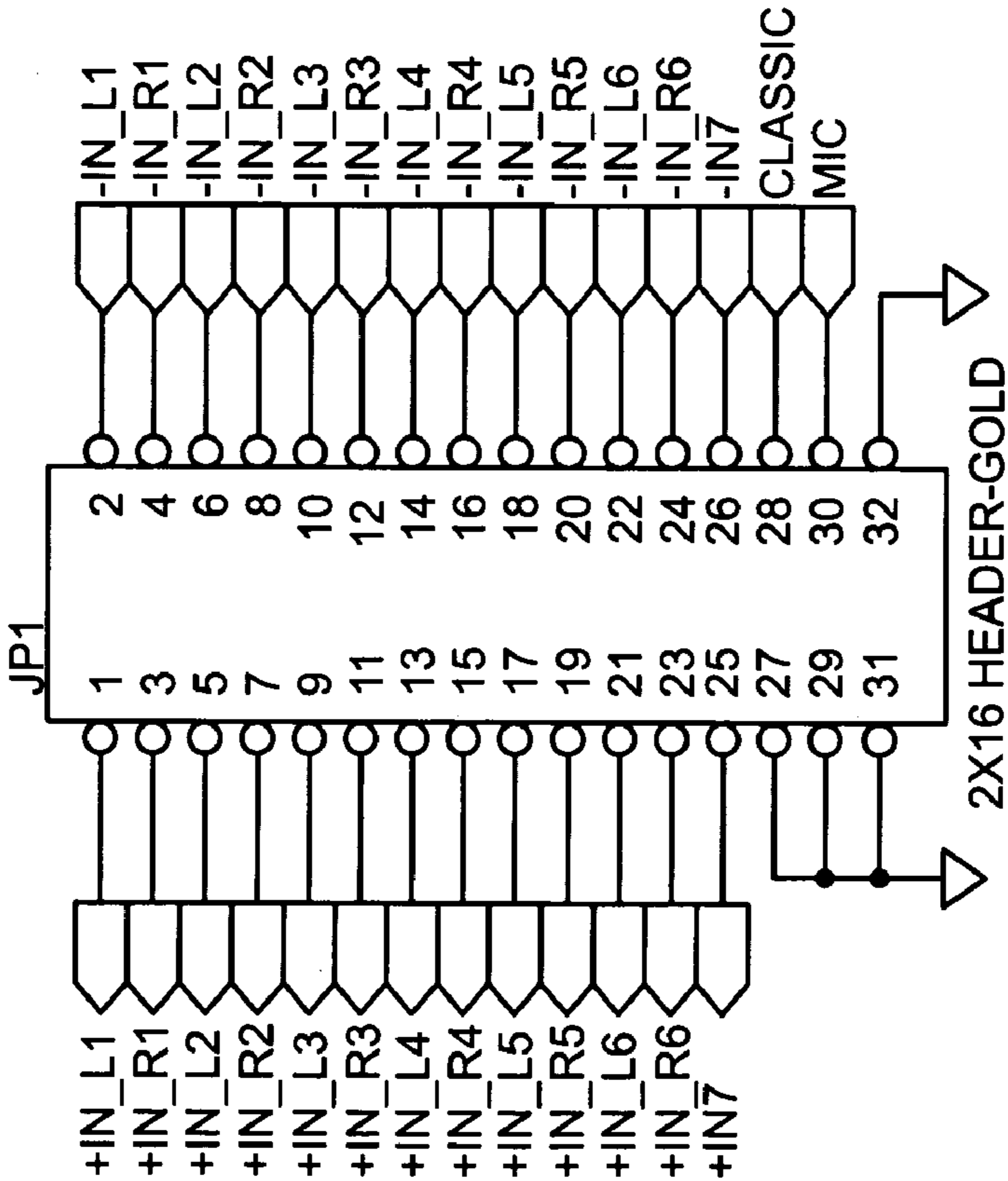
Pickup & Mic Inputs Connector to be specified
