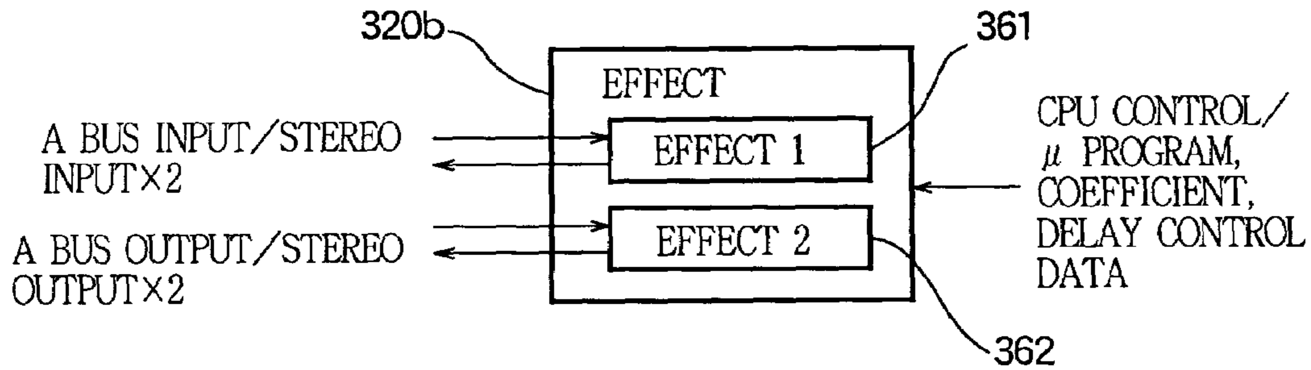
FIG.11 (c)
