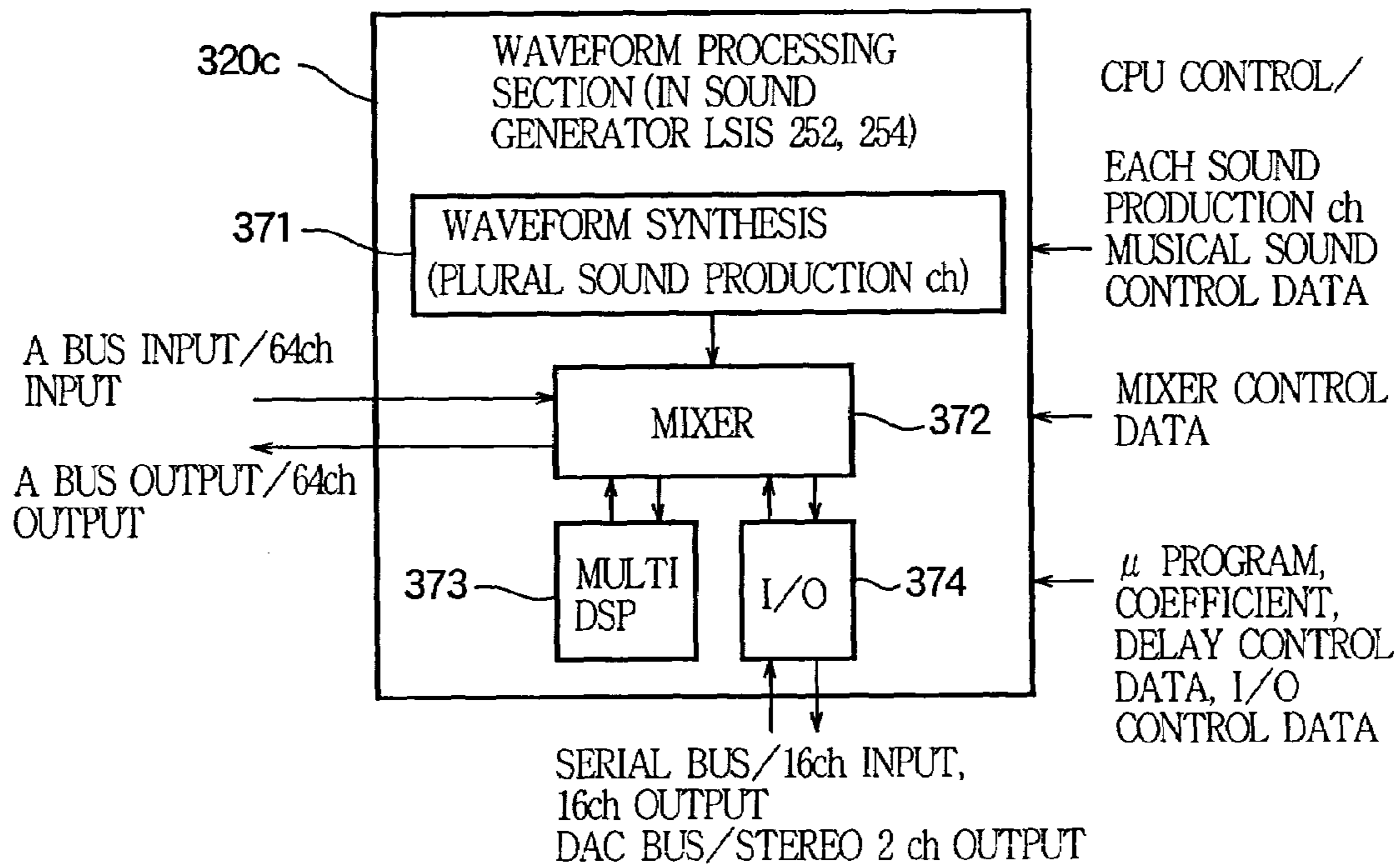
FIG.11 (c)
