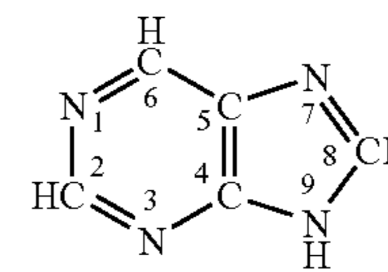
PURINE
