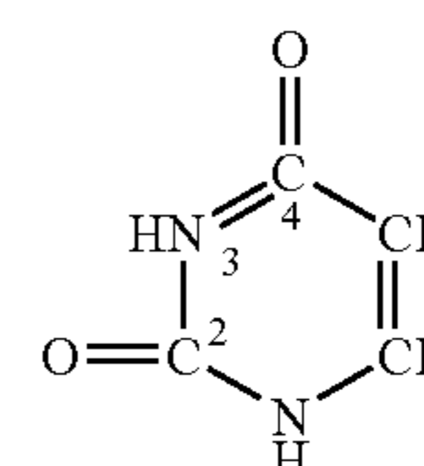
Uracil (2,4-dioxypyrimidine)
