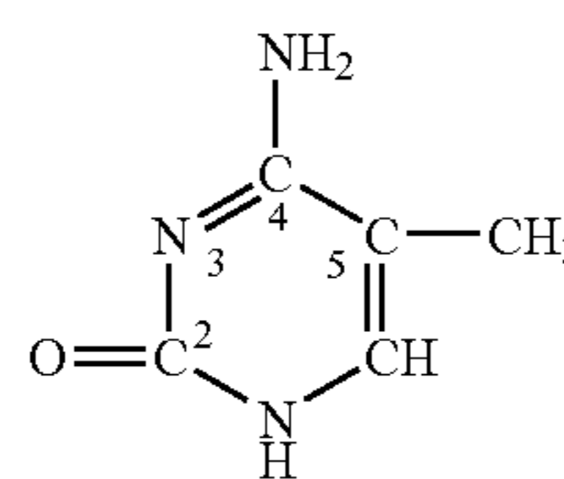
5-Methylcytosine
