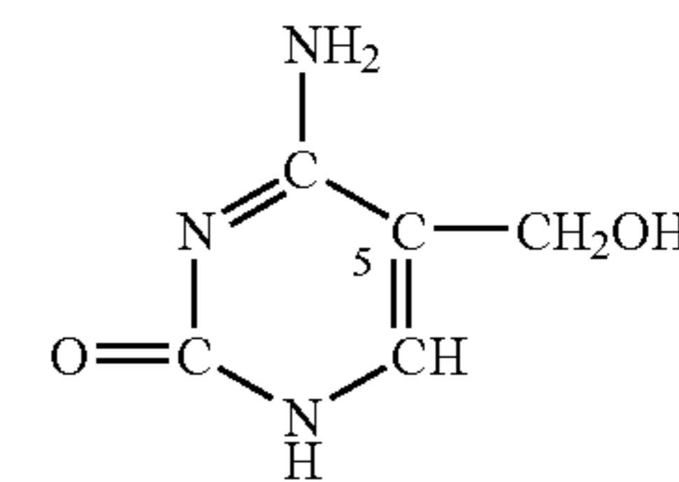
5-Hydroxymethylcytosine
