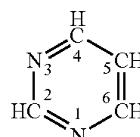
PYRIMIDINE
