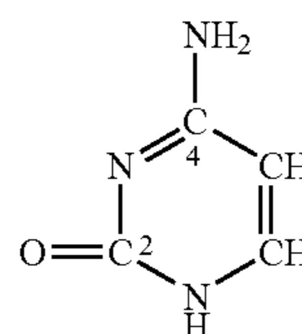
Cytosine (2-oxy-4-aminopyrimidine)
