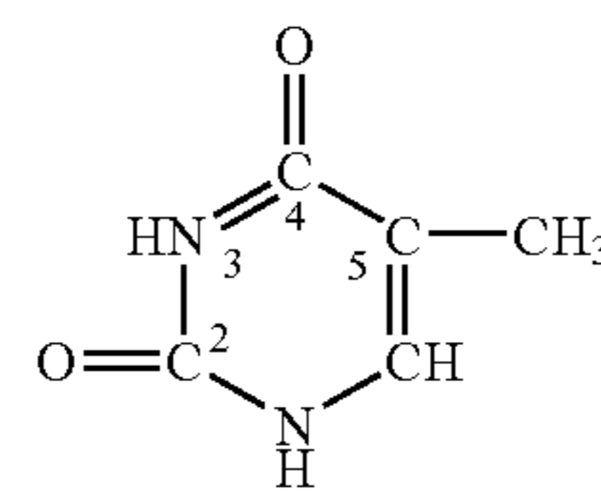
Thymine (5-methyl-2,4-dioxypyrimidine)
