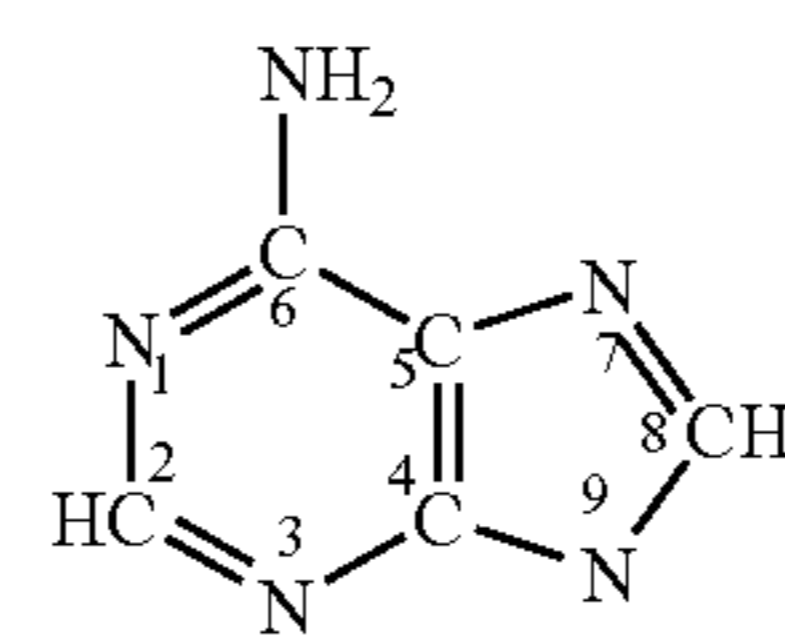
Adenosine (6-aminopurine)
