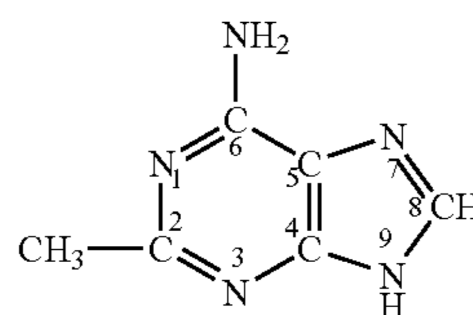
2-Methyladenine
