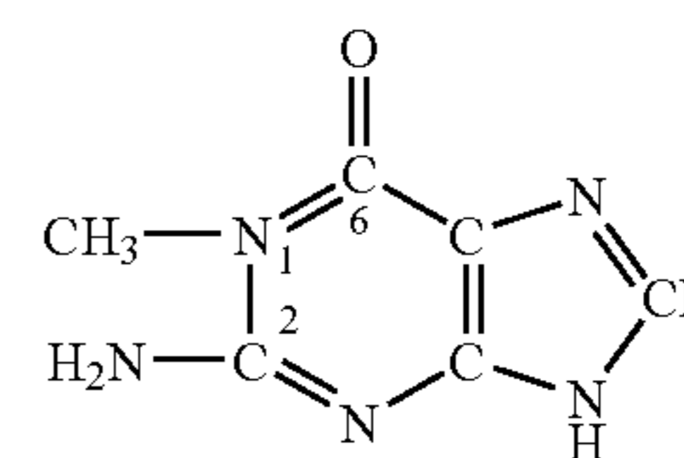
1-Methylguanine
