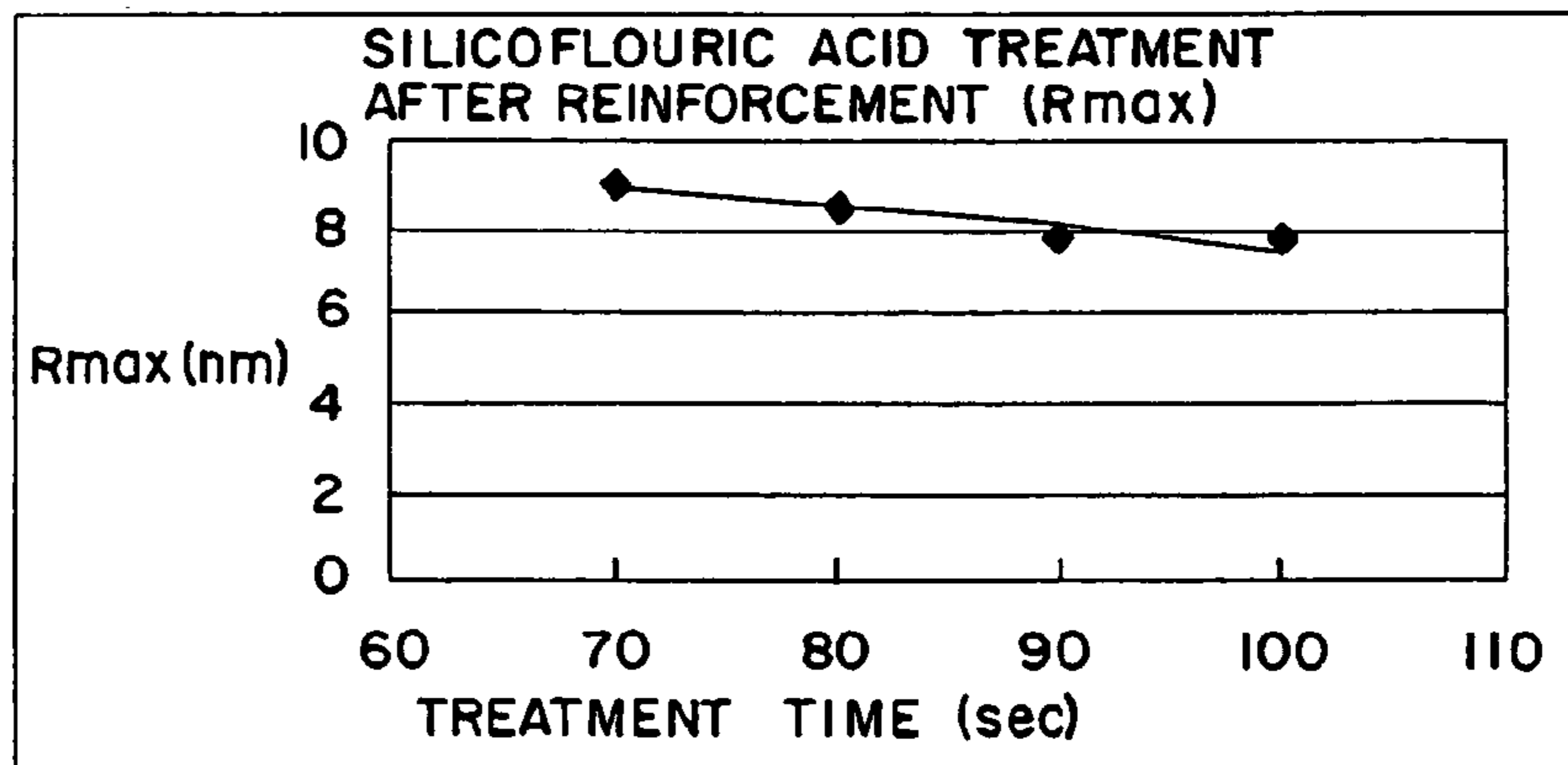
ROUGHNESS CHANGE BY H 2 SIF 6 TREATMENT AFTER CHEMICAL REINFORCEMENT (Rmax)
