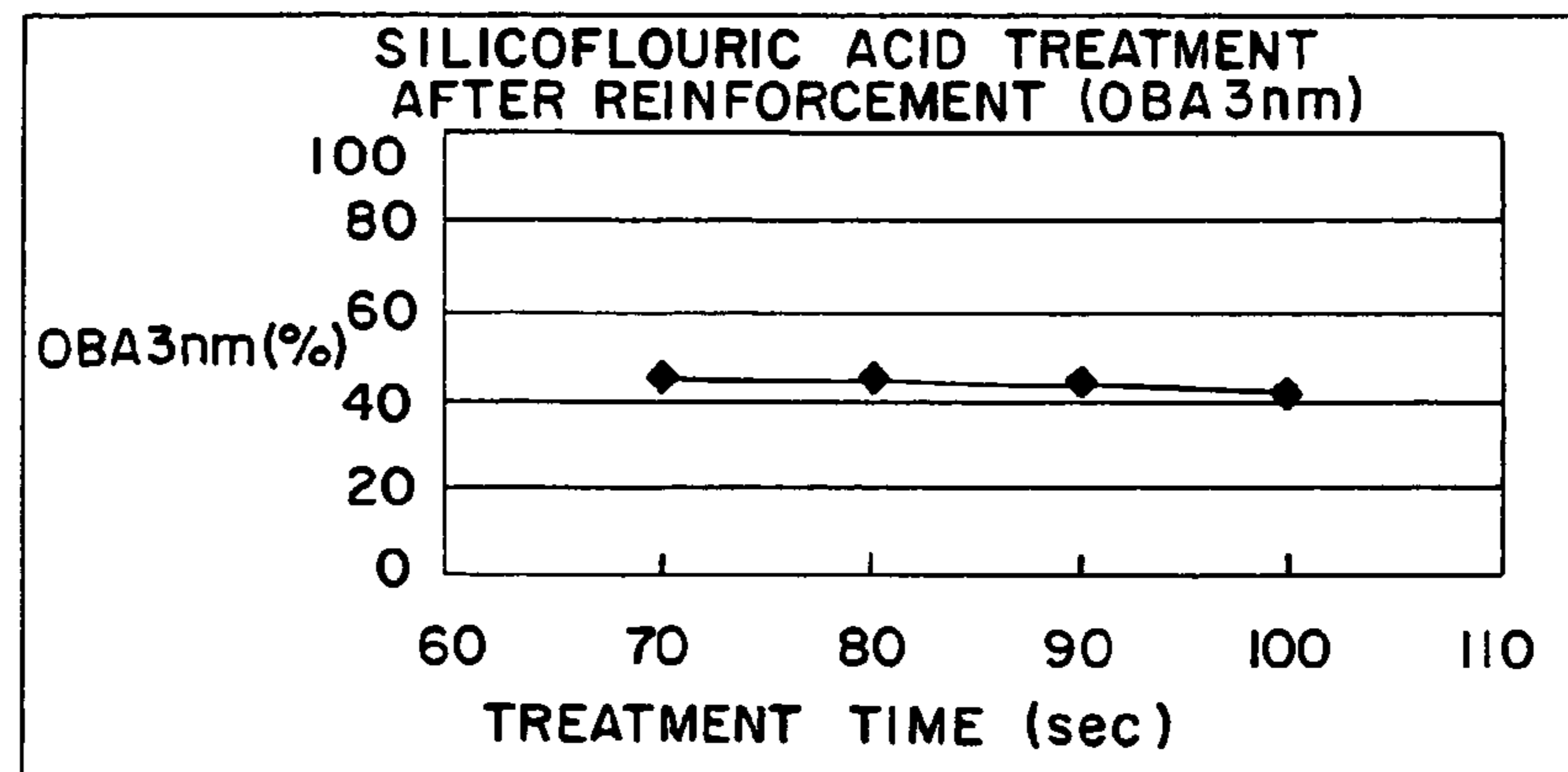
ROUGHNESS CHANGE BY H 2 SIF 6 TREATMENT AFTER CHEMICAL REINFORCEMENT (OBA3nm)
