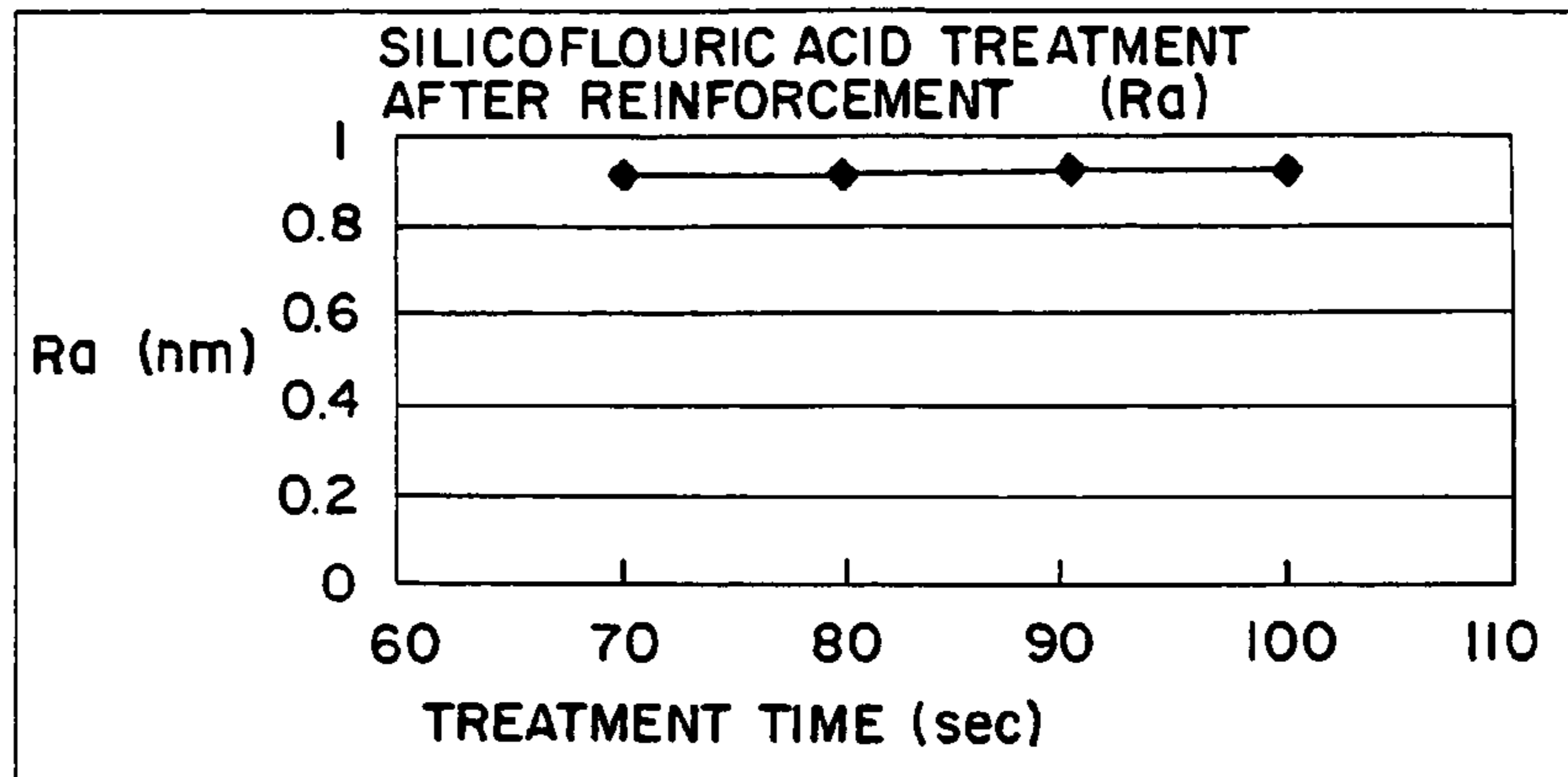
ROUGHNESS CHANGE BY H 2 SIF 6 TREATMENT AFTER CHEMICAL REINFORCEMENT (Ra)
