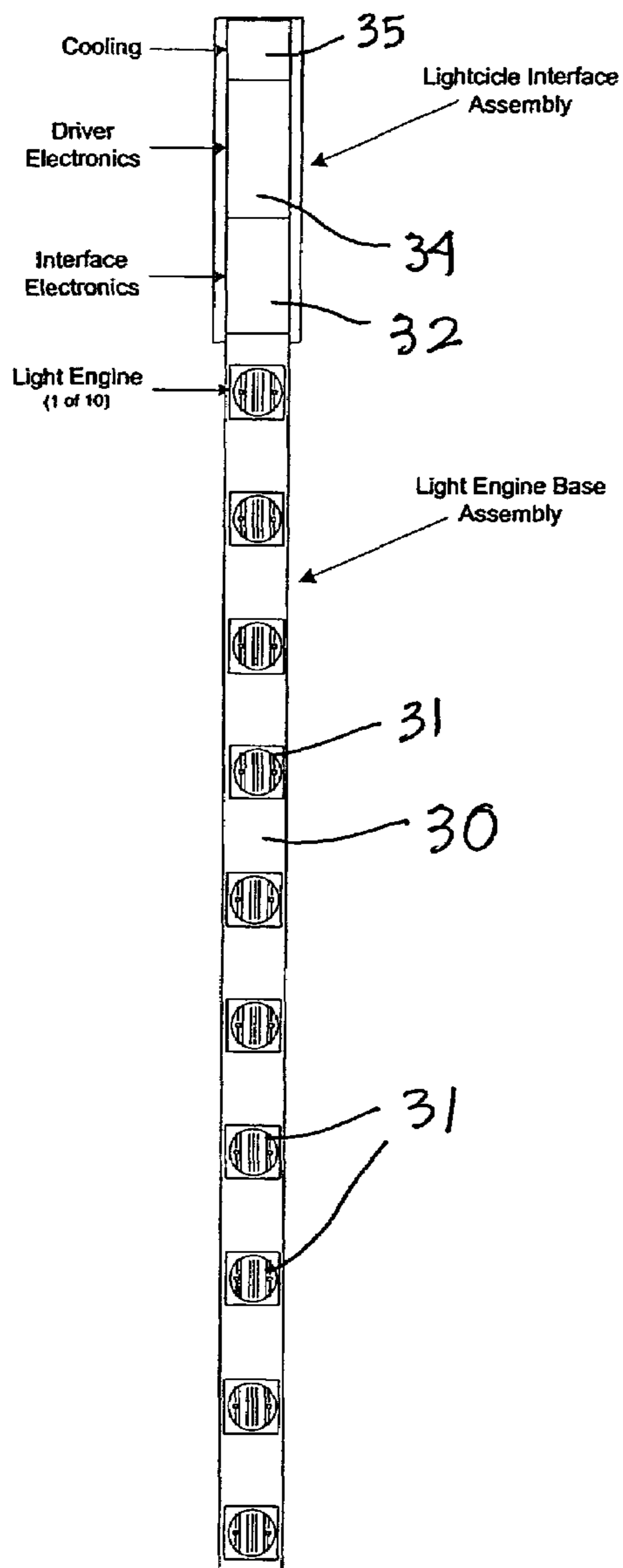
Figure 6 Lightcicle Basic Structure
