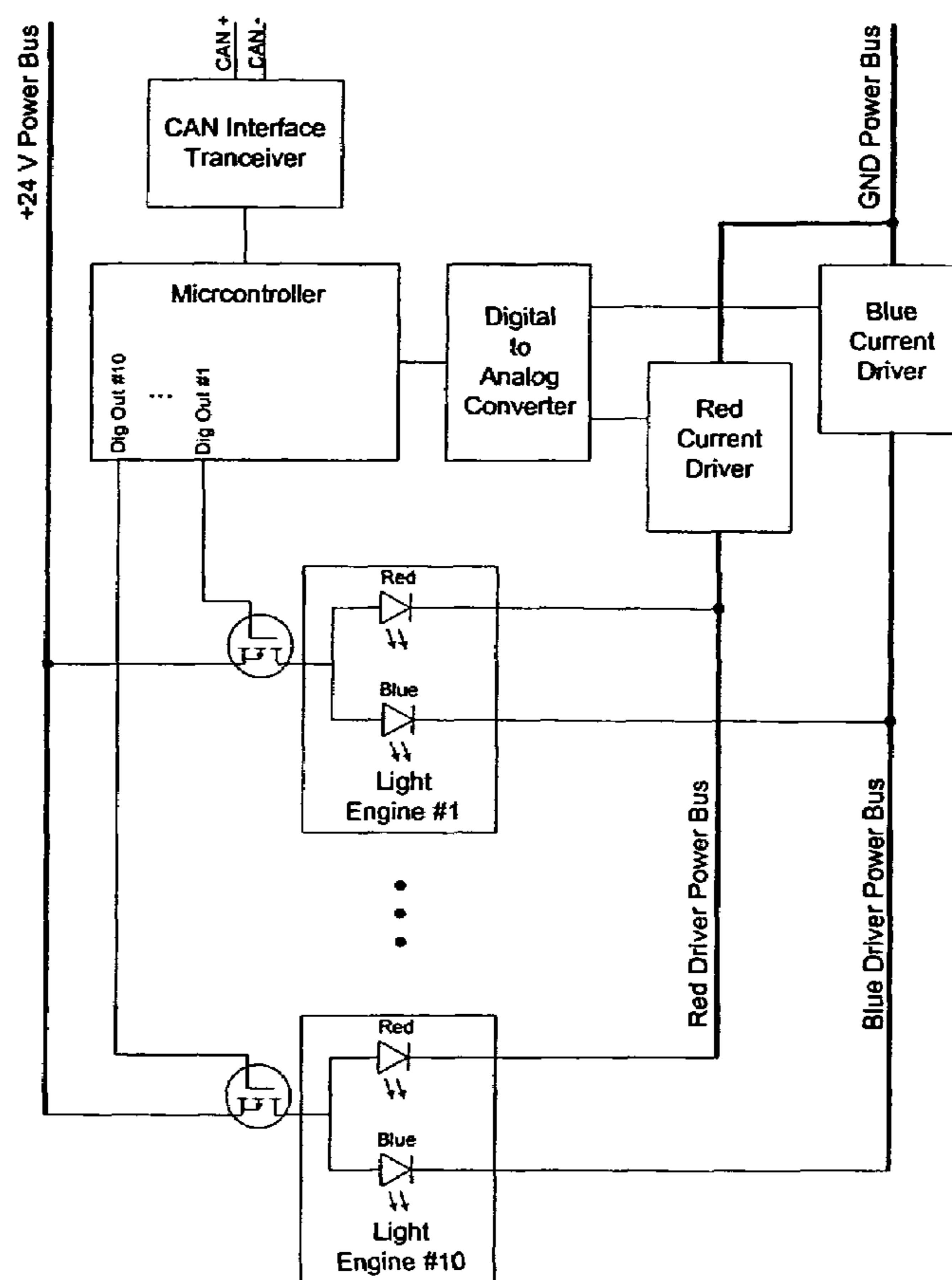
Figure 7 Interface and Driver Electronics Block Diagram
