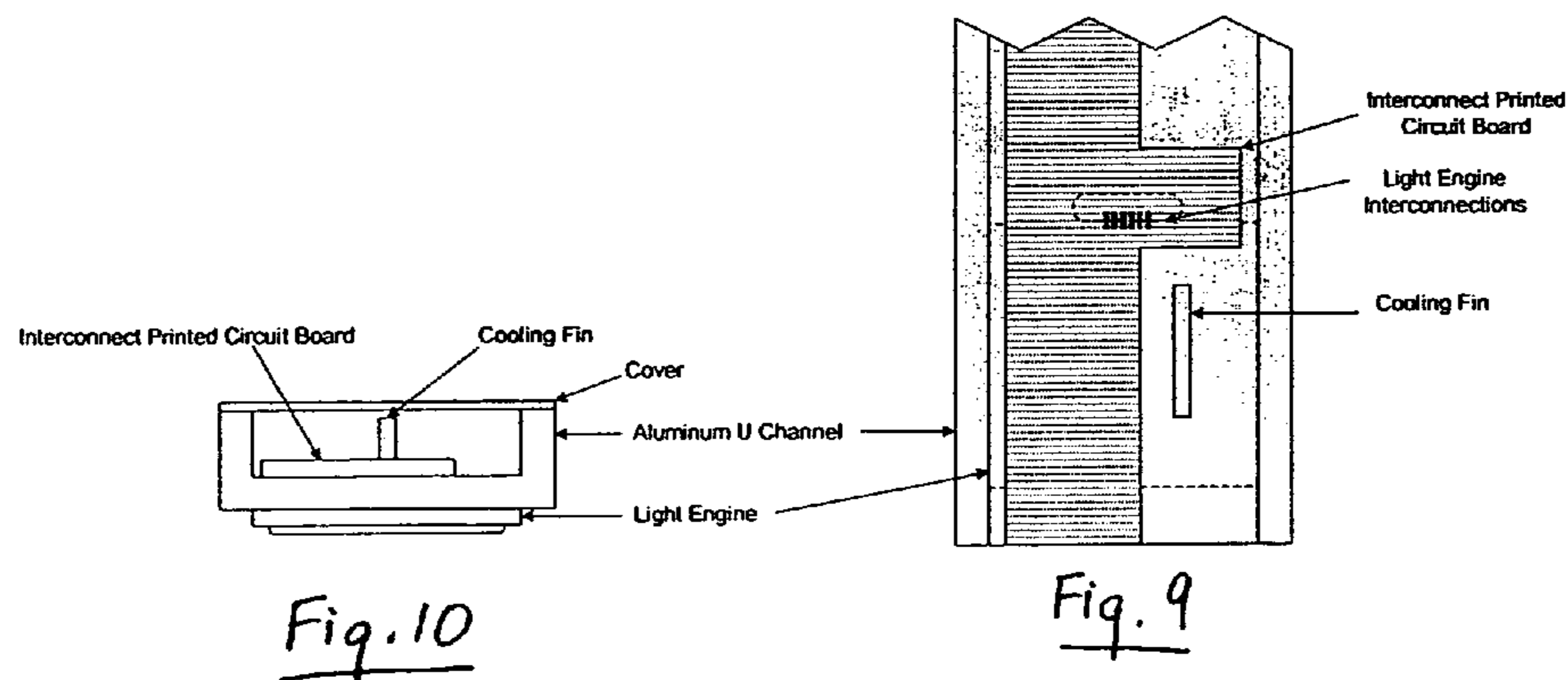
Fig. 10 Fig. 9 Light Engine Base Assembly Details
