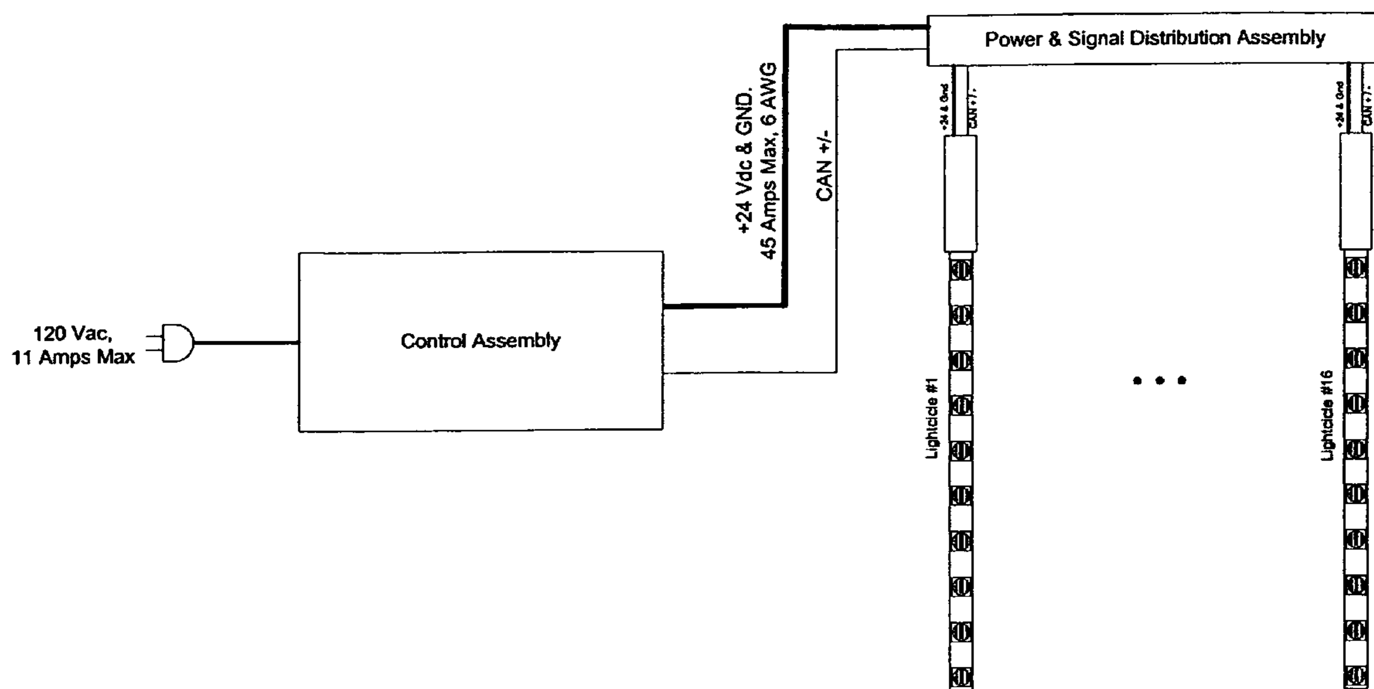
Figure 8 Quadrant System Components and Interconnects
