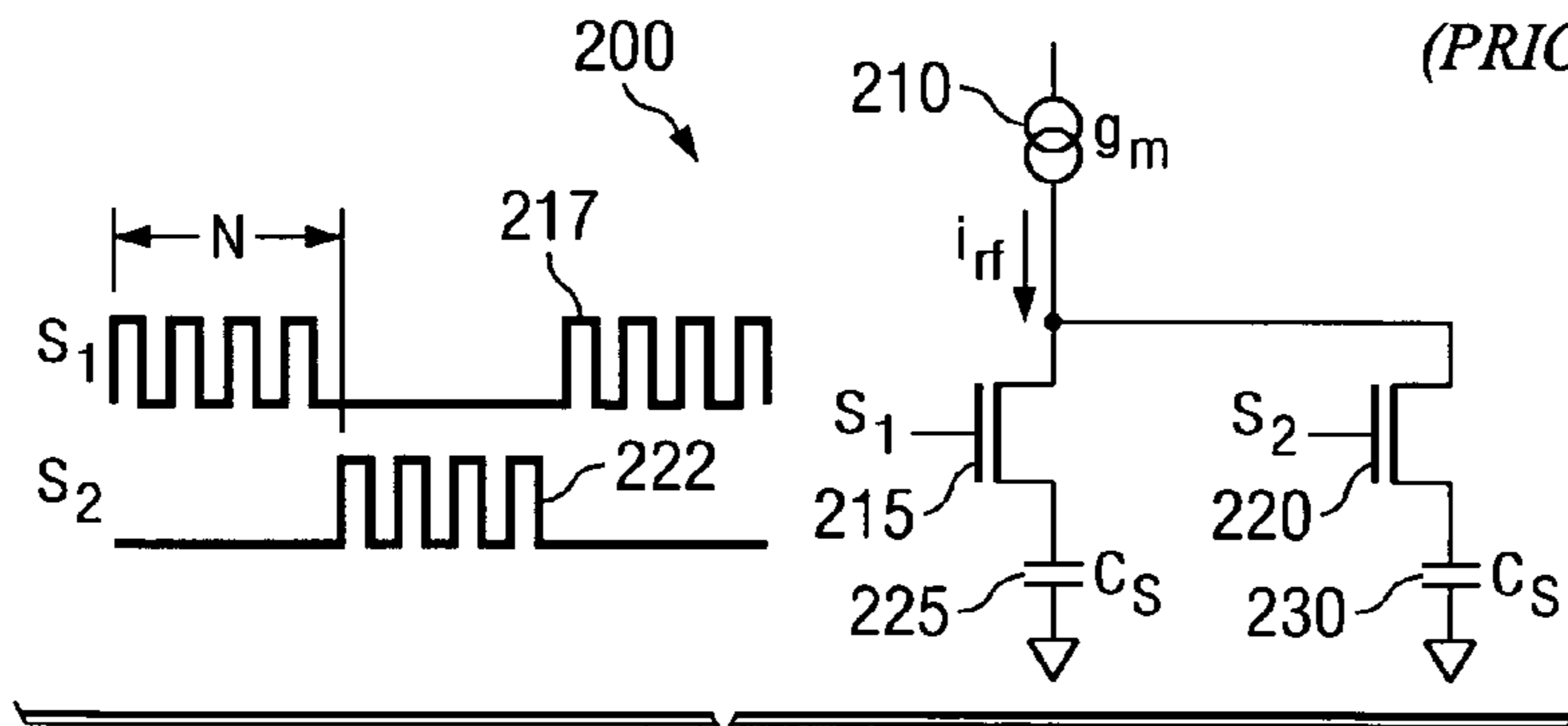
FIG. 2 (PRIOR ART)
