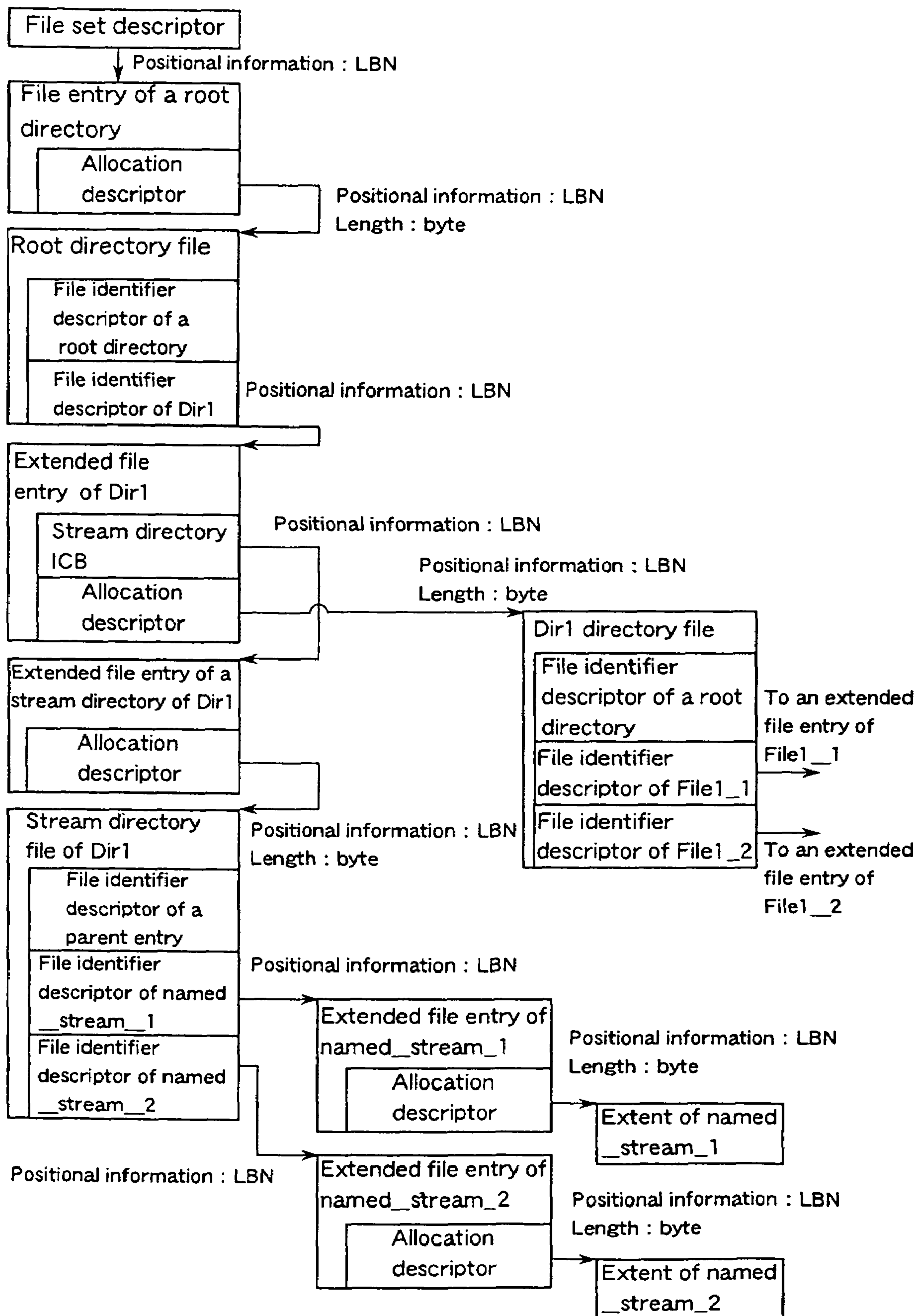
FIG. 46 (PRIOR ART)
