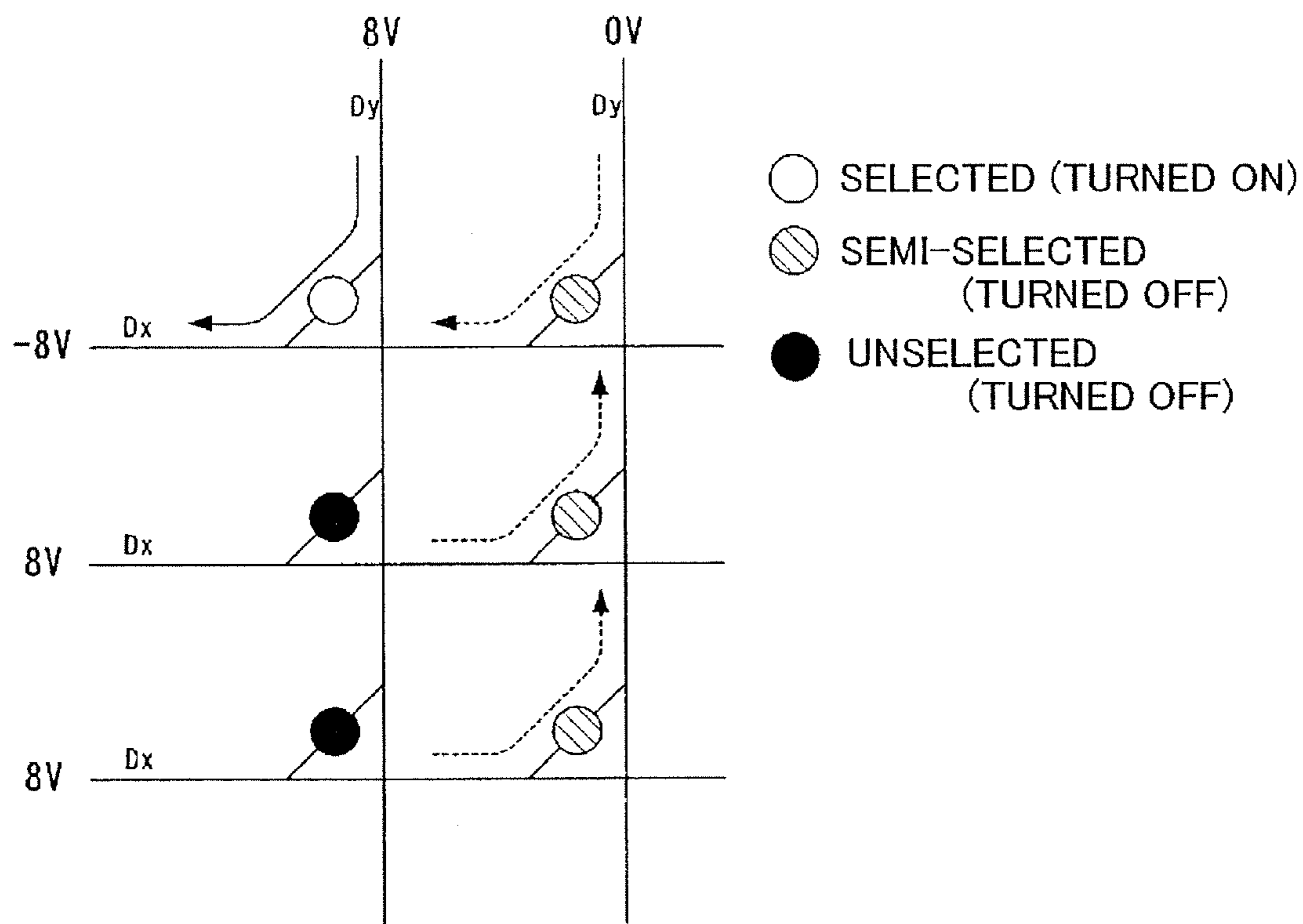
Fig.17 (PRIOR ART)
