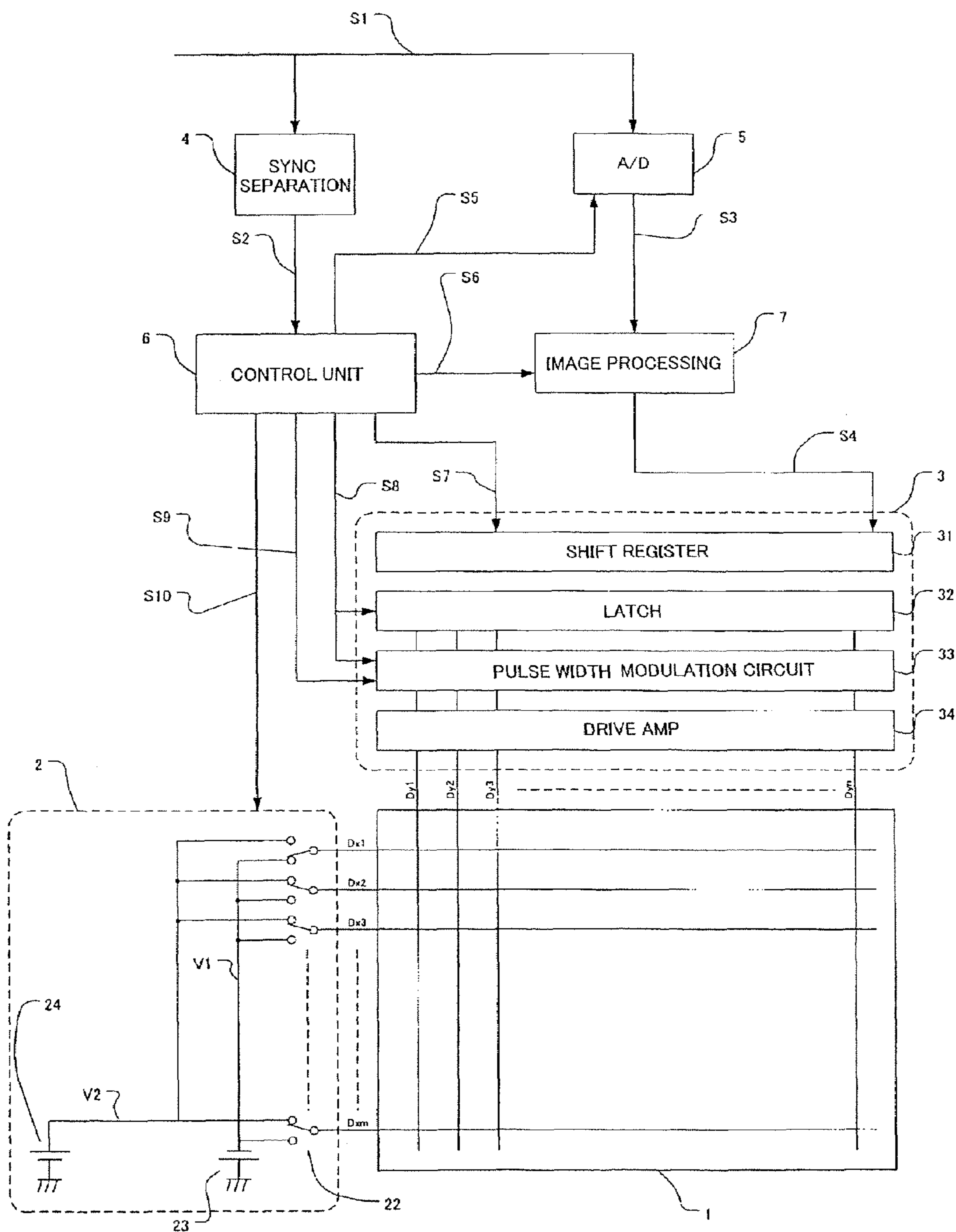
Fig.15 (PRIOR ART)
