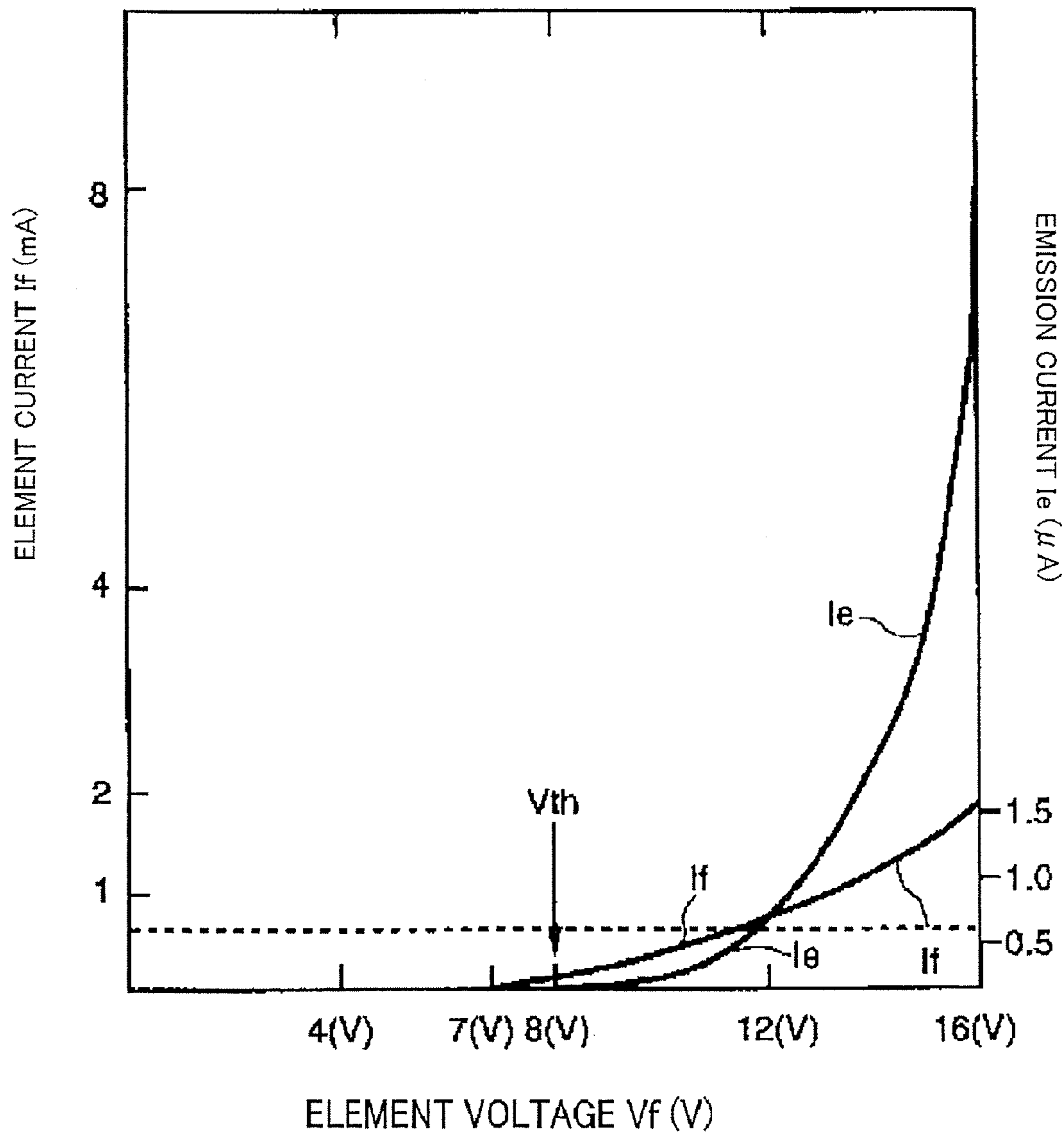
Fig.16 (PRIOR ART)
