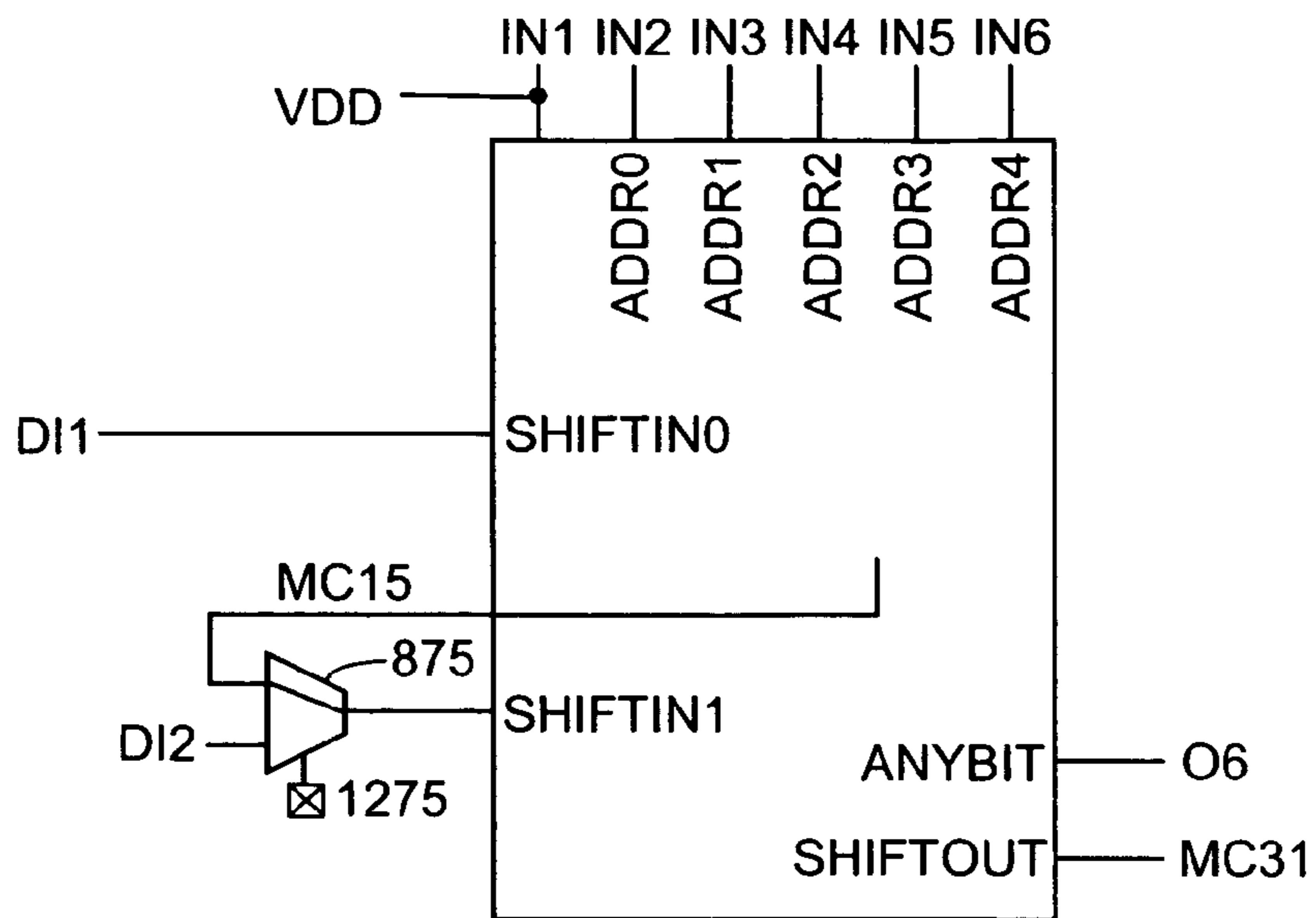
FIG. 12 (32x1 SRL)
