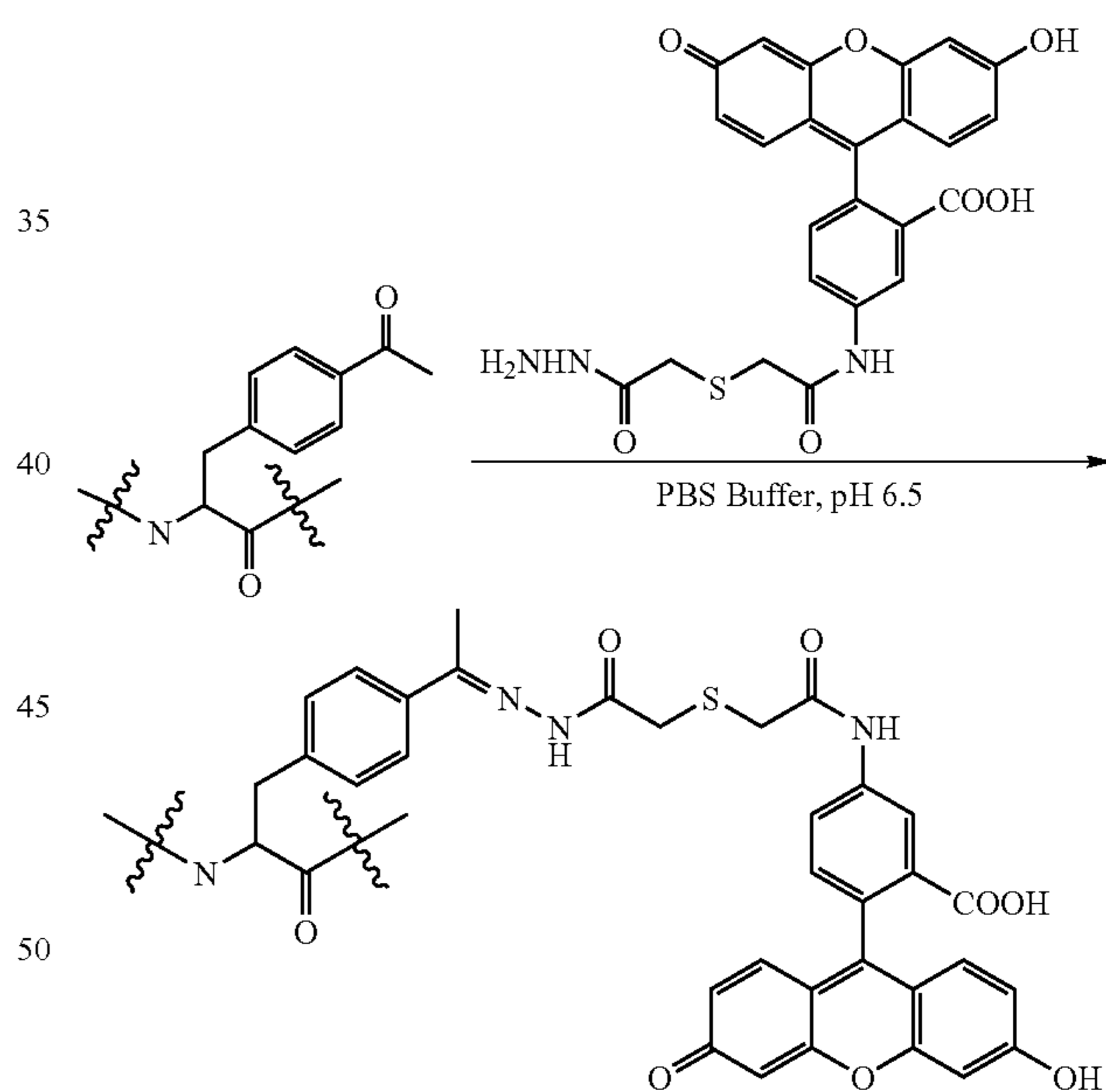
Scheme 1
