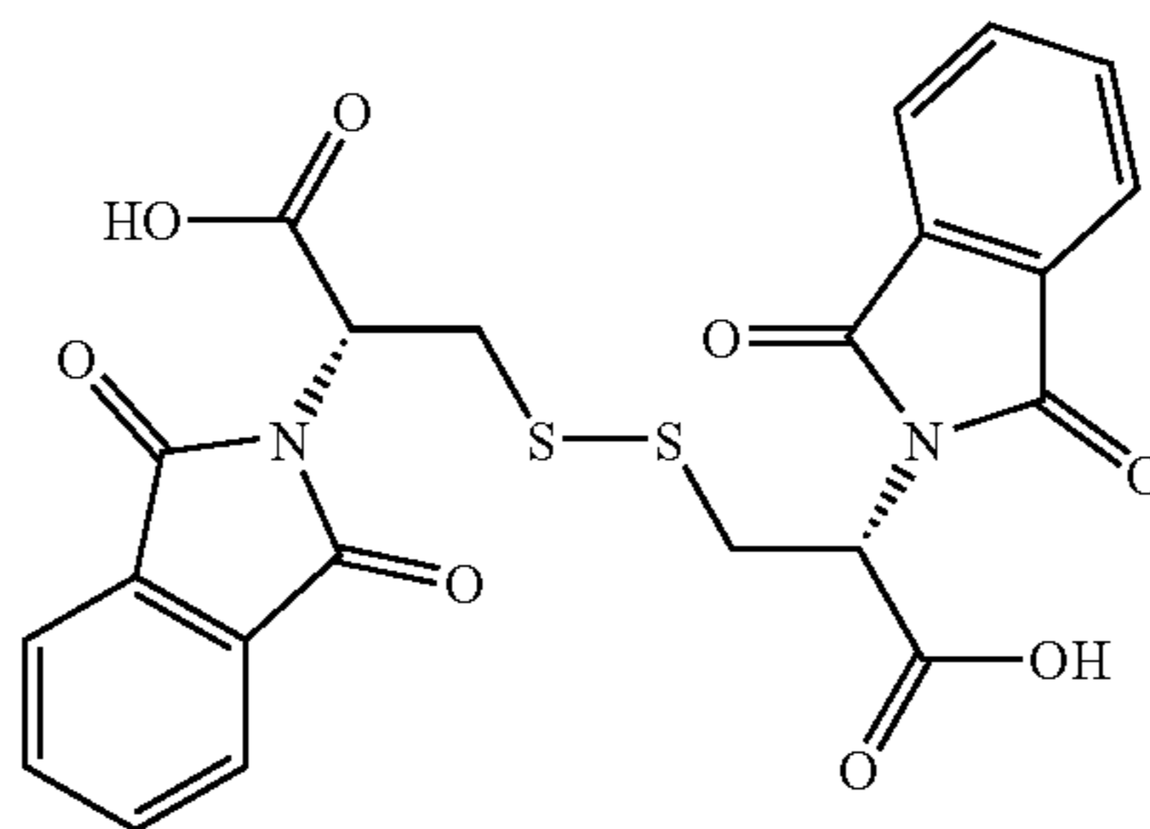
Chiral X-123
