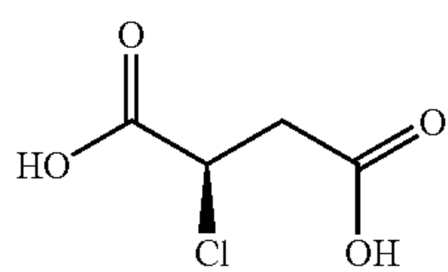
Chiral X-34
