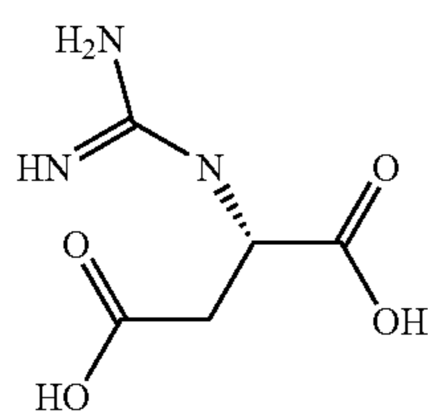
Chiral X-53
