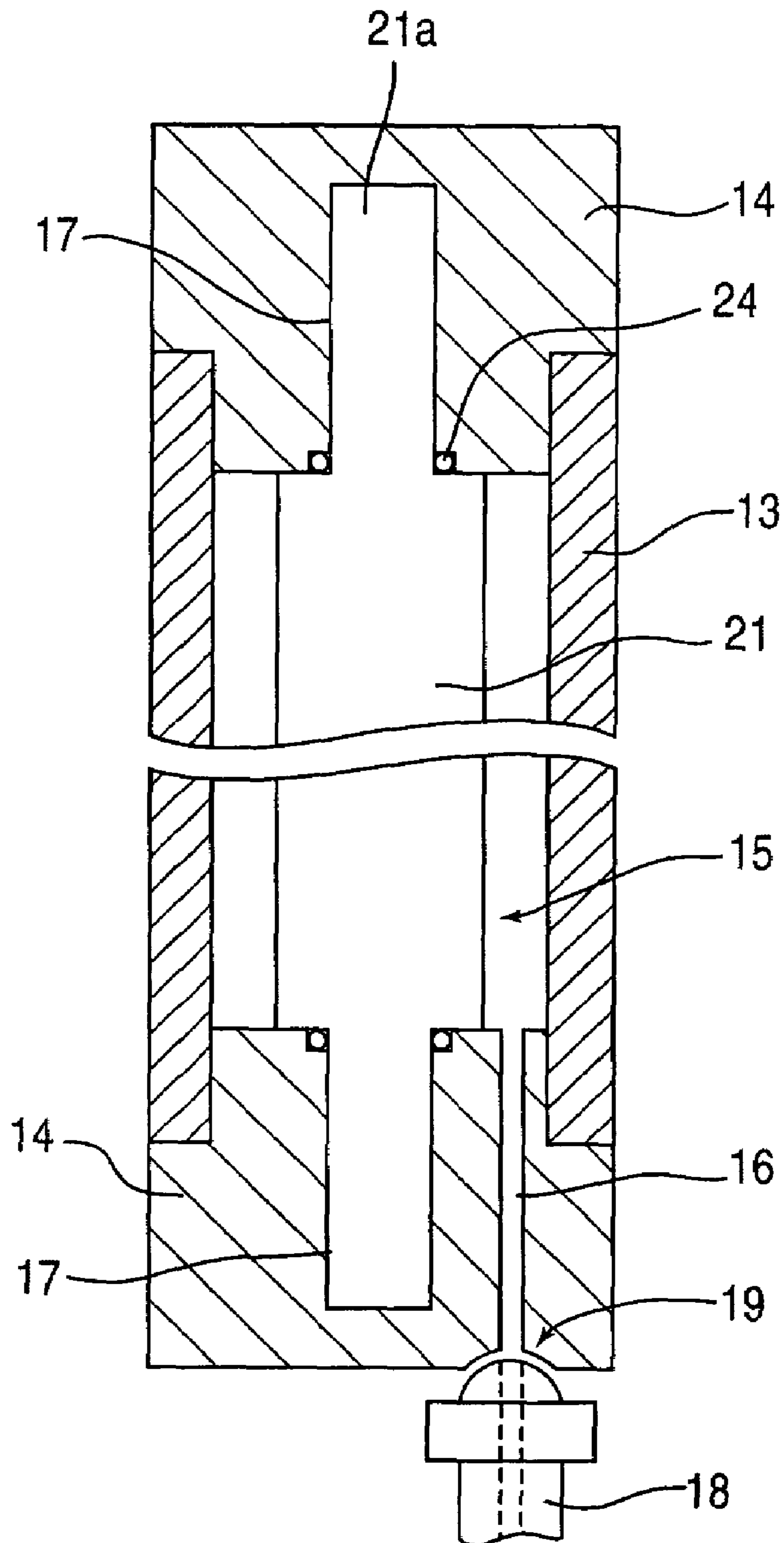
FIG. 25 PRIOR ART
