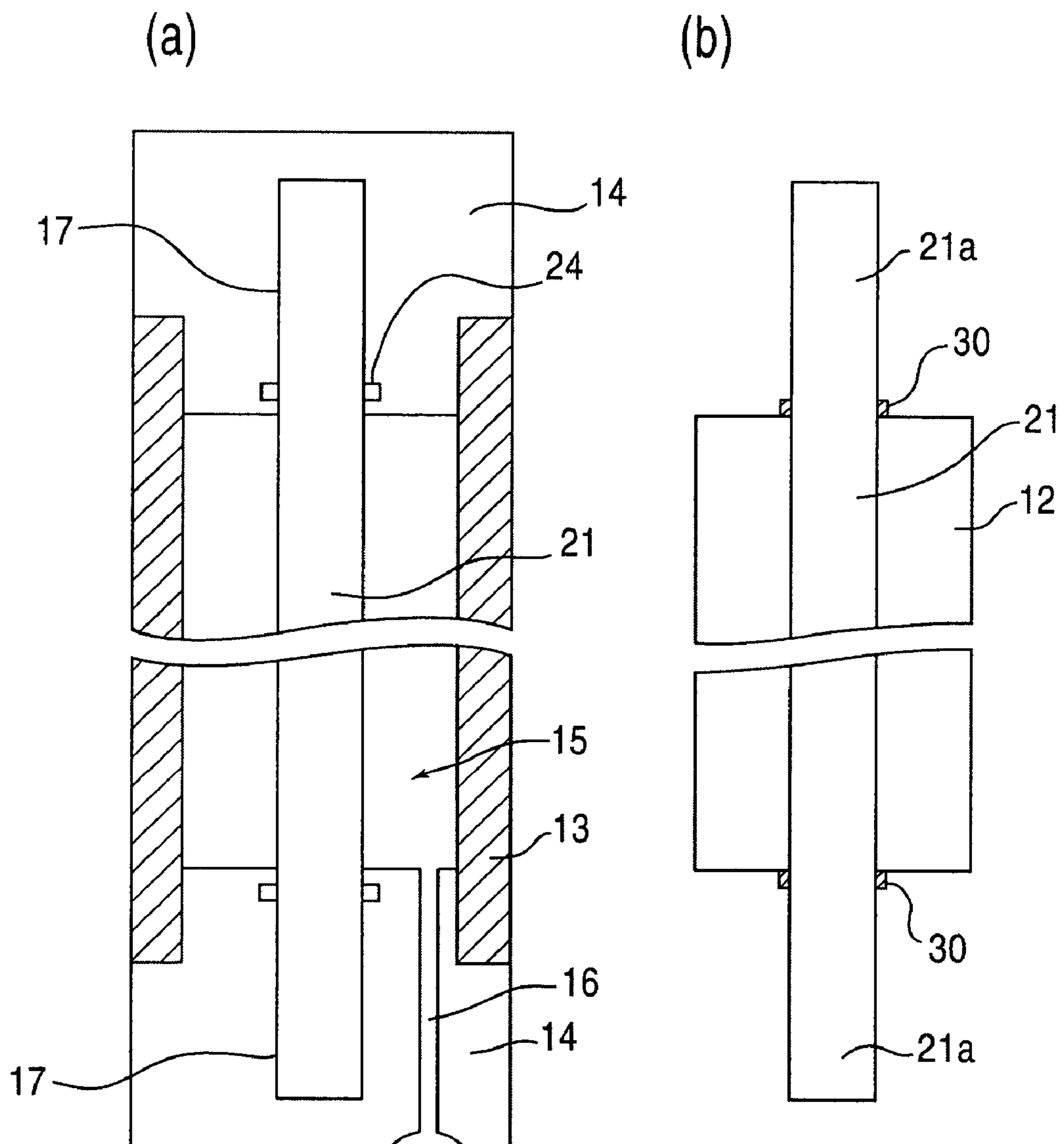
FIG. 26 PRIOR ART
