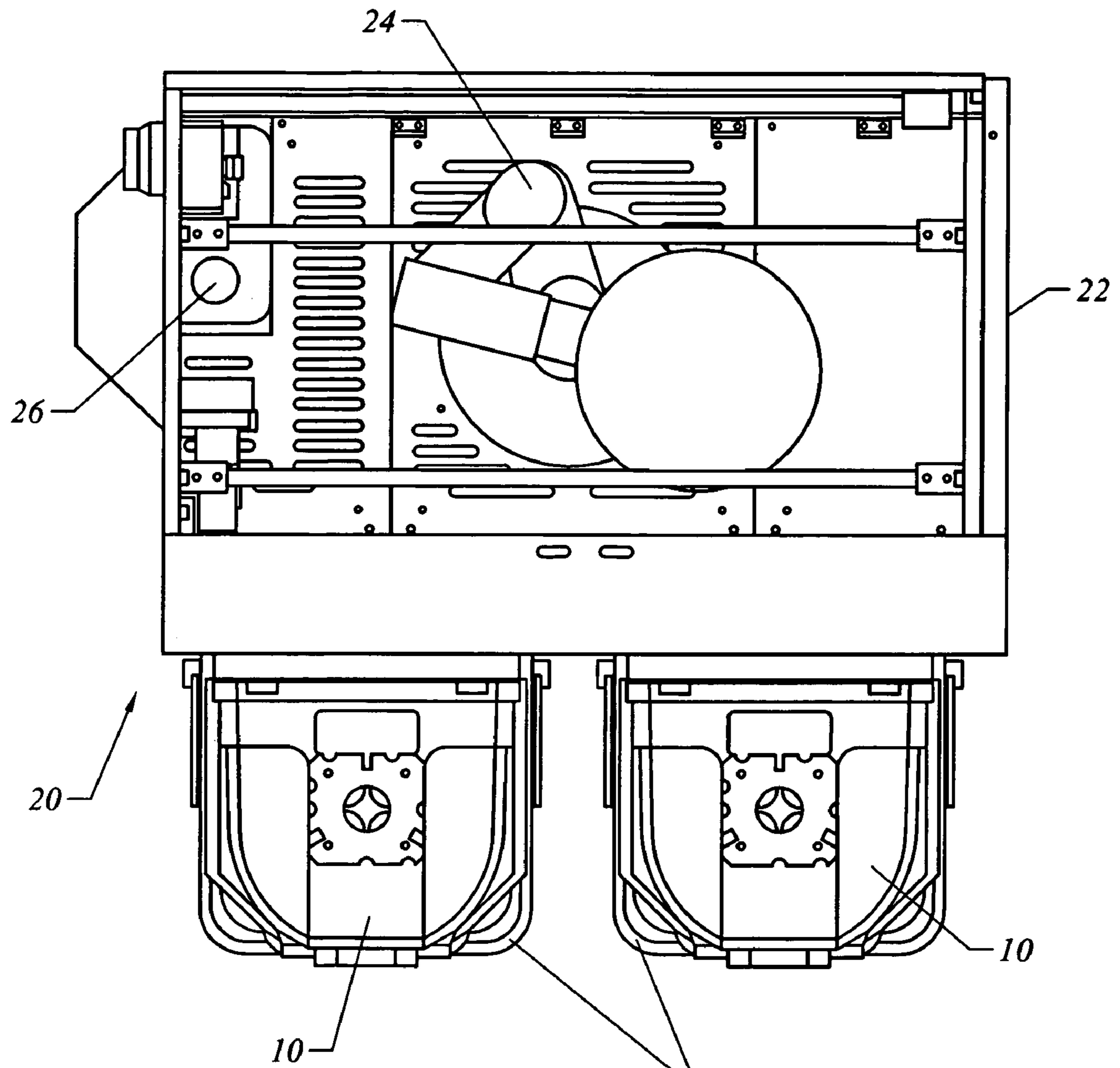
FIG. 2 (Prior Art)
