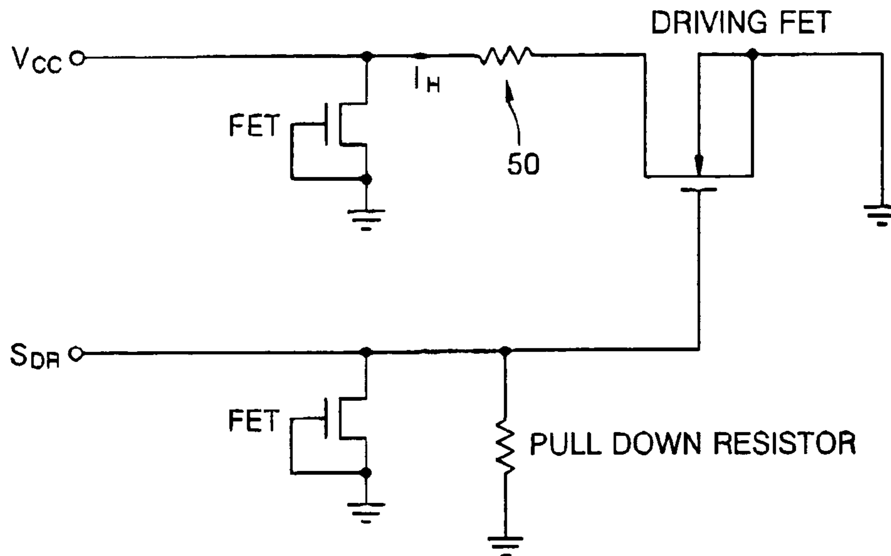
FIG. 6 (PRIOR ART)
