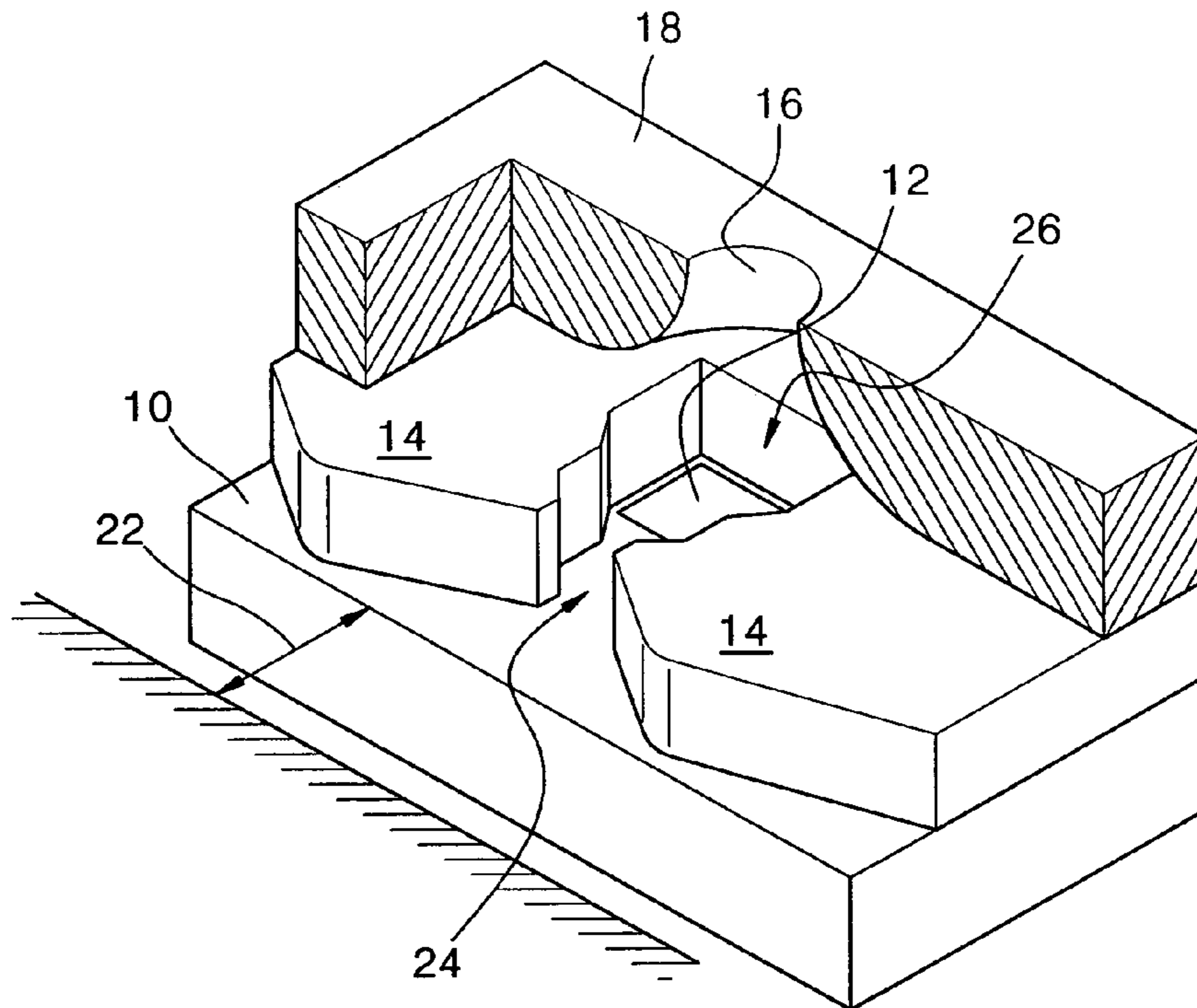
FIG. 2 (PRIOR ART)
